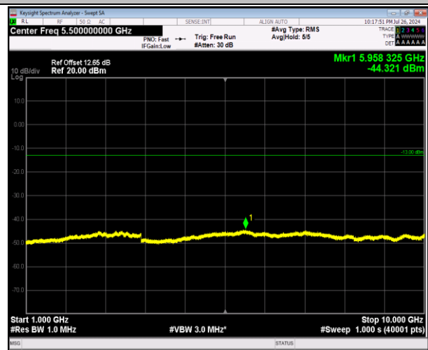
5-5-3MHz-5MHz-64QAM-64QAM-20416-20455-1RB#0-0RB#0-1000~10000MHz-PASS
