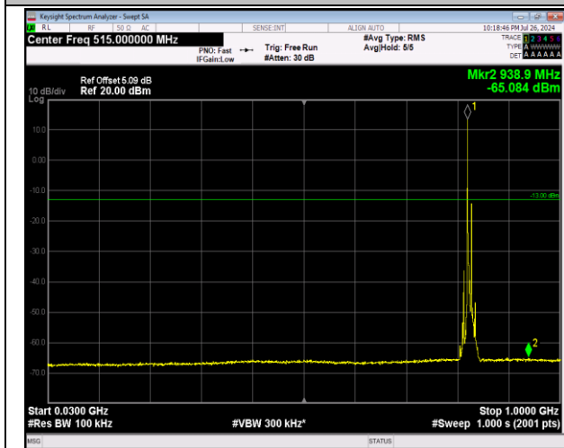
5-5-3MHz-5MHz-64QAM-64QAM-20416-20455-1RB#0-0-1RB#24-30~1000MHz-PASS
