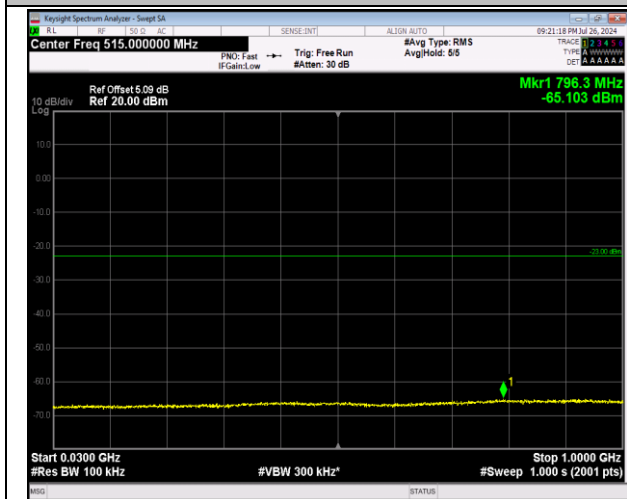
2-2-20MHz-20MHz-64QAM-64QAM-18902-19100-1RB#0-1RB#99-30~1000MHz-PASS
