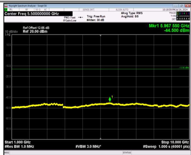
5-5-3MHz-5MHz-64QAM-64QAM-20416-20455-1RB#0-0-1RB#24-1000~10000MHz-PASS
