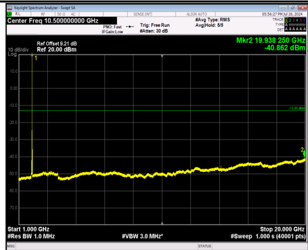
2-2-5MHz-20MHz-64QAM-64QAM-18983-19100-1RB#24-0 RB#0-1000~20000MHz-PASS
