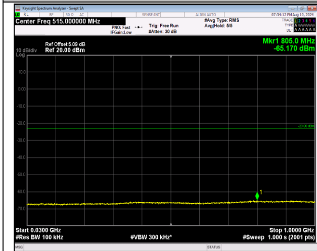
2-2-20MHz-20MHz-16QAM-16QAM-18902-19100-1RB#9 9-0RB#0-30~1000MHz-PASS
