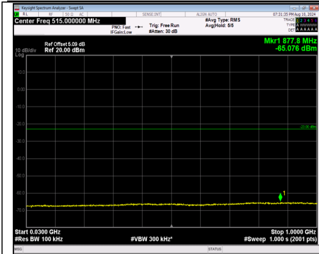
2-2-20MHz-20MHz-16QAM-16QAM-18801-18999-100RB #0-100RB#0-30~1000MHz-PASS
