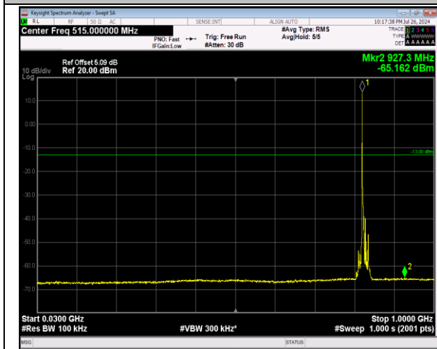
5-5-3MHz-5MHz-64QAM-64QAM-20416-20455-1RB#0-0-RB#0-30~1000MHz-PASS
