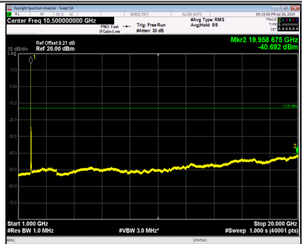
2-2-20MHz-20MHz-64QAM-64QAM-18801-18999-1RB#0-1 RB#99-1000~20000MHz-PASS
