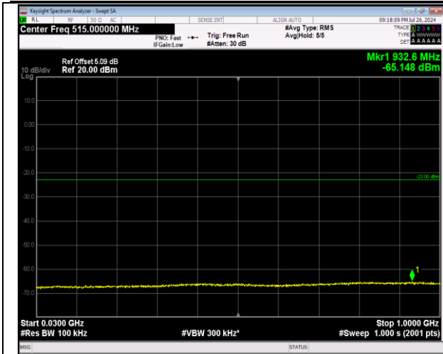
2-2-20MHz-20MHz-64QAM-64QAM-18801-18999-1RB#9 9-ORB#0-30~1000MHz-PASS
