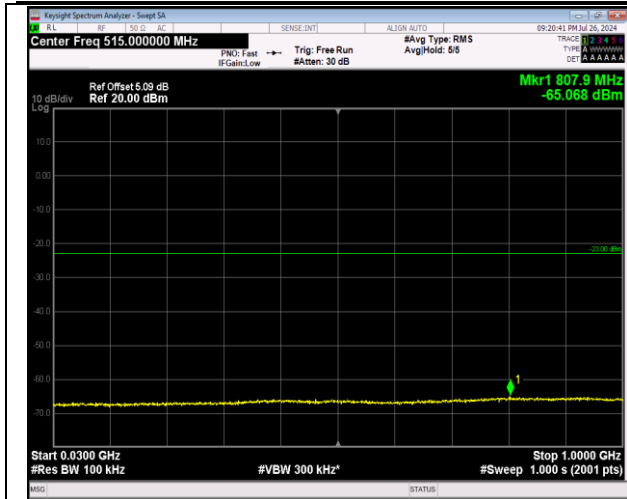
2-2-20MHz-20MHz-64QAM-64QAM-18902-19100-1RB#9 9-0RB#0-30~1000MHz-PASS
