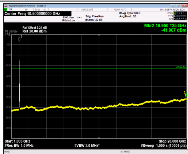
2-2-20MHz-20MHz-64QAM-64QAM-18700-18898-1RB#0-1 RB#99-1000~20000MHz-PASS
