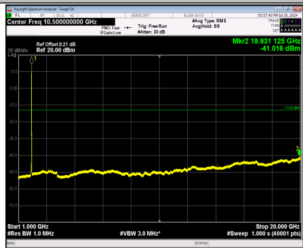
2-2-5MHz-20MHz-64QAM-64QAM-18983-19100-25RB#0-1 00RB#0-1000~20000MHz-PASS
