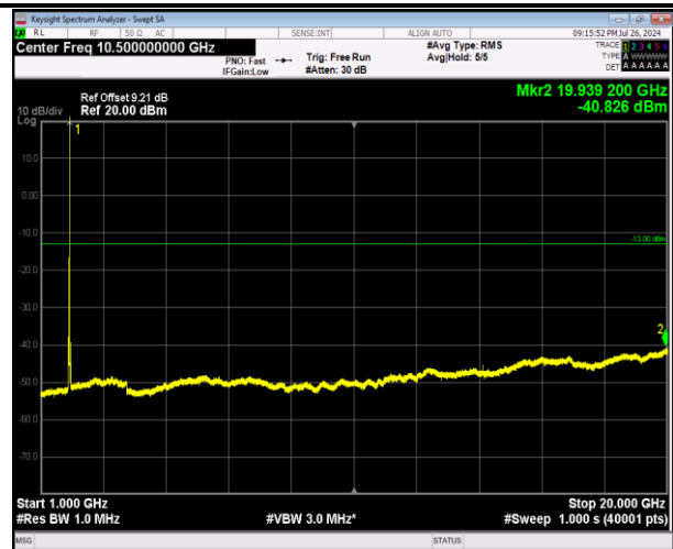
2-2-20MHz-20MHz-64QAM-64QAM-18700-18898-1RB#99- ORB#0-1000~20000MHz-PASS
