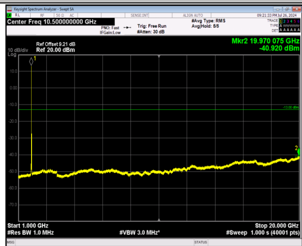
2-2-20MHz-20MHz-64QAM-64QAM-18902-19100-1RB#0-1RB#99-1000~20000MHz-PASS
