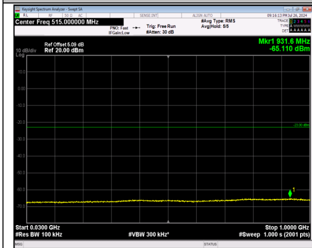
2-2-20MHz-20MHz-64QAM-64QAM-18700-18898-1RB#0 -1RB#99-30~1000MHz-PASS
