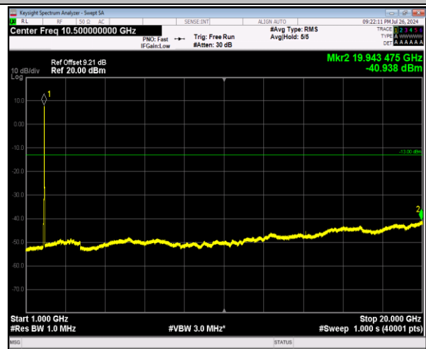
2-2-20MHz-20MHz-64QAM-64QAM-18902-19100-100RB#0 -100RB#0-1000~20000MHz-PASS
