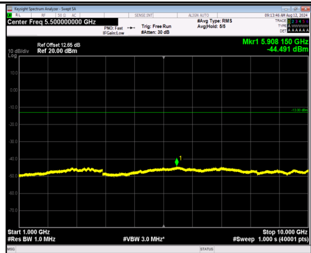
5-5-3MHz-5MHz-16QAM-16QAM-20416-20455-15RB#0-25RB#0-1000~10000MHz-PASS
