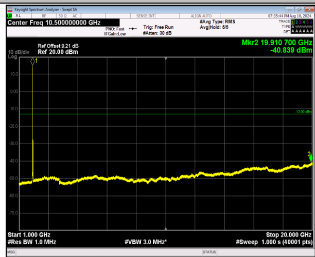
2-2-20MHz-20MHz-16QAM-16QAM-18902-19100-1RB#0-1 RB#99-1000~20000MHz-PASS
