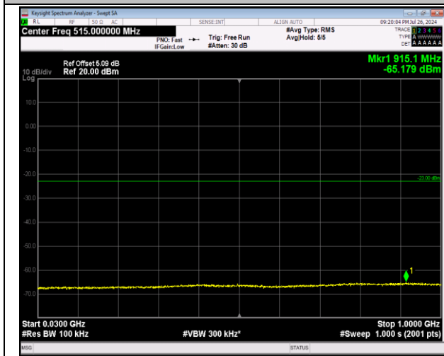
2-2-20MHz-20MHz-64QAM-64QAM-18902-19100-1RB#0-0RB#0-30~1000MHz-PASS
