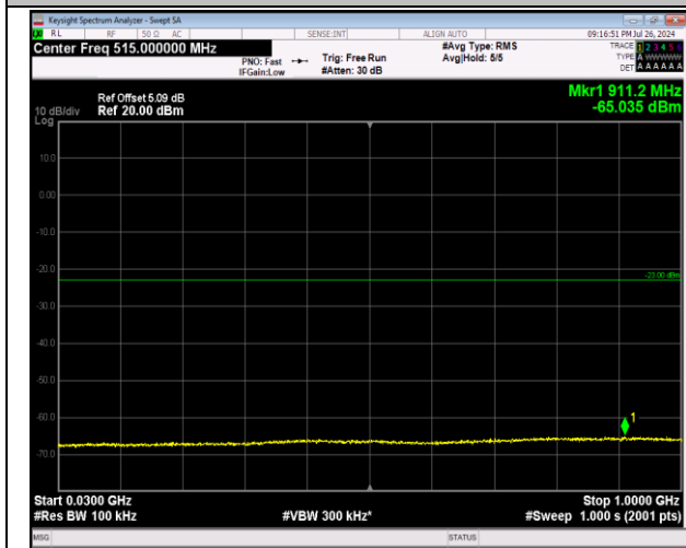
2-2-20MHz-20MHz-64QAM-64QAM-18700-18898-100RB #0-100RB#0-30~1000MHz-PASS
