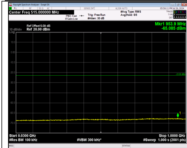
2-2-5MHz-20MHz-64QAM-64QAM-18983-19100-1RB#24 -0RB#0-30~1000MHz-PASS
