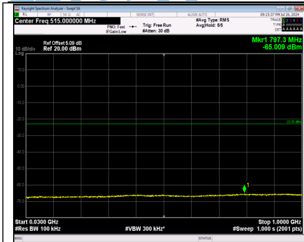
2-2-20MHz-20MHz-64QAM-64QAM-18700-18898-1RB#9 9-ORB#0-30~1000MHz-PASS
