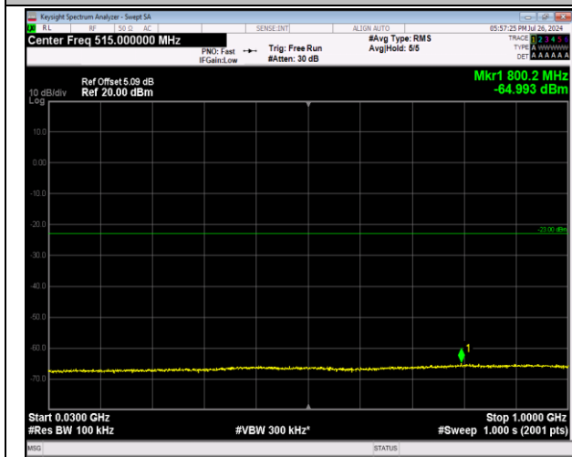
2-2-5MHz-20MHz-64QAM-64QAM-18983-19100-25RB#0 -100RB#0-30~1000MHz-PASS
