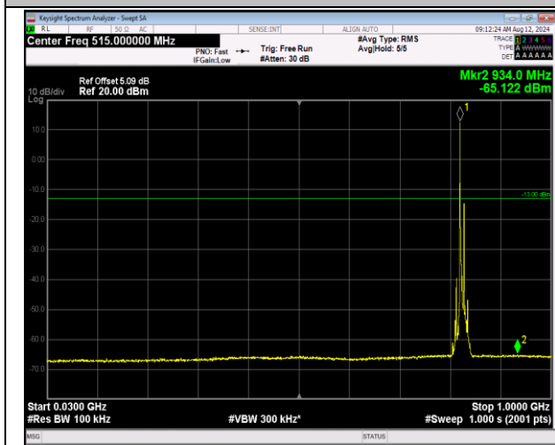
5-5-3MHz-5MHz-16QAM-16QAM-20416-20455-1RB#0-1 RB#24-30~1000MHz-PASS
