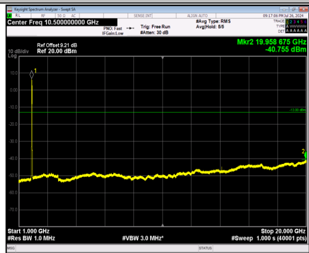
2-2-20MHz-20MHz-64QAM-64QAM-18700-18898-100RB#0 -100RB#0-1000~20000MHz-PASS
