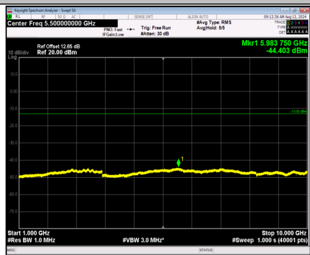
5-5-3MHz-5MHz-16QAM-16QAM-20416-20455-1RB#0-1R B#24-1000~10000MHz-PASS
