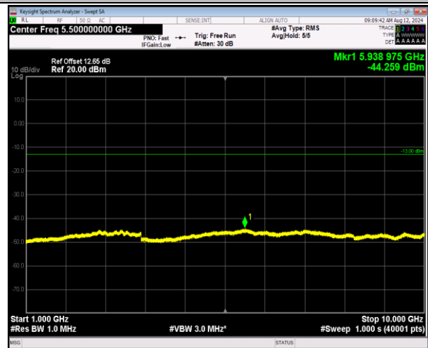
5-5-3MHz-5MHz-QPSK-QPSK-20416-20455-1RB#0-0RB#0 -1000~10000MHz-PASS
