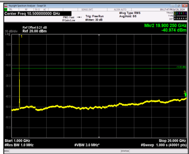
2-2-20MHz-20MHz-64QAM-64QAM-18801-18999-1RB#0-0 RB#0-1000~20000MHz-PASS
