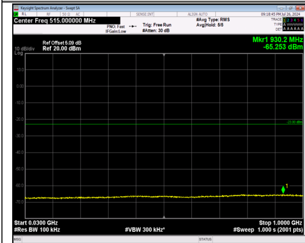
2-2-20MHz-20MHz-64QAM-64QAM-18801-18999-1RB#0 -1RB#99-30~1000MHz-PASS
