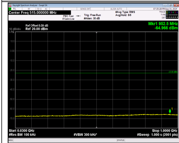
2-2-20MHz-20MHz-16QAM-16QAM-18902-19100-1RB#0 -1RB#99-30~1000MHz-PASS
