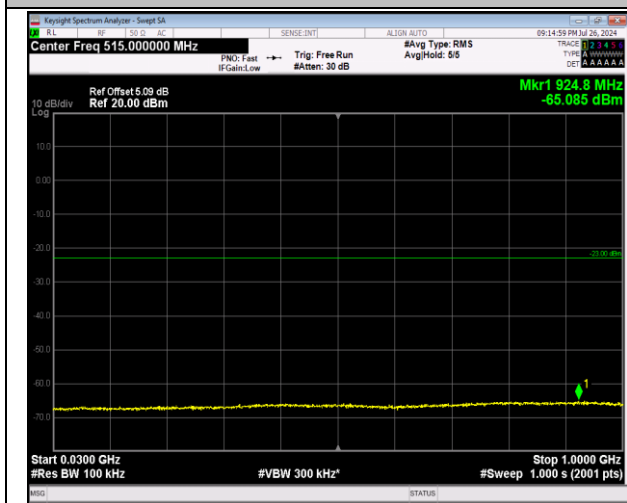
2-2-20MHz-20MHz-64QAM-64QAM-18700-18898-1RB#0 -0RB#0-30~1000MHz-PASS
