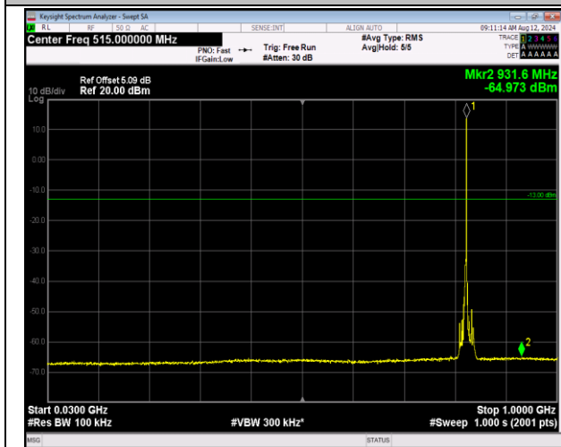
5-5-3MHz-5MHz-16QAM-16QAM-20416-20455-1RB#14- ORB#0-30~1000MHz-PASS
