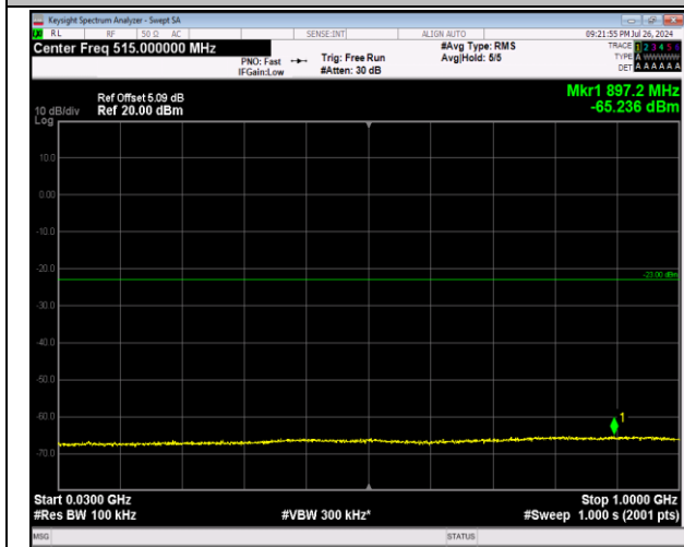
2-2-20MHz-20MHz-64QAM-64QAM-18902-19100-100RB #0-100RB#0-30~1000MHz-PASS
