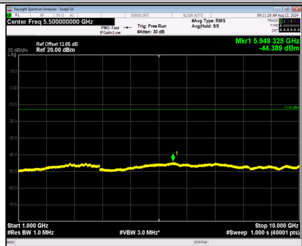
5-5-3MHz-5MHz-16QAM-16QAM-20416-20455-1RB#14-0R B#0-1000~10000MHz-PASS
