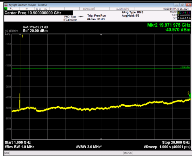
2-2-20MHz-20MHz-64QAM-64QAM-18902-19100-1RB#99- 0RB#0-1000~20000MHz-PASS
