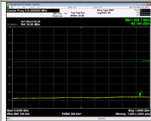
2-2-20MHz-20MHz-64QAM-64QAM-18801-18999-1RB#0 -0RB#0-30~1000MHz-PASS
