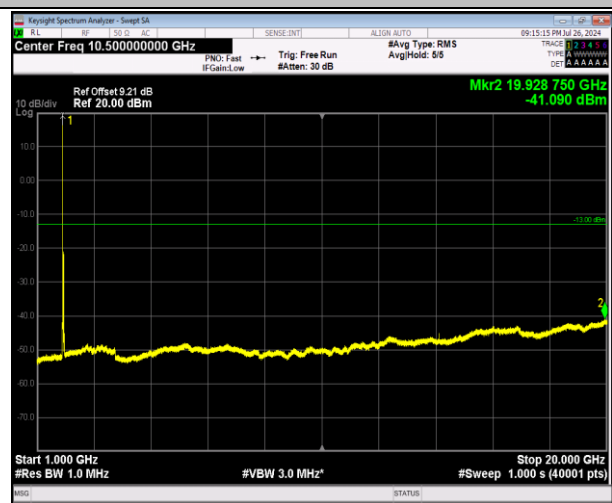
2-2-20MHz-20MHz-64QAM-64QAM-18700-18898-1RB#0-0 RB#0-1000~20000MHz-PASS
