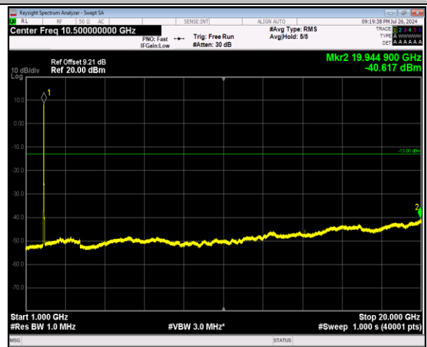
2-2-20MHz-20MHz-64QAM-64QAM-18801-18999-100RB#0 -100RB#0-1000~20000MHz-PASS
