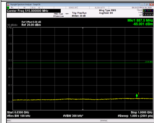
2-2-20MHz-20MHz-64QAM-64QAM-18801-18999-100RB #0-100RB#0-30~1000MHz-PASS
