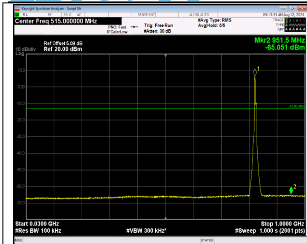
5-5-3MHz-5MHz-16QAM-16QAM-20416-20455-15RB#0-0-25RB#0-30~1000MHz-PASS
