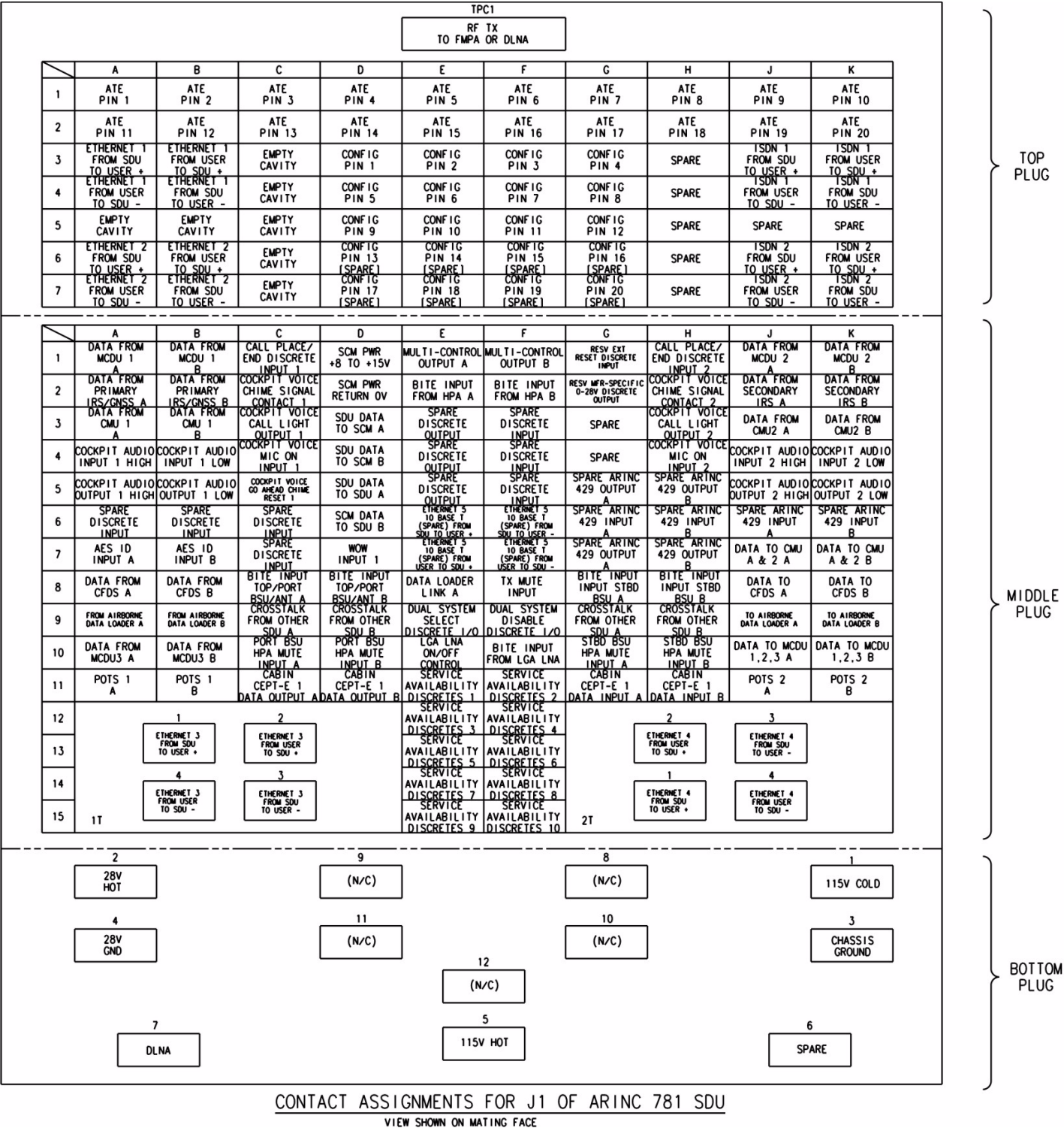
Figure 3-9 ARINC 781 System Interconnect Drawing, 1394-B-1001 Rev A00 (Sheet 3 of 3)
