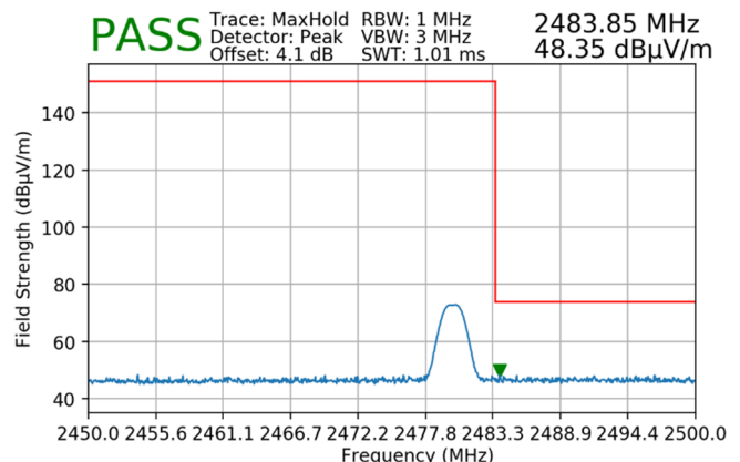
Plot 7-24. Radiated Restricted Upper Band Edge Measurement (Peak)
