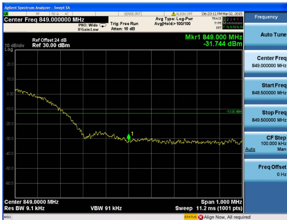
Fig.40 WCDMA Band V-CH4232Band Edge Compliance(HSDPA Subtest1)
