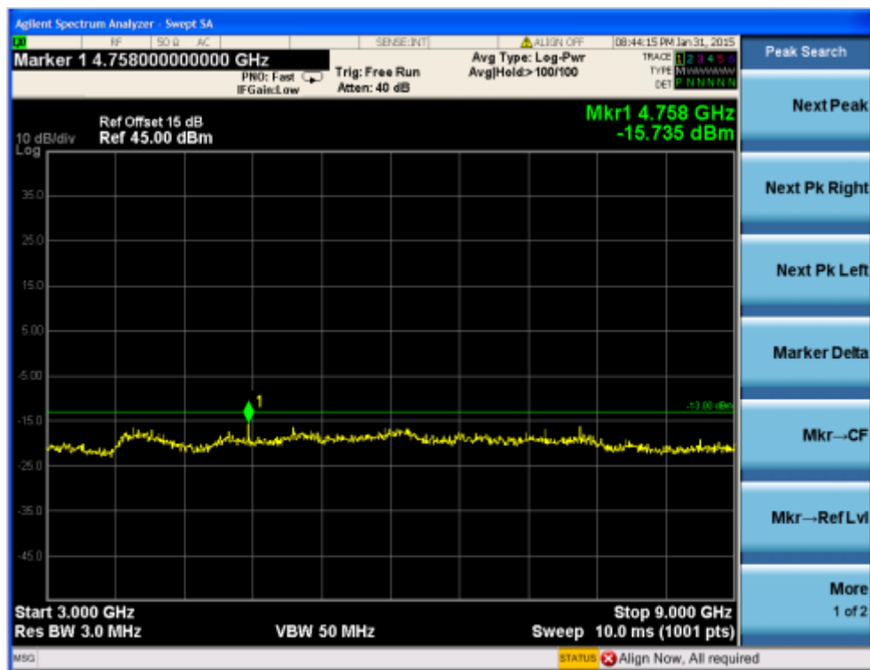
Fig.54 WCDMA Band V on Channel 4175 3GHz~9GHz
