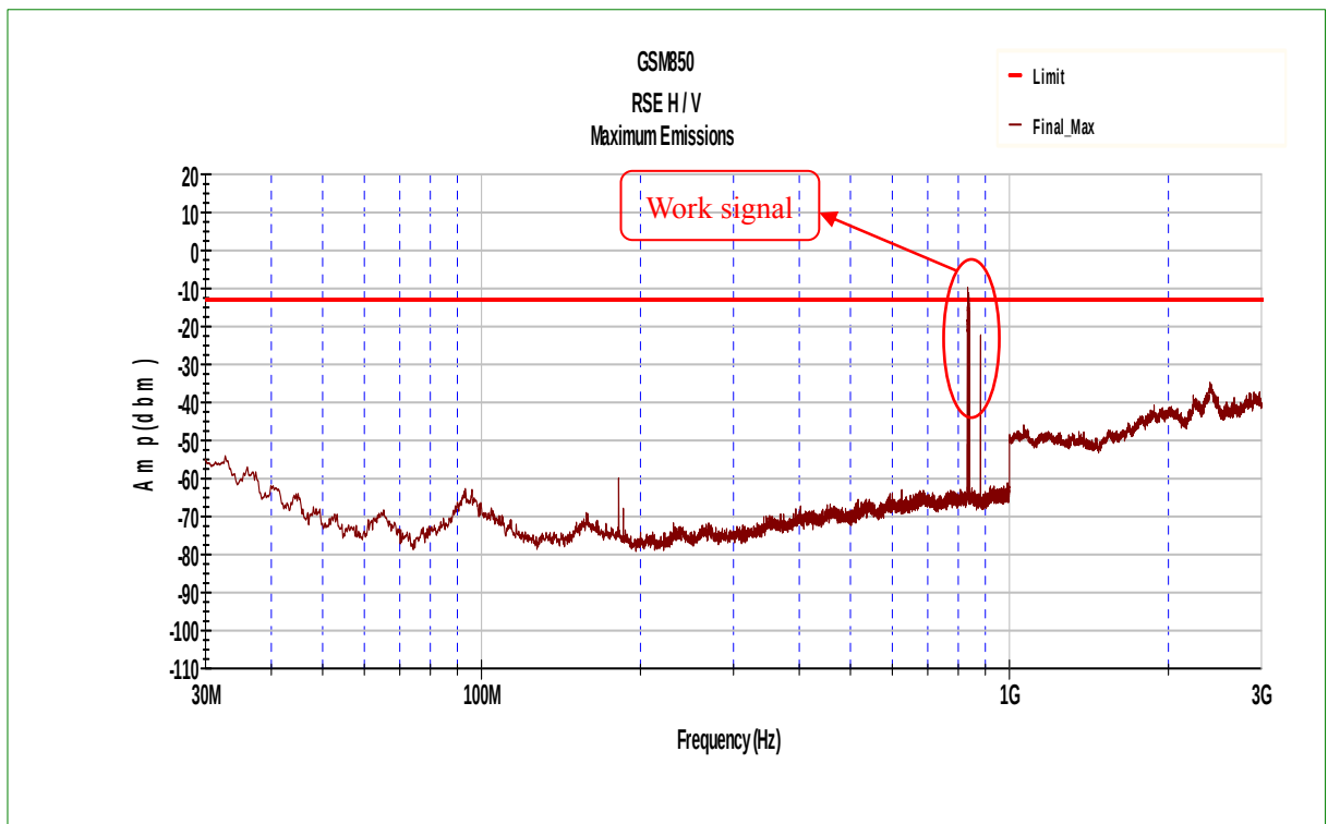
Fig.25 GSM850 on Channel 189 30MHz~3GHz
