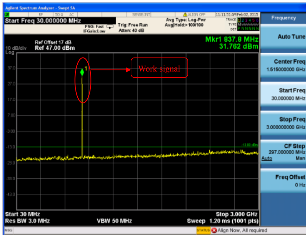
Fig.49 GSM850 on Channel 189 30MHz~3GHz
