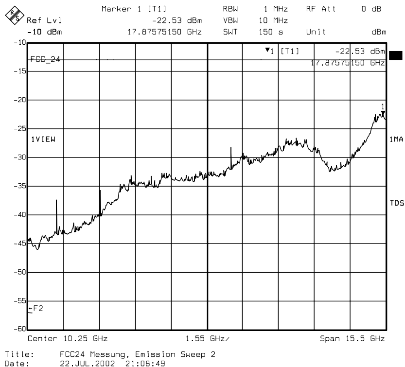
diagram 8.24: carrier on channel 661 (1880 MHz), TCH mode
