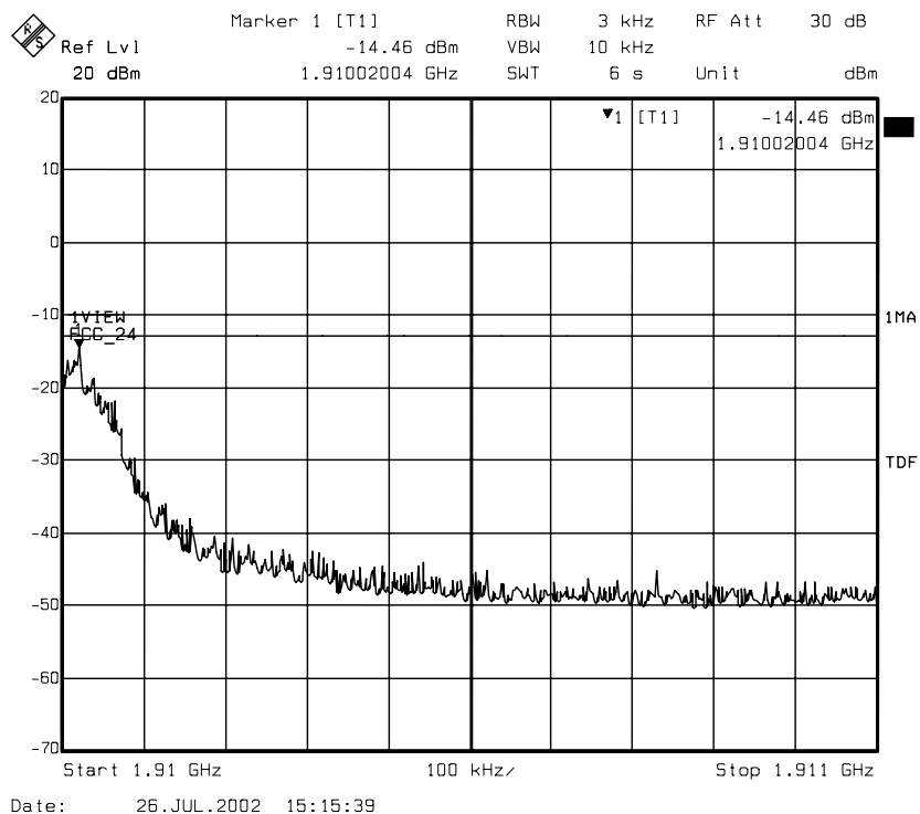
diagram 8.15: carrier on channel 810 (1909,8 MHz), TCH mode
