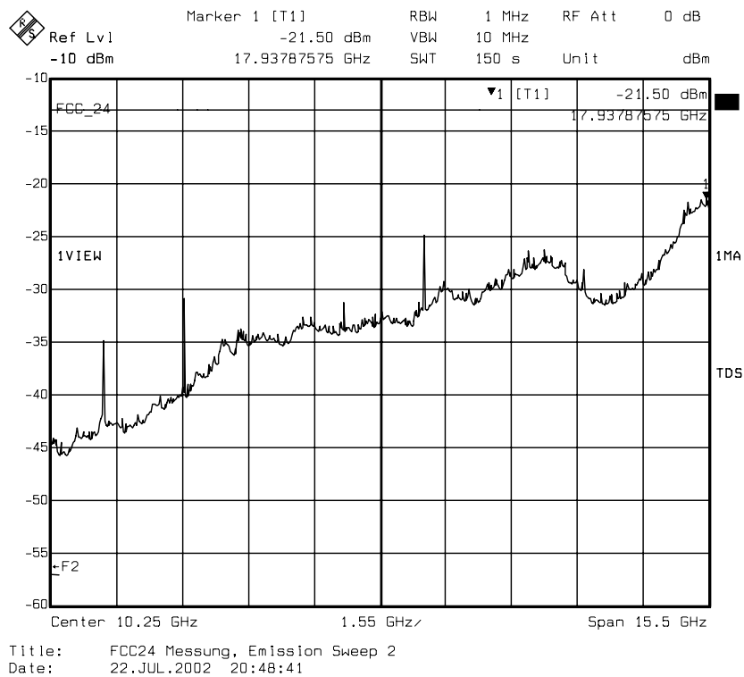
diagram 8.08: carrier on channel 661 (1880 MHz), TCH mode
