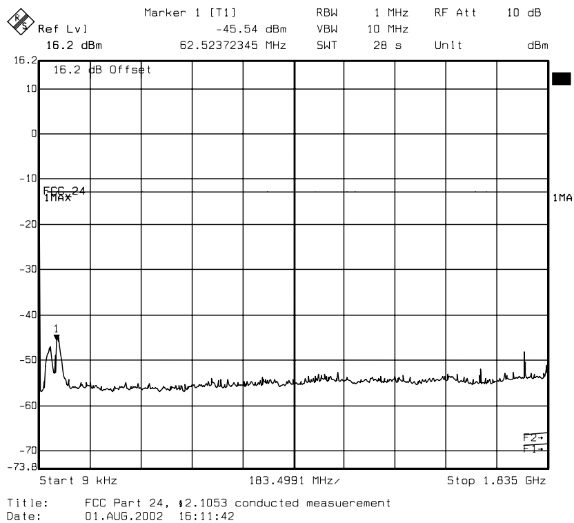
diagram 14.10: carrier on channel 810 (1909.8 MHz)
