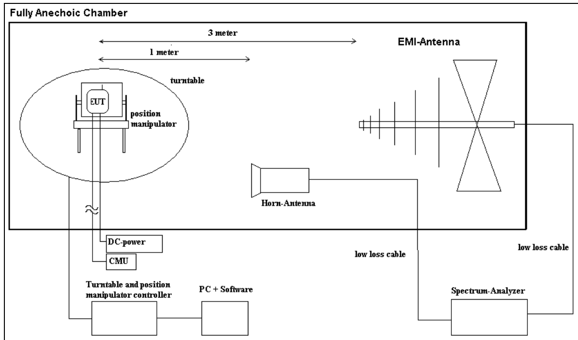
Block diagram: Test set-up 2
