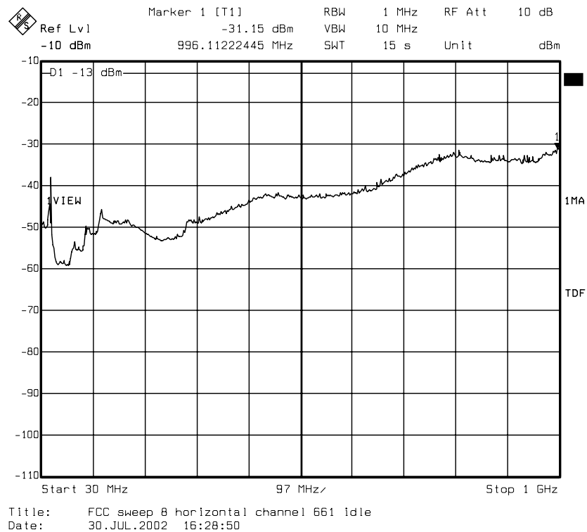
diagram 8.33: carrier on channel 661 (1880,0 MHz), IDLE mode
