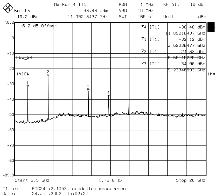
diagram 14.03: carrier on channel 512 (1850,2 MHz)
