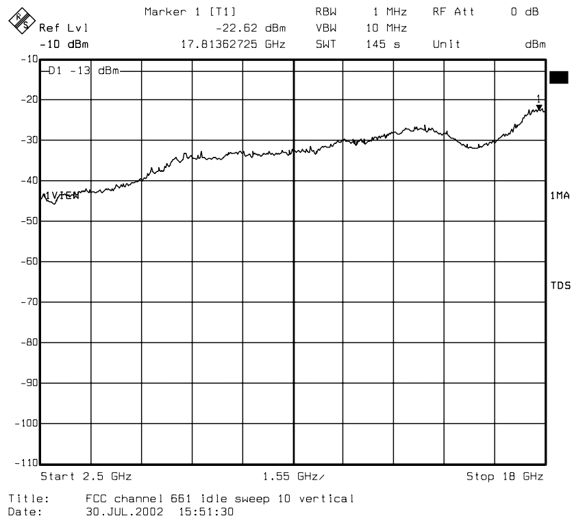
diagram 8.39: carrier on channel 661 (1880,0 MHz), IDLE mode
