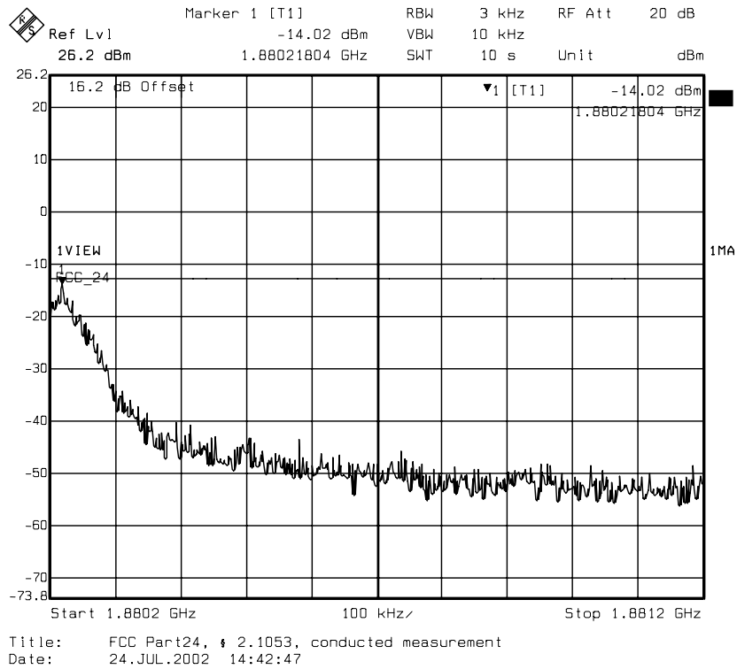
diagram 14.09: carrier on channel 661 (1880 MHz)
