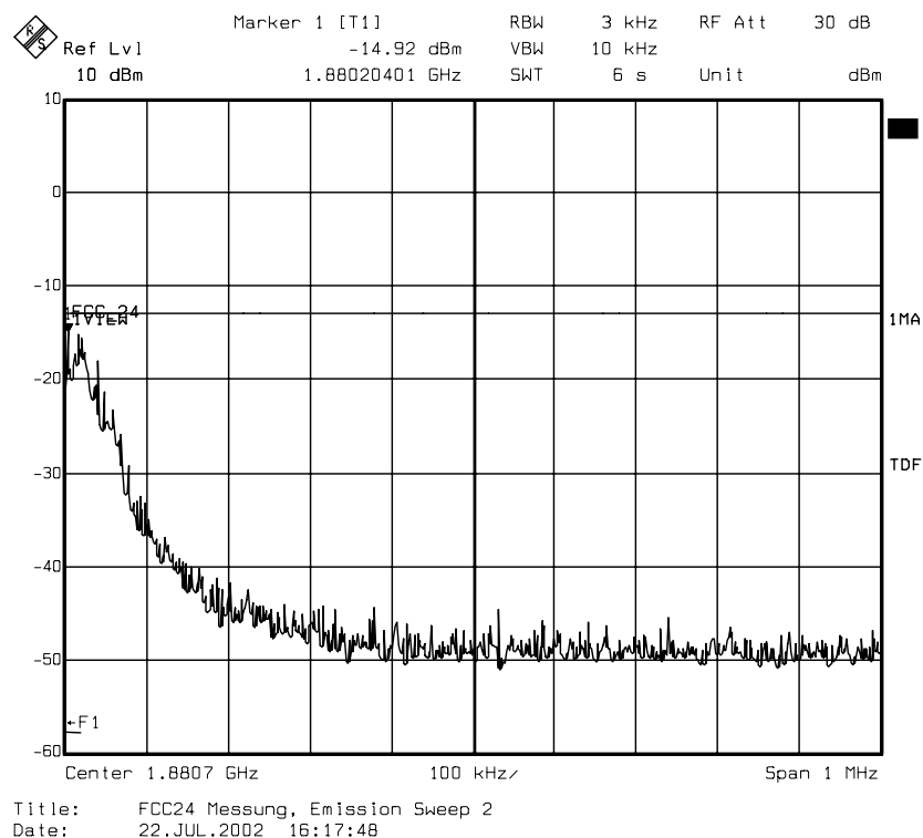
diagram 8.10: carrier on channel 661 (1880 MHz), TCH mode
