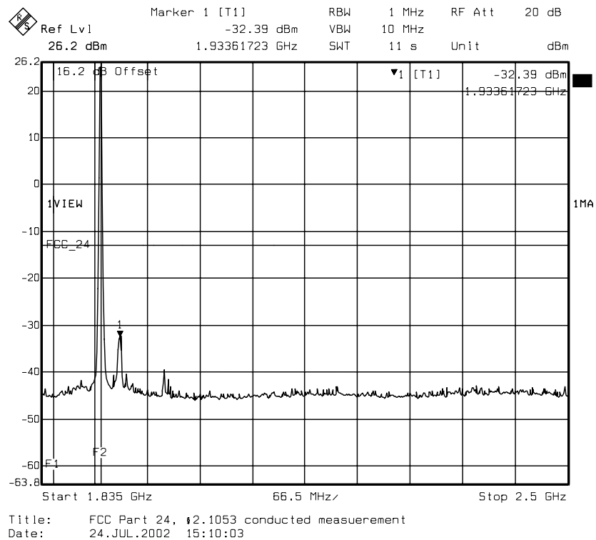
diagram 14.11: carrier on channel 810 (1909.8 MHz)
