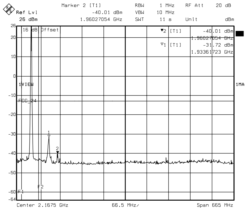
diagram 14.06: carrier on channel 661 (1880 MHz)
