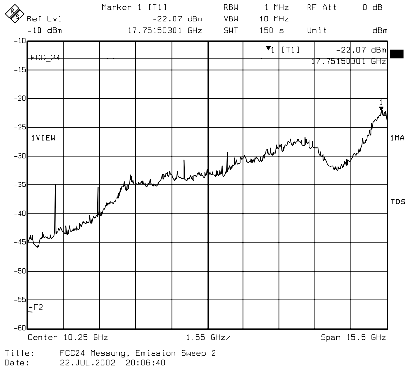
diagram 8.19: carrier on channel 512 (1850,2 MHz), TCH mode
