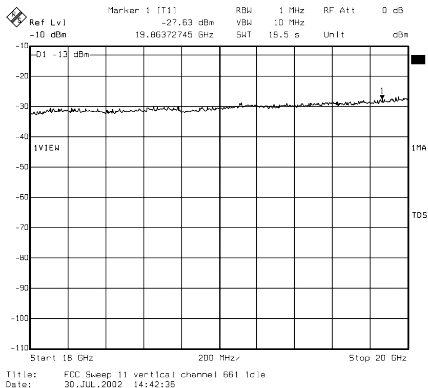
diagram 8.40: carrier on channel 661 (1880,0 MHz), IDLE mode
