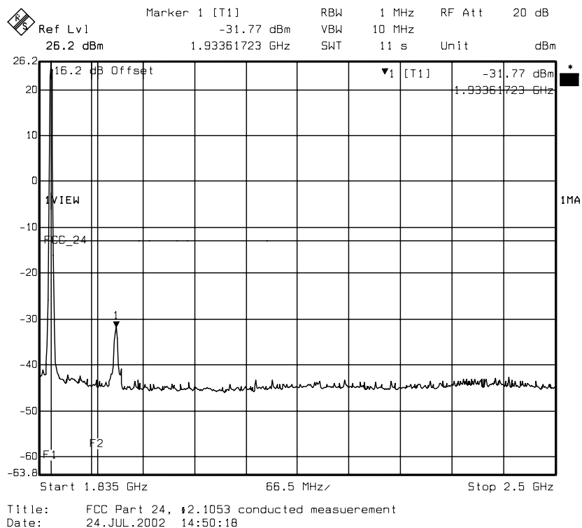
diagram 14.02: carrier on channel 512 (1850,2 MHz)
