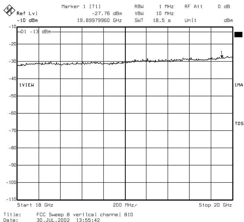
diagram 8.32: carrier on channel 810 (1909,8 MHz), TCH mode
