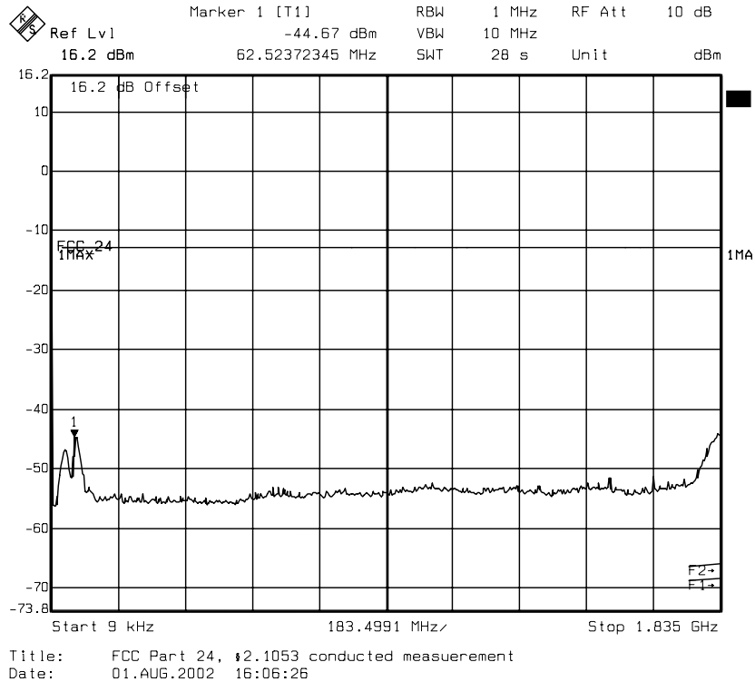
diagram 14.01: carrier on channel 512 (1850,2 MHz)
