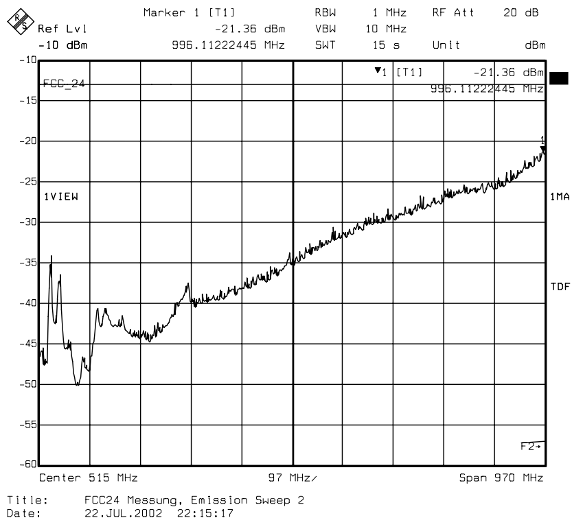
diagram 8.28: carrier on channel 810 (1909,8 MHz), TCH mode
