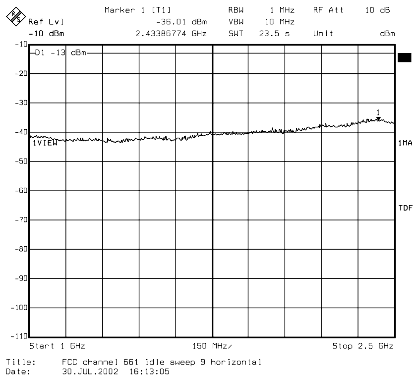
diagram 8.34: carrier on channel 661 (1880,0 MHz), IDLE mode
