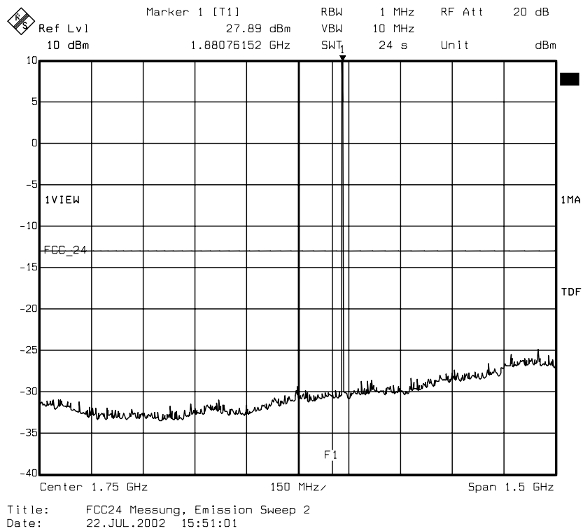
diagram 8.07: carrier on channel 661 (1880 MHz), TCH mode
