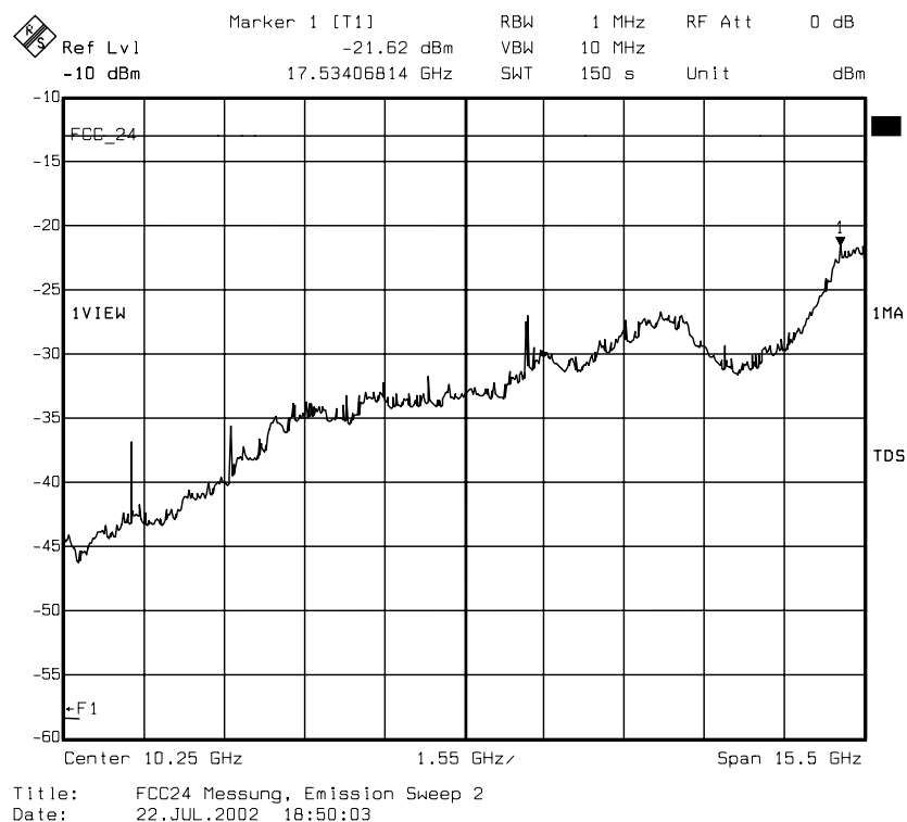
diagram 8.14: carrier on channel 810 (1909,8 MHz), TCH mode
