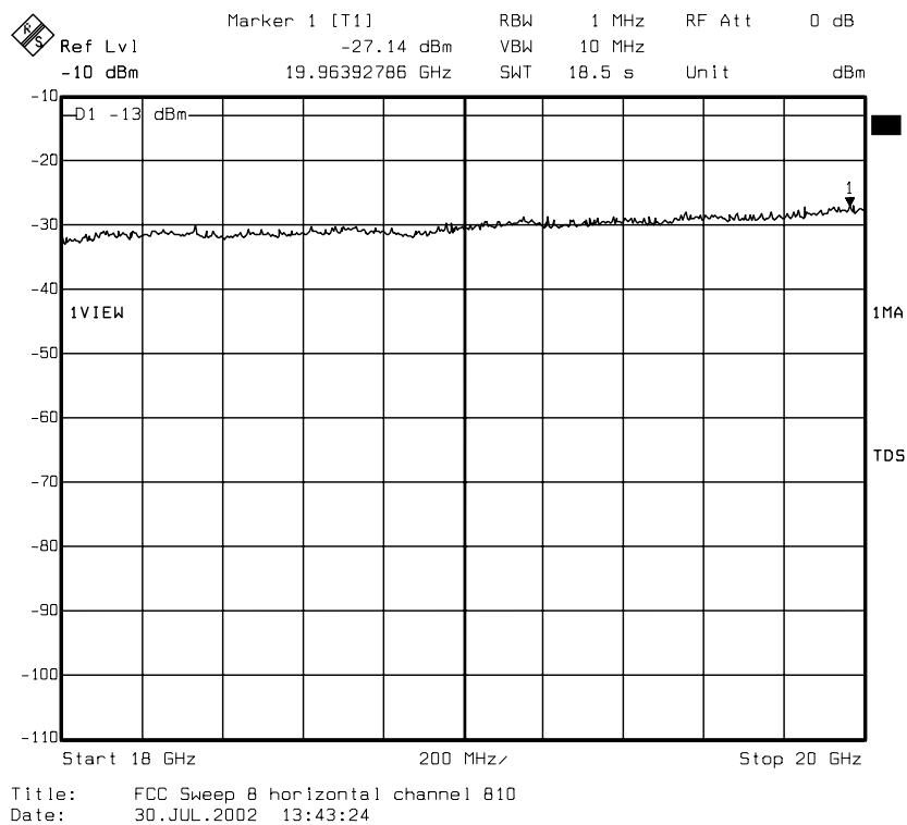
diagram 8.16: carrier on channel 810 (1909,8 MHz), TCH mode
