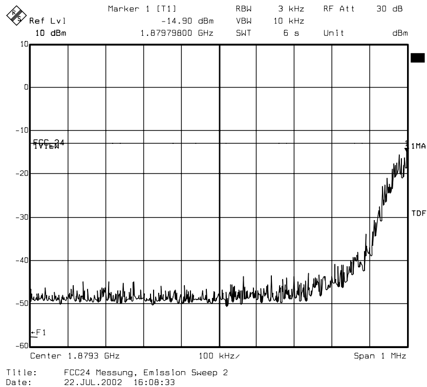
diagram 8.09: carrier on channel 661 (1880 MHz), TCH mode
