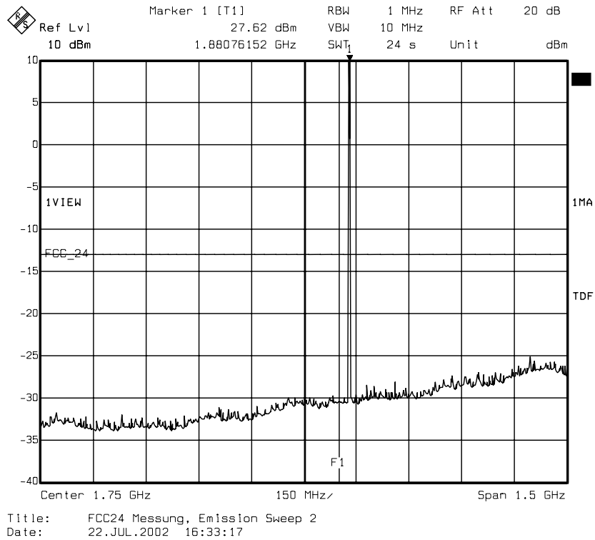
diagram 8.23: carrier on channel 661 (1880 MHz), TCH mode
