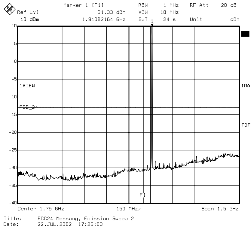
diagram 8.13: carrier on channel 810 (1909,8 MHz), TCH mode
