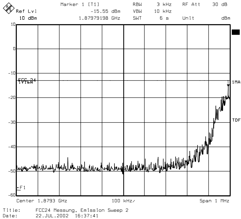
diagram 8.25: carrier on channel 661 (1880 MHz), TCH mode
