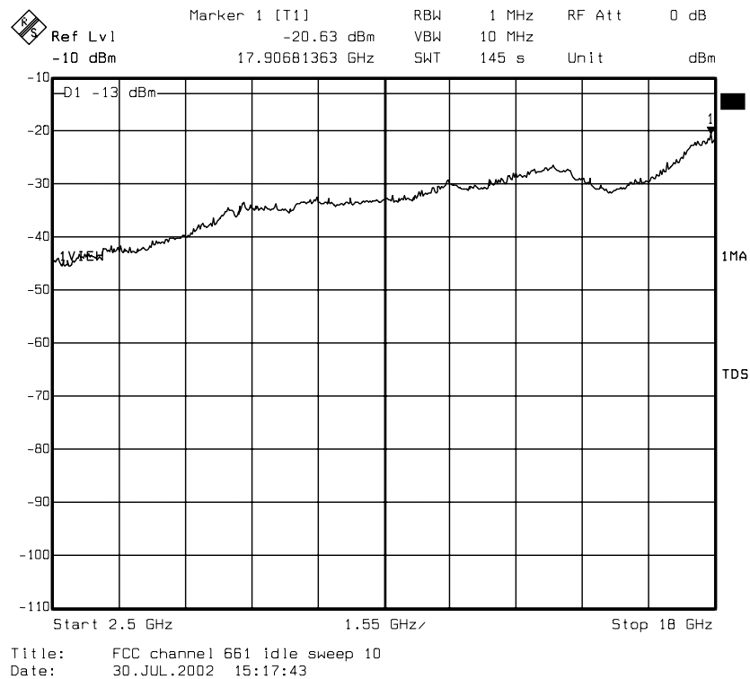
diagram 8.35: carrier on channel 661 (1880,0 MHz), IDLE mode
