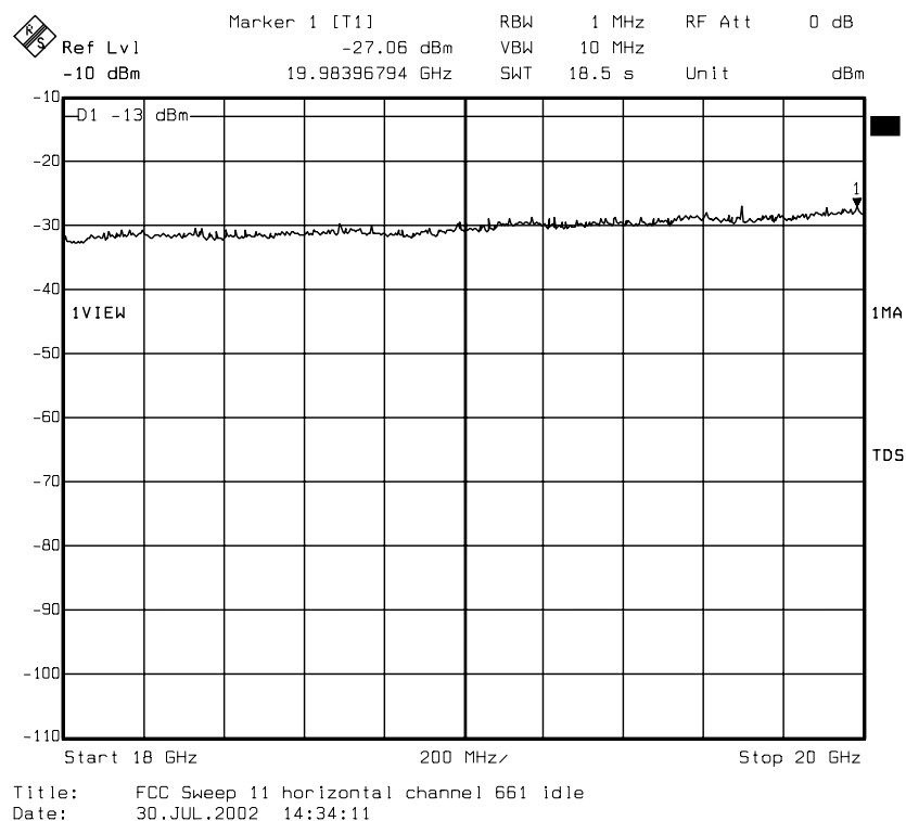
diagram 8.36: carrier on channel 661 (1880,0 MHz), IDLE mode
