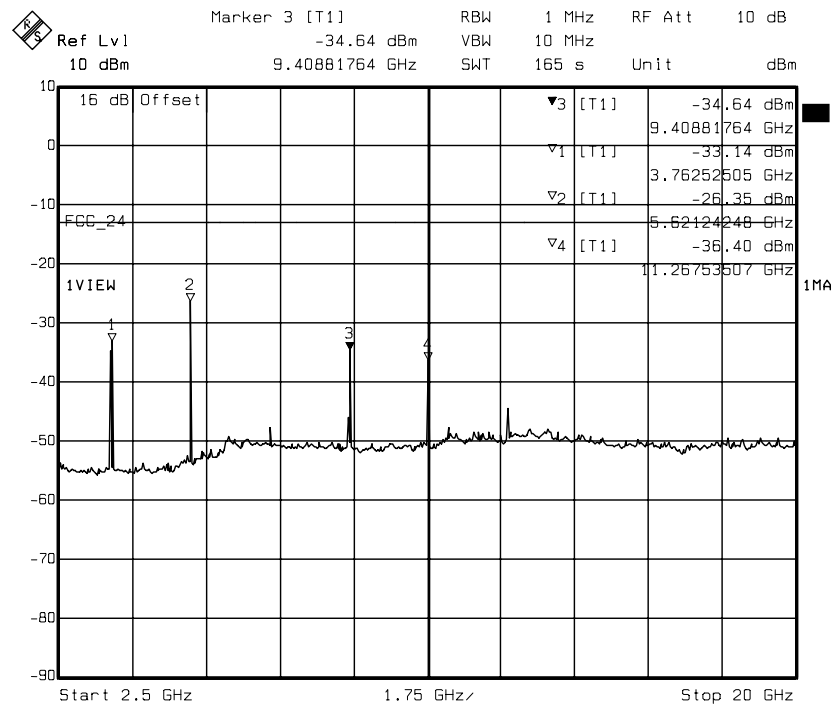
diagram 14.07: carrier on channel 661 (1880 MHz)
