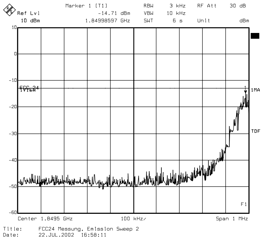
diagram 8.20: carrier on channel 512 (1850,2 MHz), TCH mode
