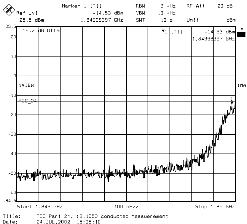
diagram 14.04: carrier on channel 512 (1850,2 MHz)
