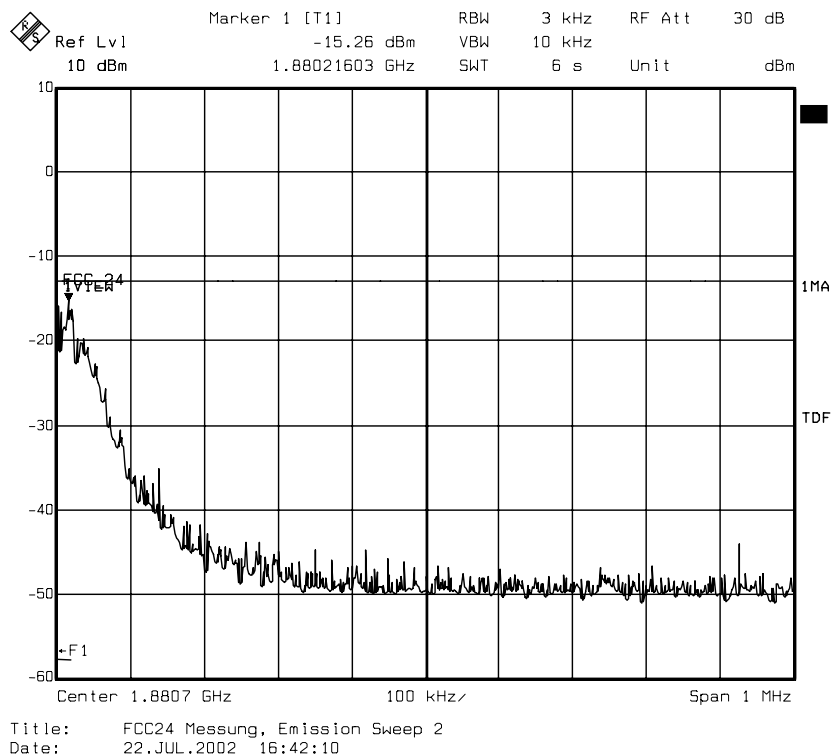
diagram 8.26: carrier on channel 661 (1880 MHz), TCH mode
