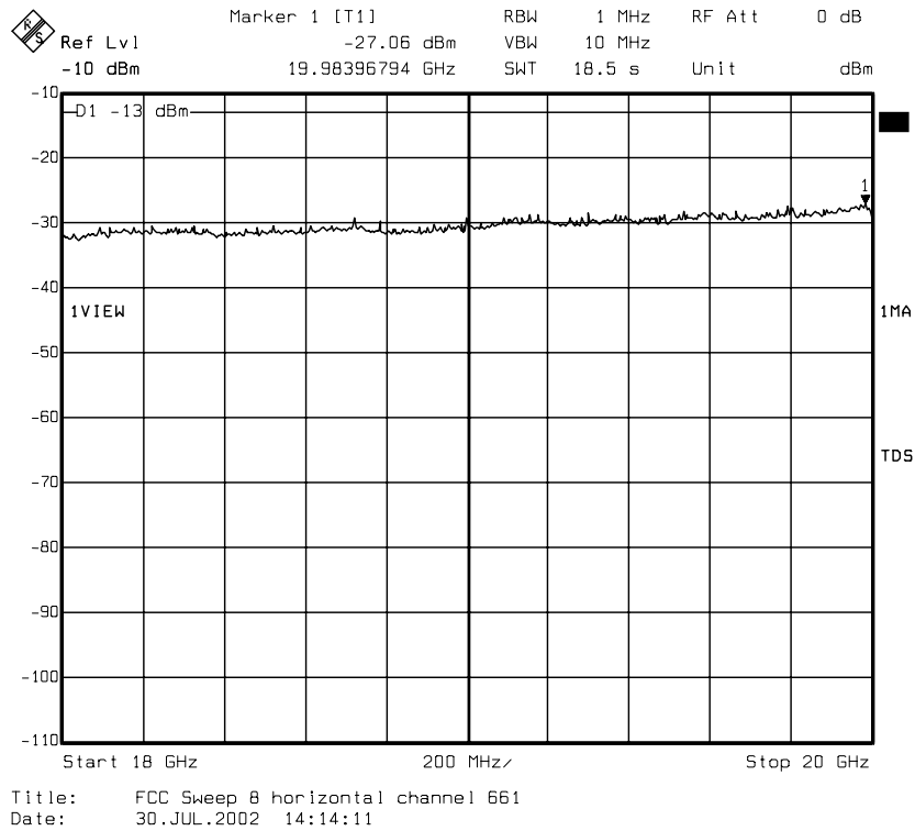
diagram 8.11: carrier on channel 661 (1880 MHz), TCH mode
