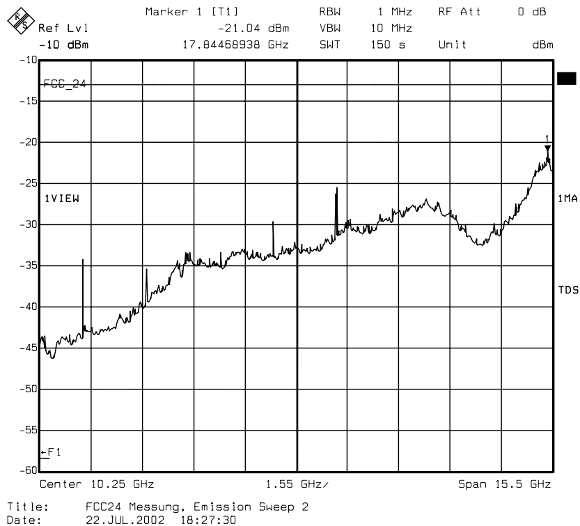
diagram 8.30: carrier on channel 810 (1909,8 MHz), TCH mode
