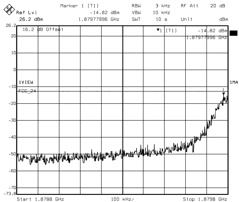
diagram 14.08: carrier on channel 661 (1880 MHz)
