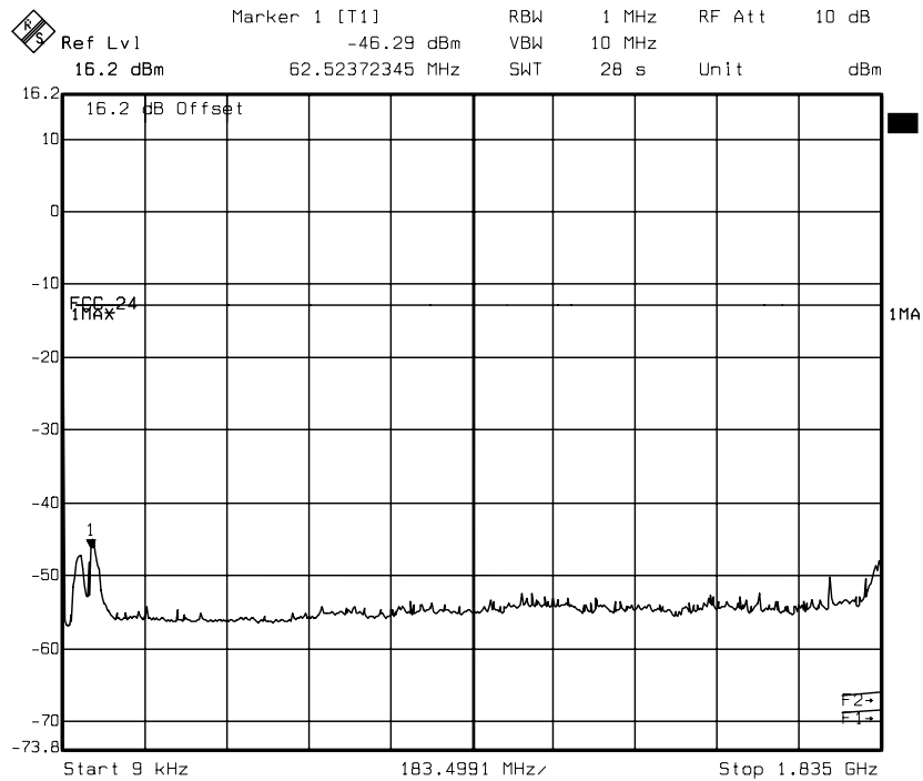
diagram 14.05: carrier on channel 661 (1880 MHz)
