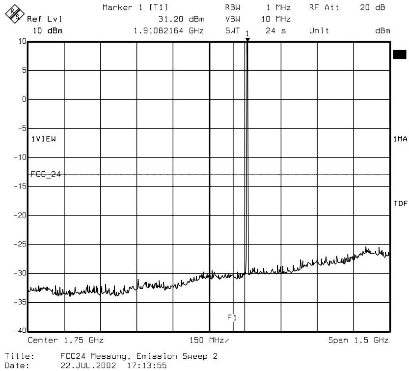
diagram 8.29: carrier on channel 810 (1909,8 MHz), TCH mode
