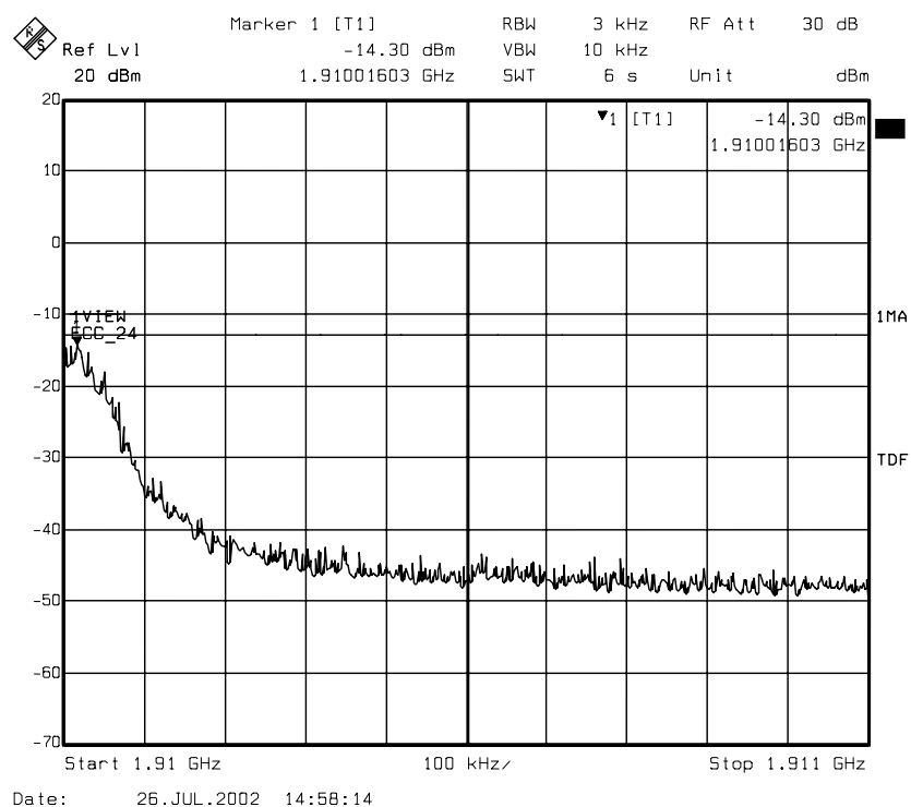
diagram 8.31: carrier on channel 810 (1909,8 MHz), TCH mode
