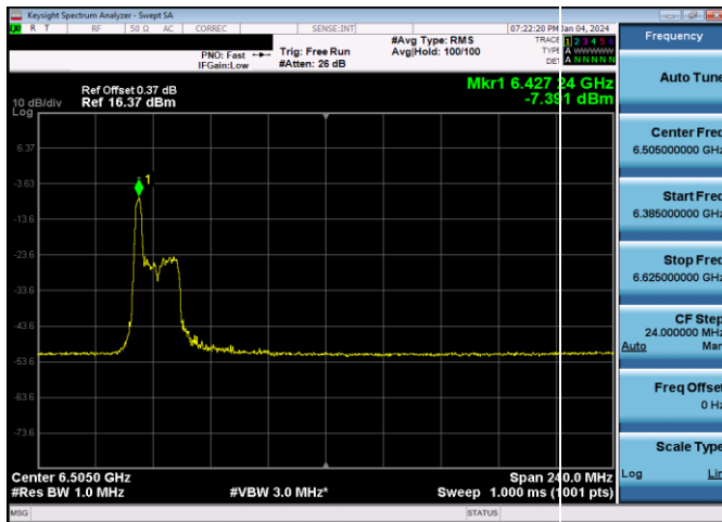
Plot 7-665. LPI Power Spectral Density Plot SDM Antenna WF7a (160MHz 802.11ax RU26 (UNII Band 6) – Ch. 111)
