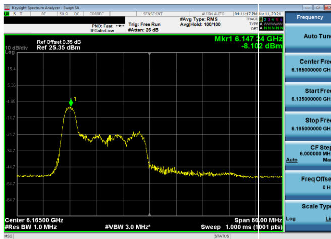
Plot 7-617. LPI Power Spectral Density Plot SDM Antenna WF7a (40MHz 802.11ax RU26 (UNII Band 5) – Ch. 43)
