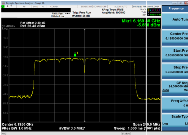
Plot 7-640. LPI Power Spectral Density Plot SDM Antenna WF2a (160MHz 802.11ax RU996x2 (UNII Band 5) – Ch. 47)
