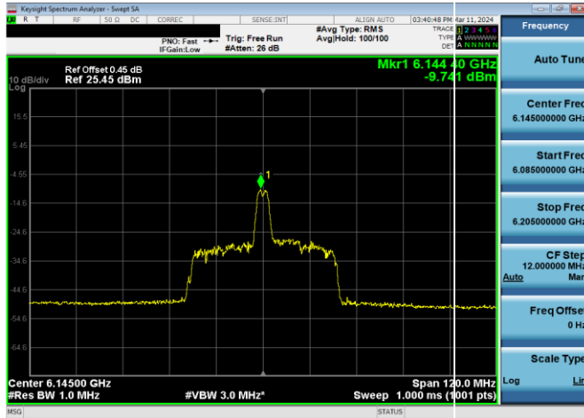
Plot 7-628. LPI Power Spectral Density Plot SDM Antenna WF2a (80MHz 802.11ax RU26 (UNII Band 5) – Ch. 39)
