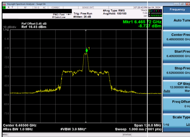
Plot 7-659. LPI Power Spectral Density Plot SDM Antenna WF7a (80MHz 802.11ax RU26 (UNII Band 6) – Ch. 103)
