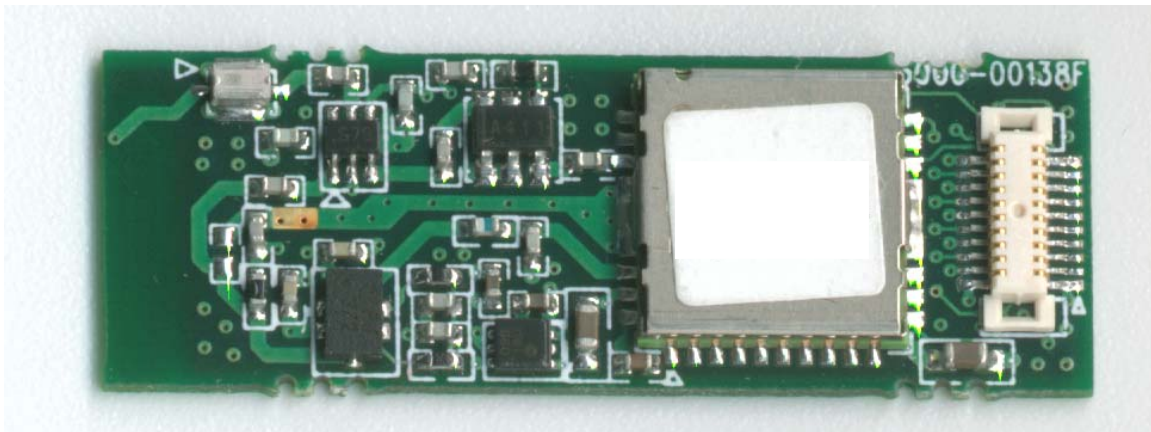
Component Side
