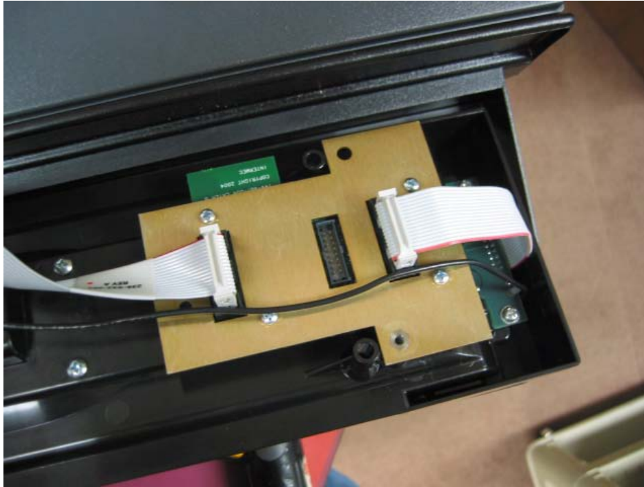
CK60 holder rotated to show PCB mounting
