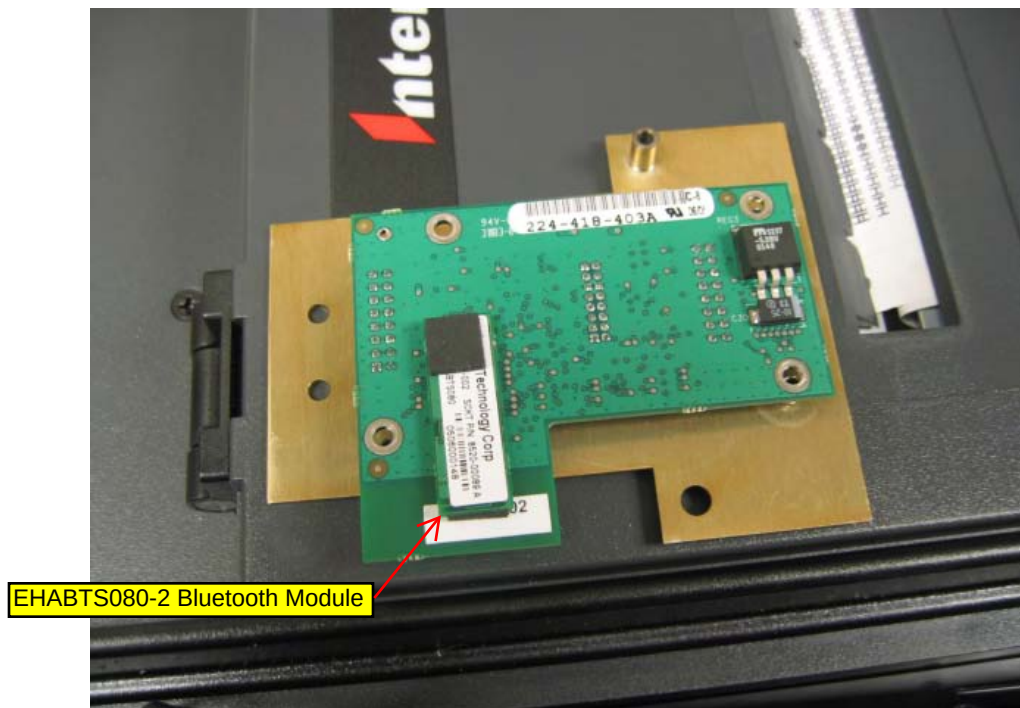
PCB removed to show EHABTS080-2 module location
