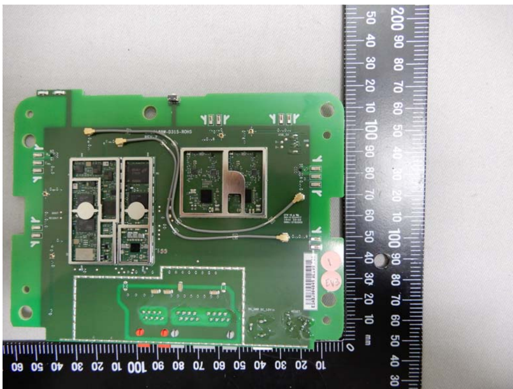
Internal View of EUT – 6 (2 nd PCB)
