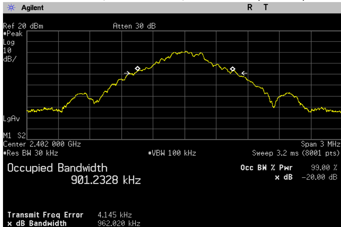
20 dB & 99% Bandwidth, GFSK modulation, Lowest Channel (2 402 MHz)
