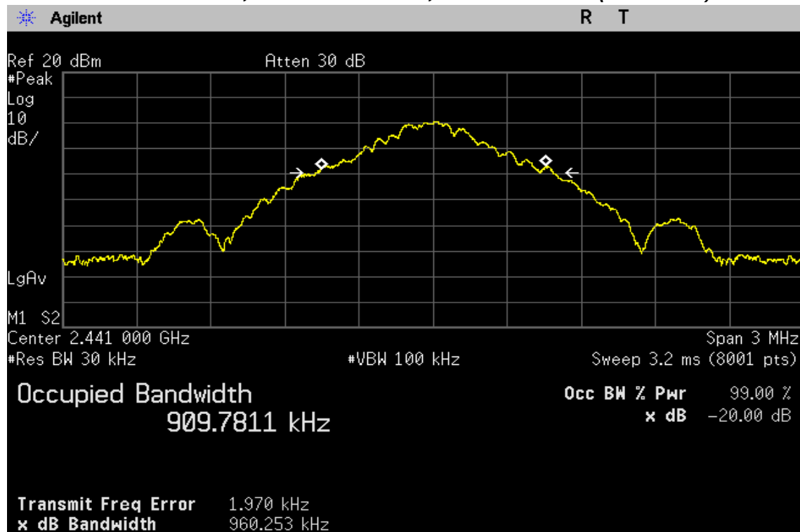
20 dB & 99% Bandwidth, GFSK modulation, Middle Channel (2 441 MHz)
