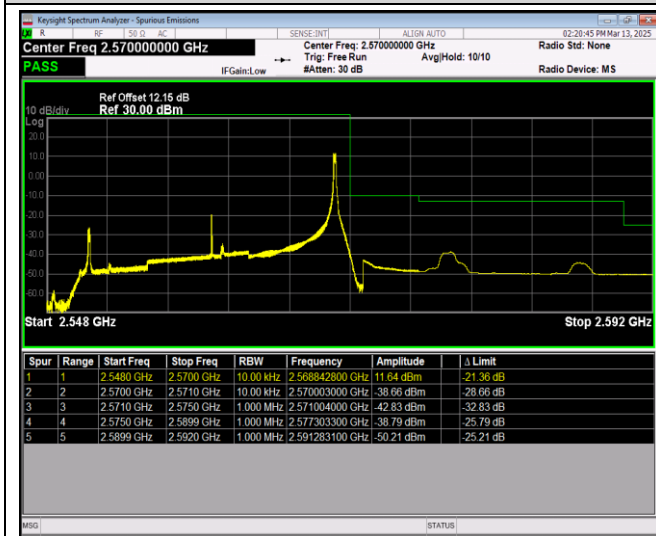
Band38-5MHz-QPSK-37775-1RB#0
