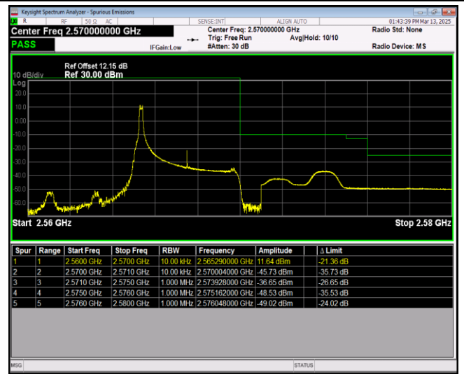
Band7-5MHz-QPSK-21425-25RB#0
