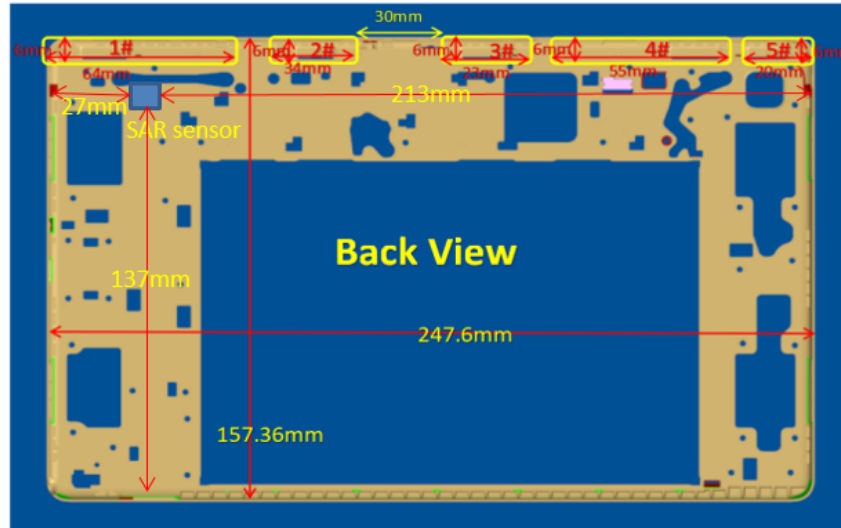
SAR Sensor Trigger
