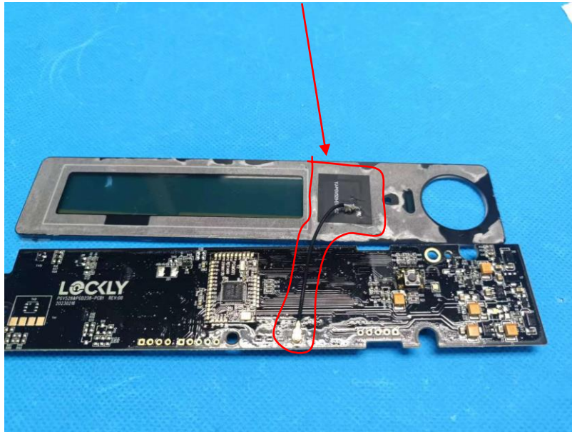
View of BT antenna
