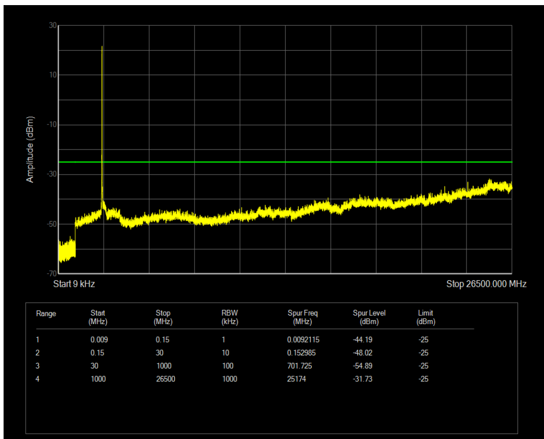
Band41(2555-2655) 16QAM BW=10MHz Channel=40290 RB Size=1 Position=#0
