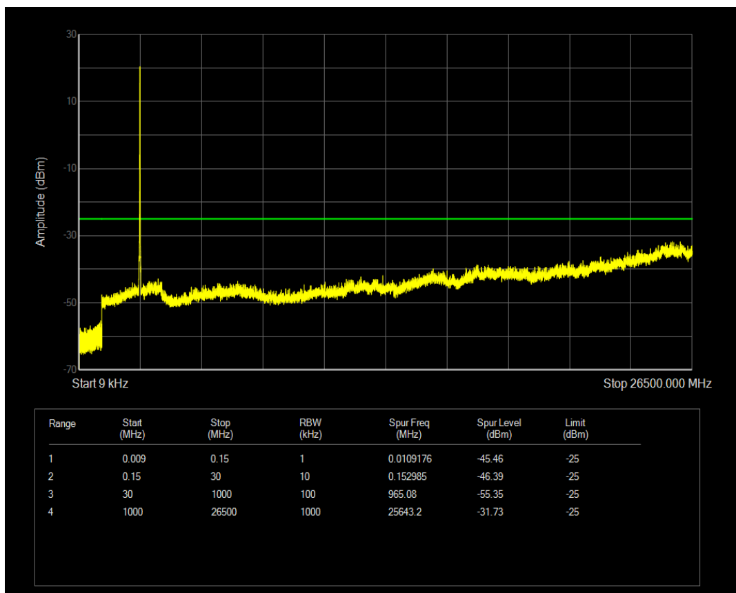
Band41(2555-2655) QPSK BW=15MHz Channel=40315 RB Size=1 Position=#0
