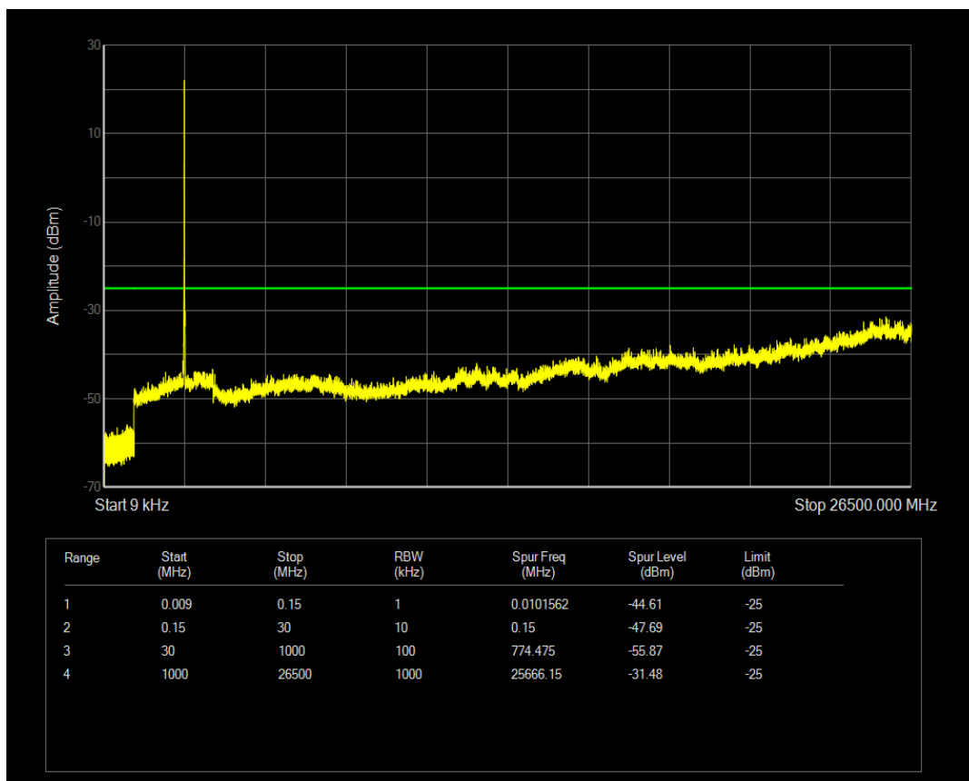
Band41(2555-2655) 16QAM BW=5MHz Channel=41215 RB Size=1 Position=#0
