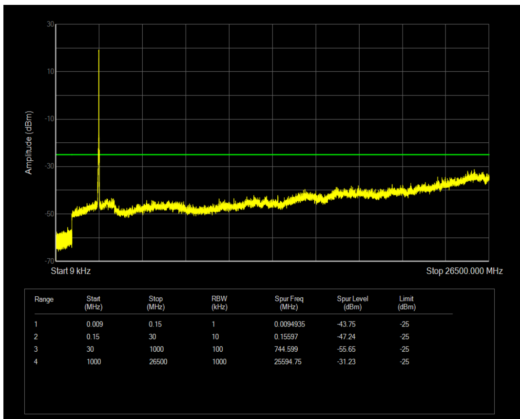
Band41(2555-2655) 16QAM BW=15MHz Channel=41165 RB Size=1 Position=#0
