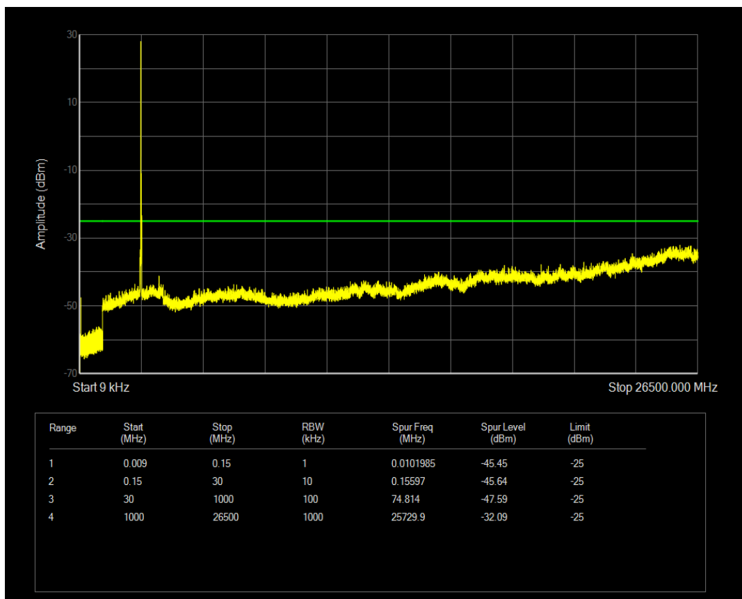
Band41(2555-2655) 16QAM BW=20MHz Channel=41140 RB Size=100 Position=#0
