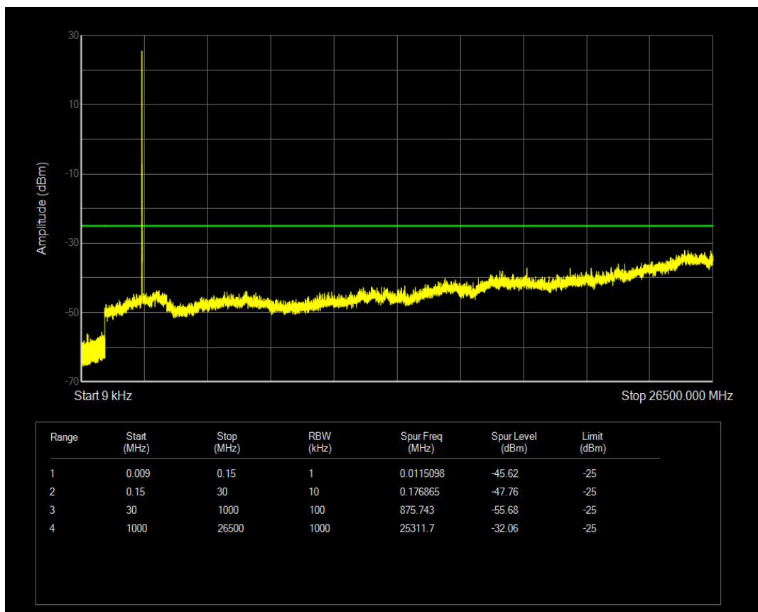
Band41(2555-2655) 16QAM BW=10MHz Channel=40290 RB Size=50 Position=#0
