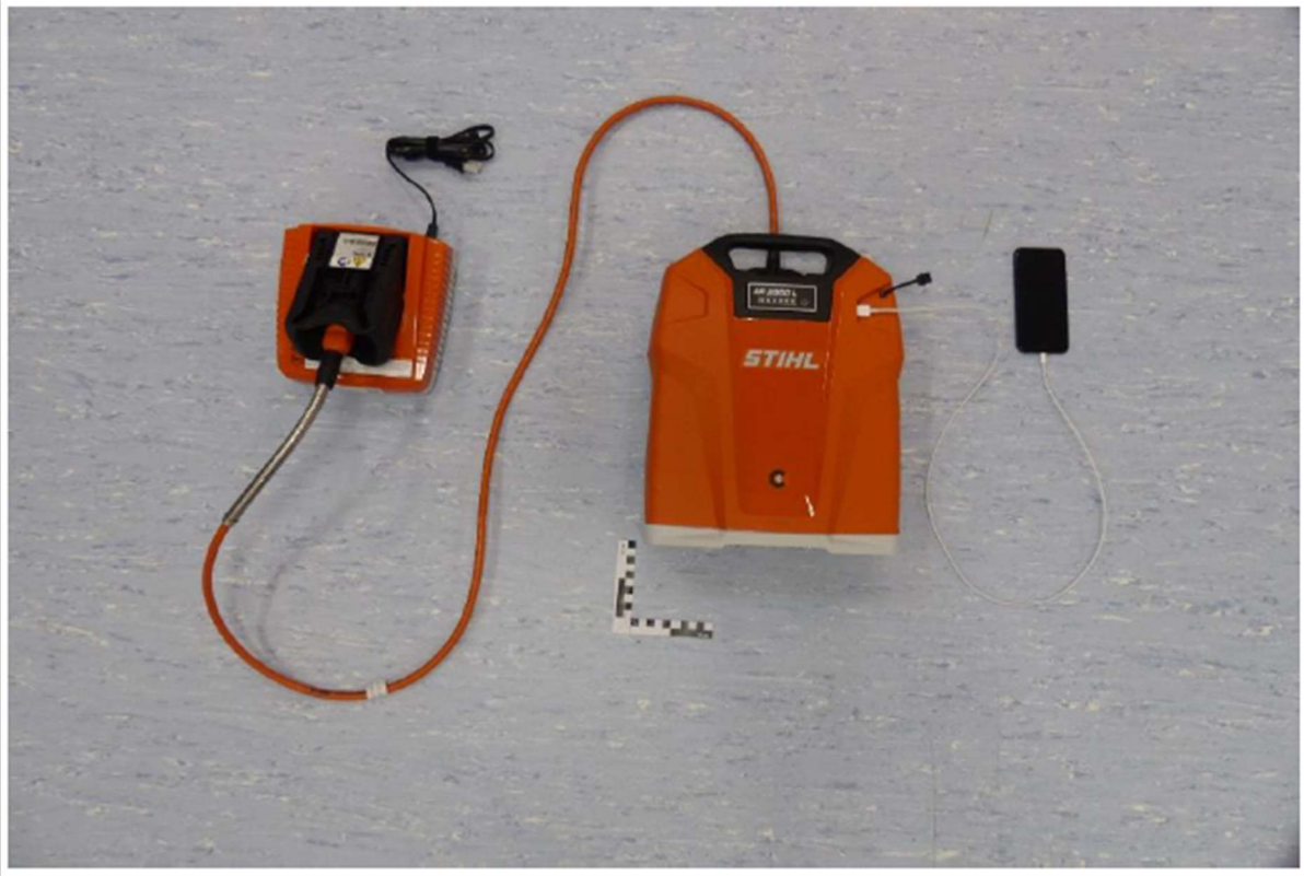
EUT + Auxiliary Equipment EUT Configuration 2
