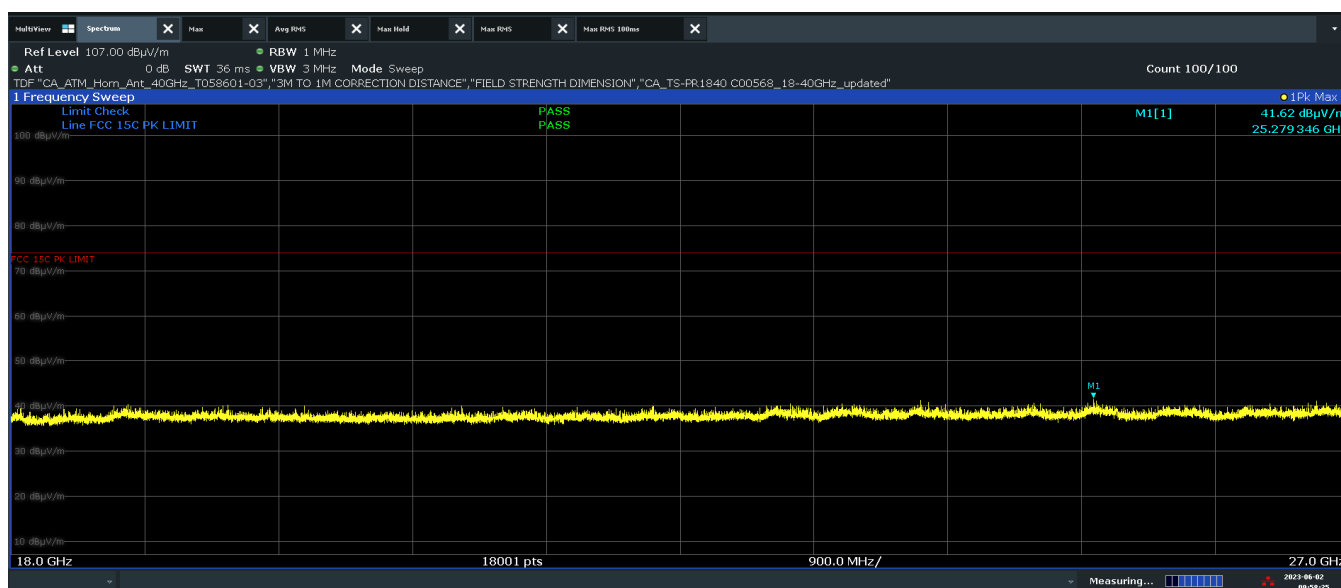
Plot 7-30. Radiated Spurious Emissions Above 18GHz V Polarity (Co-Tx)
