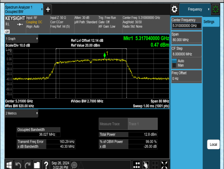
11N40MIMO-Ant2-5310
