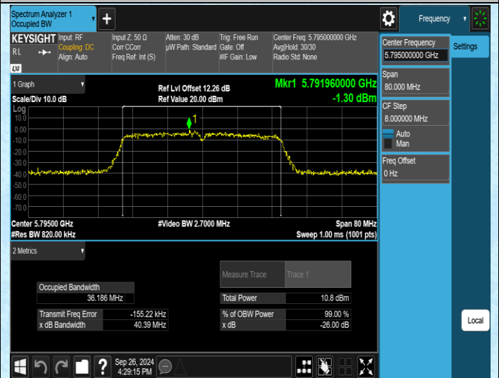
11AC40MIMO-Ant2-5795
