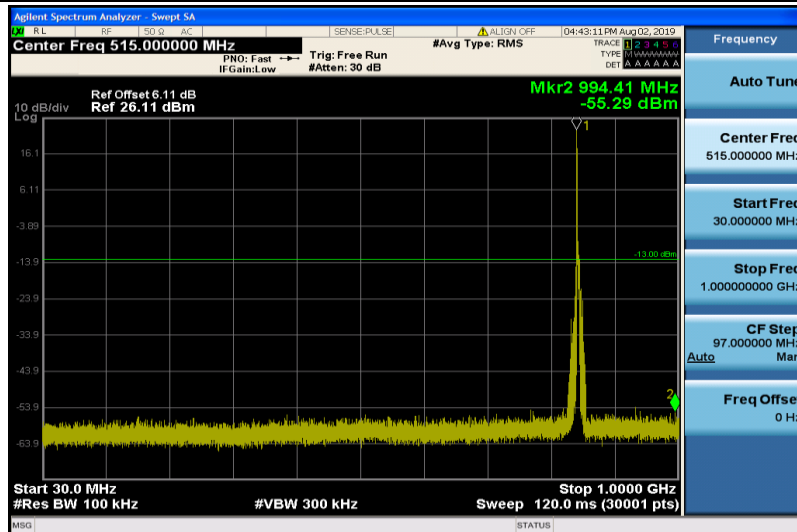
Band5-5MHz-QPSK-20625-1RB#0-30~1000MHz
