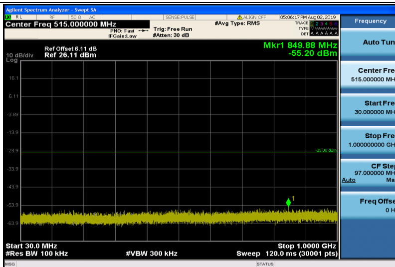
Band7-10MHz-16QAM-20800-1RB#0-30~1000MHz
