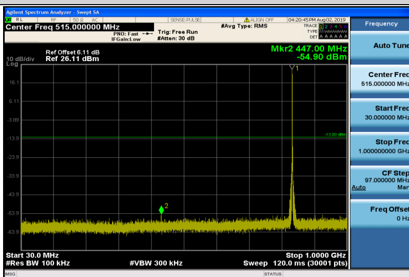
Band5-1.4MHz-QPSK-20525-1RB#0-30~1000MHz
