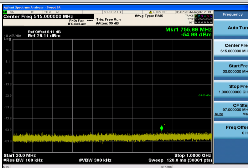
Band7-10MHz-16QAM-21100-1RB#0-30~1000MHz
