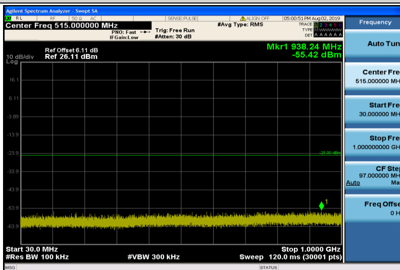
Band7-5MHz-16QAM-21425-1RB#0-30~1000MHz
