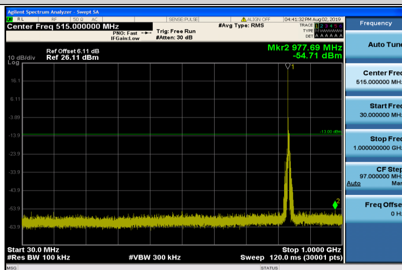
Band5-5MHz-16QAM-20525-1RB#0-30~1000MHz
