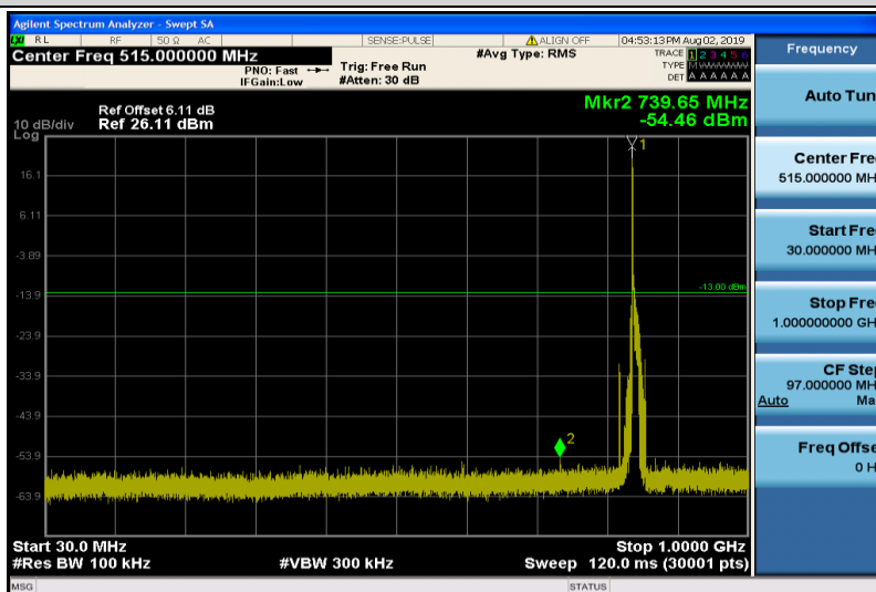
Band5-10MHz-16QAM-20600-1RB#0-30~1000MHz
