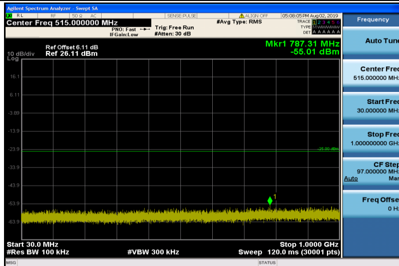
Band7-10MHz-QPSK-21400-1RB#0-30~1000MHz
