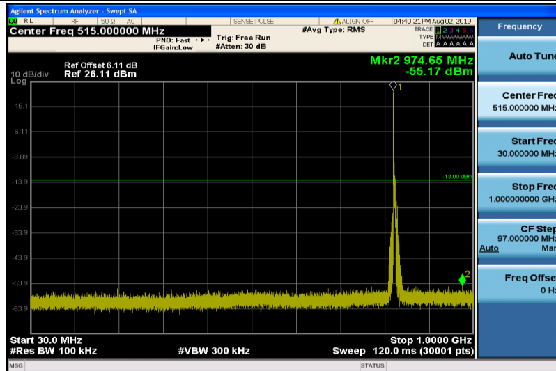
Band5-5MHz-16QAM-20425-1RB#0-30~1000MHz
