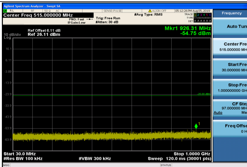
Band7-15MHz-QPSK-20825-1RB#0-30~1000MHz
