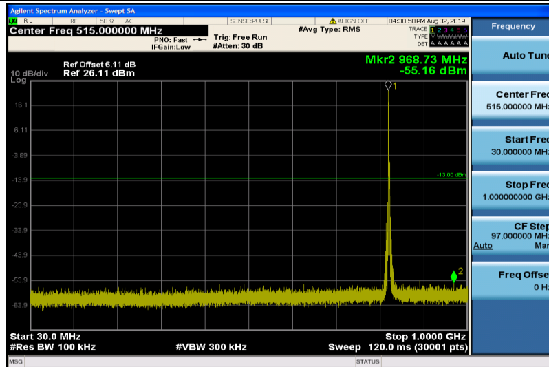
Band5-3MHz-16QAM-20415-1RB#0-30~1000MHz
