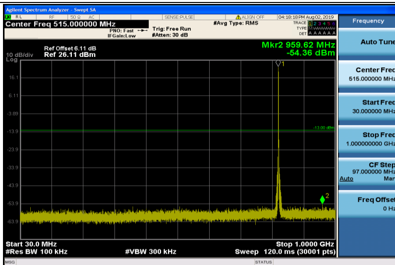
Band5-1.4MHz-QPSK-20407-1RB#0-30~1000MHz
