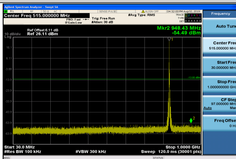
Band5-3MHz-16QAM-20525-1RB#0-30~1000MHz
