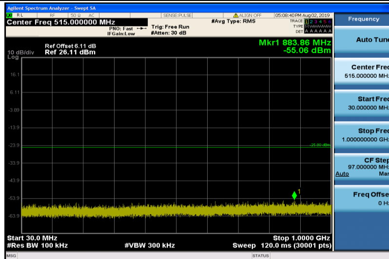
Band7-10MHz-16QAM-21400-1RB#0-30~1000MHz
