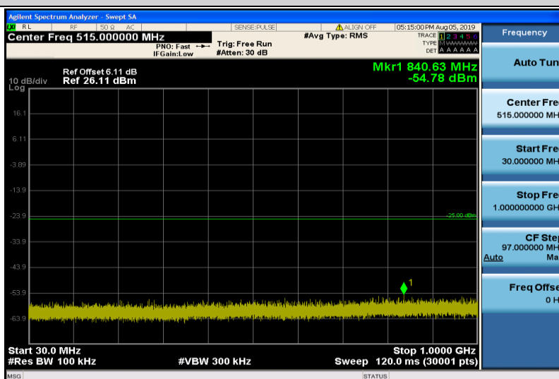
Band7-15MHz-QPSK-21100-1RB#0-30~1000MHz
