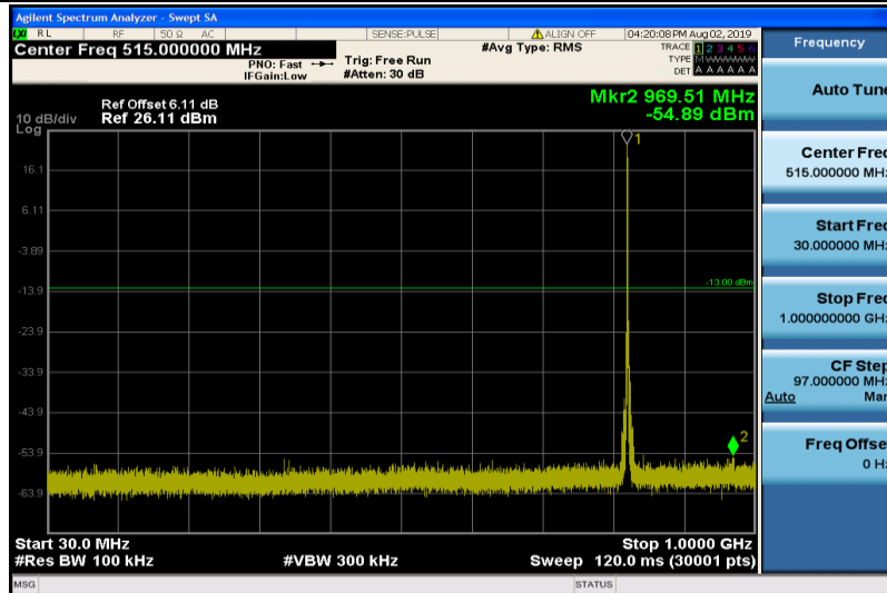
Band5-1.4MHz-16QAM-20407-1RB#0-30~1000MHz
