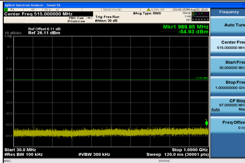
Band4-20MHz-16QAM-20300-1RB#0-30~1000MHz
