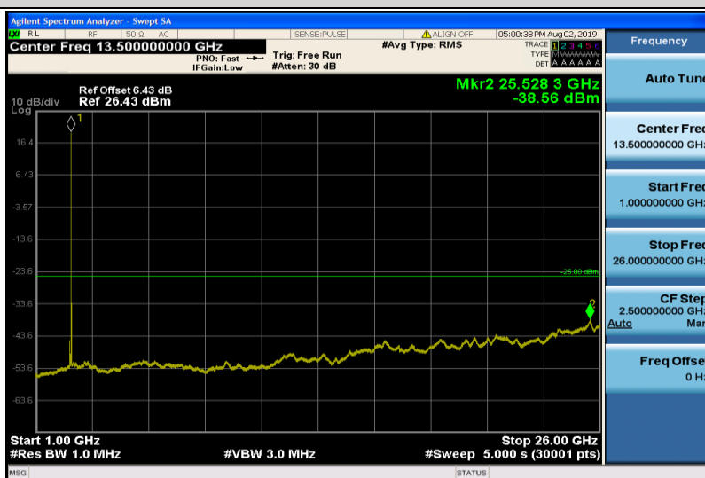
Band7-5MHz-QPSK-21425-1RB#0-1000~26000MHz
