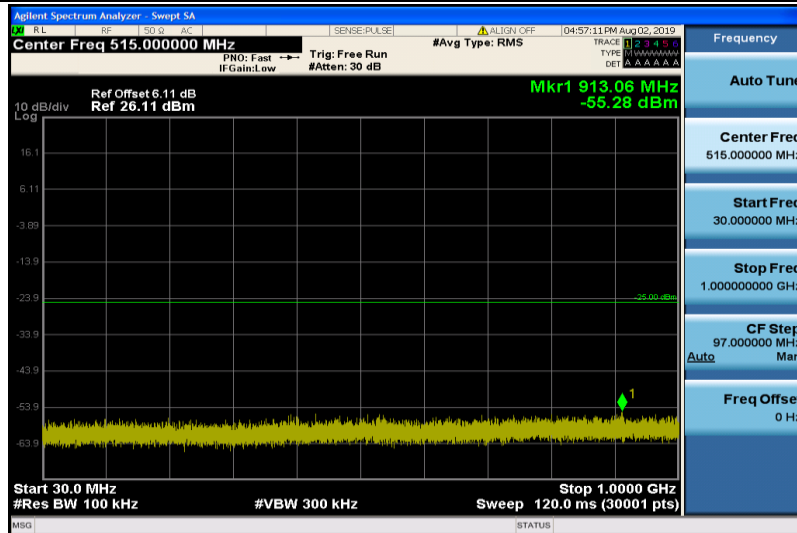
Band7-5MHz-QPSK-20775-1RB#0-30~1000MHz
