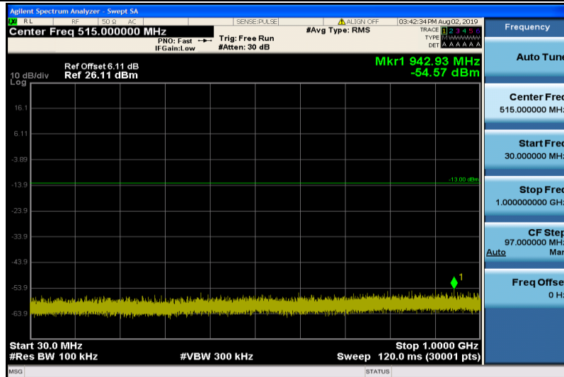
Band4-20MHz-16QAM-20050-1RB#0-30~1000MHz
