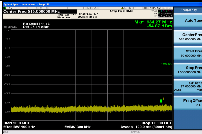
Band4-15MHz-16QAM-20325-1RB#0-30~1000MHz
