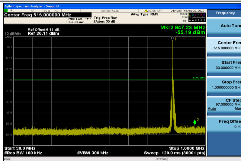
Band5-5MHz-QPSK-20525-1RB#0-30~1000MHz
