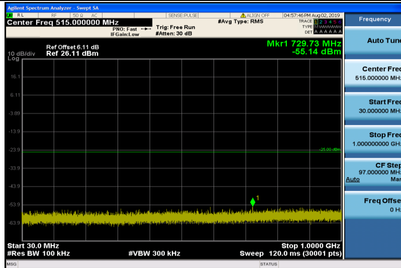
Band7-5MHz-16QAM-20775-1RB#0-30~1000MHz
