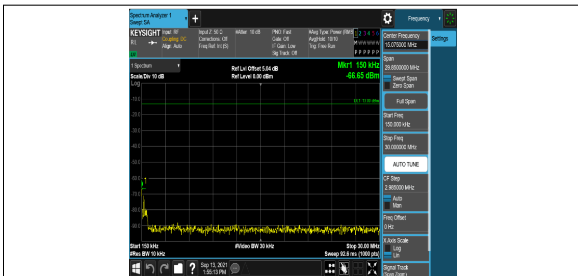
Band26-1.4MHz-16QAM-26915-1RB#0-Range2:0.15~30MHz
