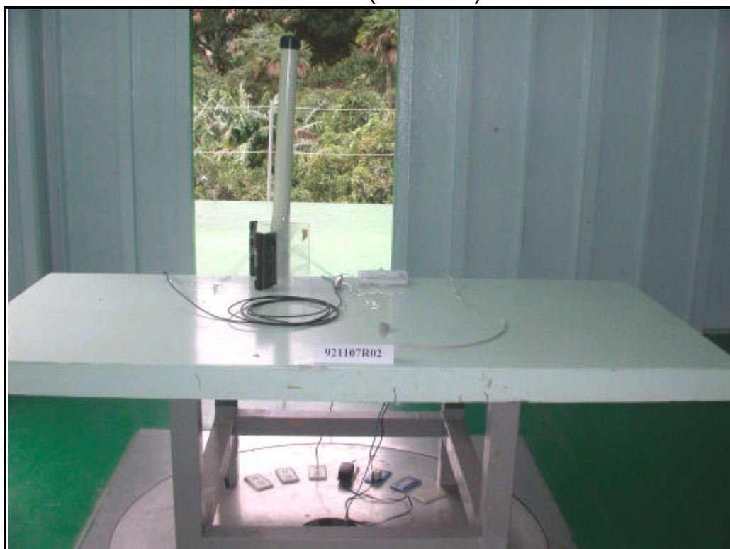
Antenna 8 (For 5 GHz)
