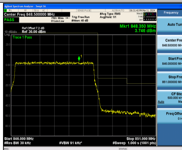
Band5 3MHz QPSK 20635 15RB#0
