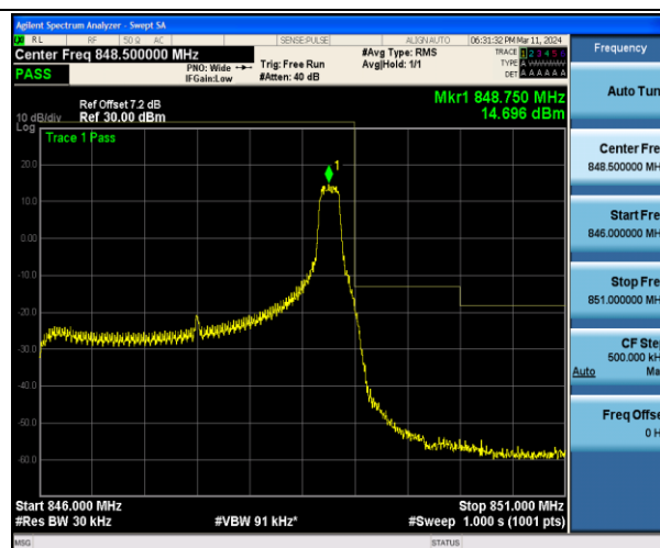
Band5 3MHz 16QAM 20635 1RB#14
