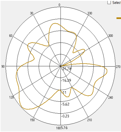
2D Antenna Pattern (X->Y;X->Z;Y->Z)
