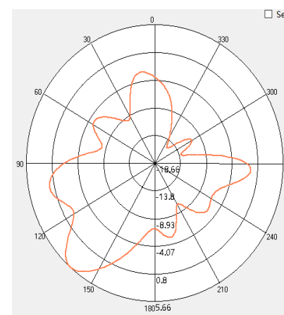
2D Antenna Pattern (X->Y; X->Z; Y->Z)
