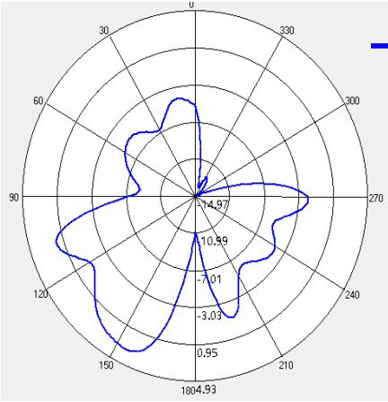
2D Antenna Pattern (X->Y;X->Z;Y->Z)
