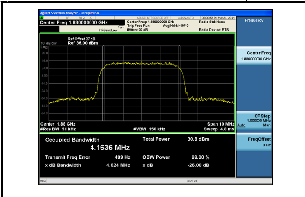
(Plot C1: HSPA+1900 MHz Channel = 9400)
