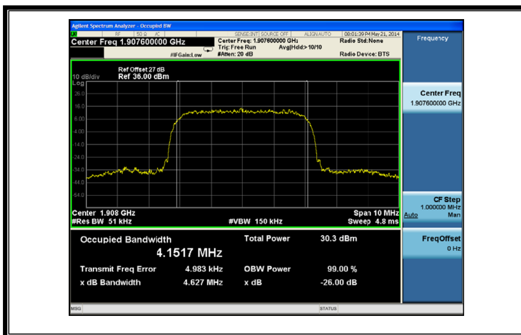
(Plot D1: HSPA+1900 MHz Channel = 9538)
