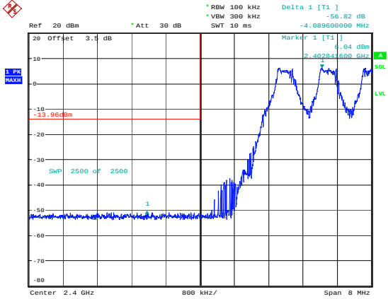
GFSK_Hopping_Lower 56.82dB
