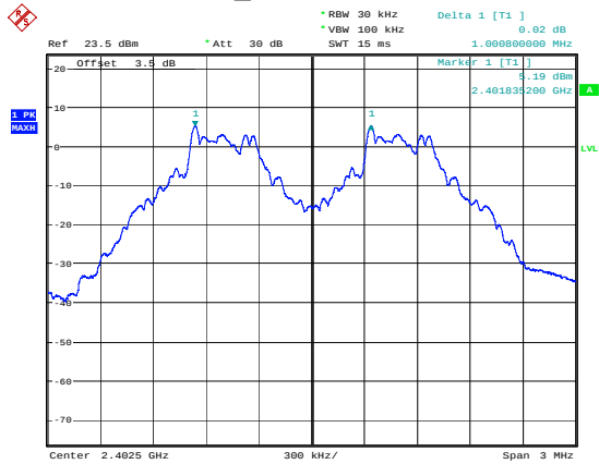
GFSK_Low 1.001MHz
