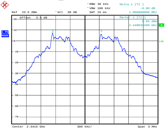
GFSK_Middle 1.001MHz
