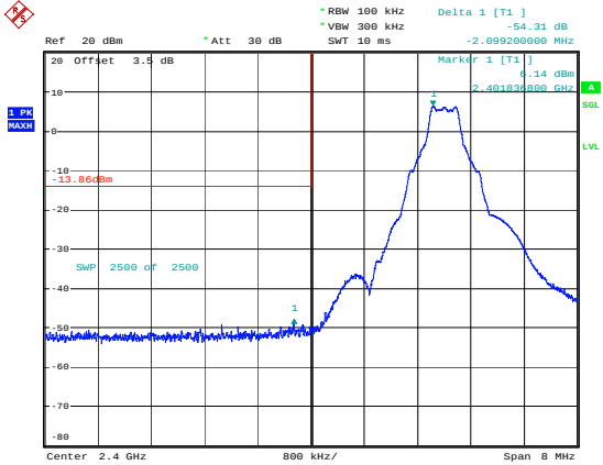
GFSK_Low 54.31dB
