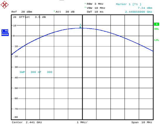
GFSK_Middle 7.24dBm
