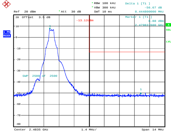
GFSK_High 56.67dB
