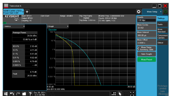
5G NR n77_CH656000_50M_1RB_16-QAM_Ratio
