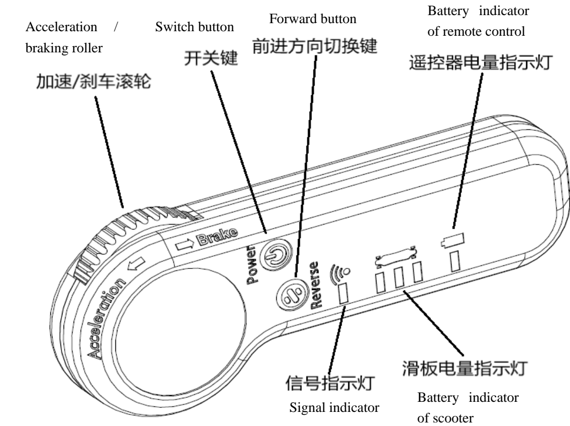
遥控器示意图 Diagram of remote control:
