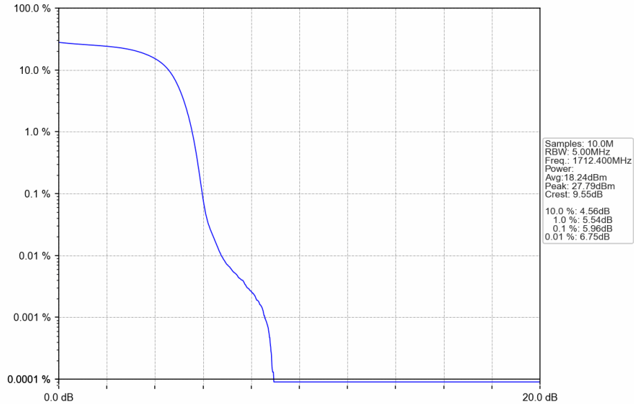
Band4_HSDPA_LCH_1712.4MHz_Subtest 1_NTNV
