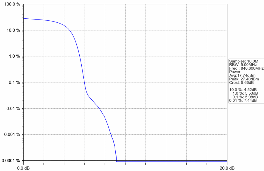
Band5_HSUPA_HCH_846.6MHz_Subtest 1_NTNV
