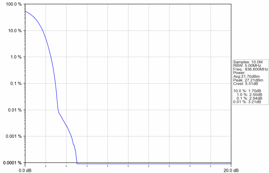
Band5_RMC_MCH_836.6MHz_12.2kbps RMC_NTNV
