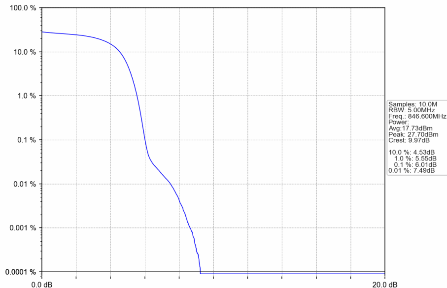
Band5_HSDPA_HCH_846.6MHz_Subtest 1_NTNV
