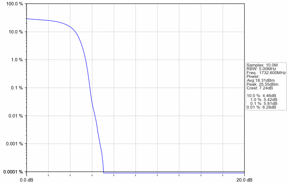
Band4_HSUPA_MCH_1732.6MHz_Subtest 1_NTNV
