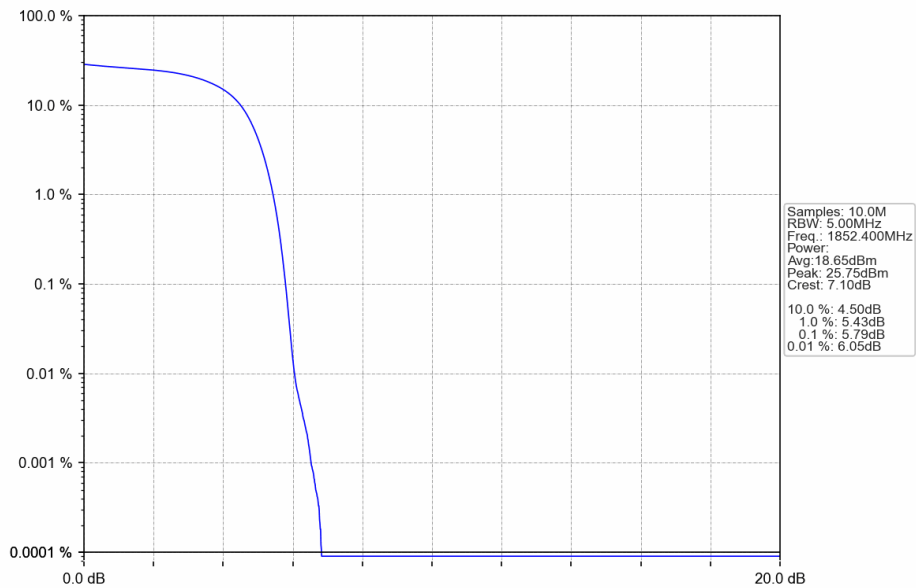
Band2_HSDPA_LCH_1852.4MHz_Subtest 1_NTNV
