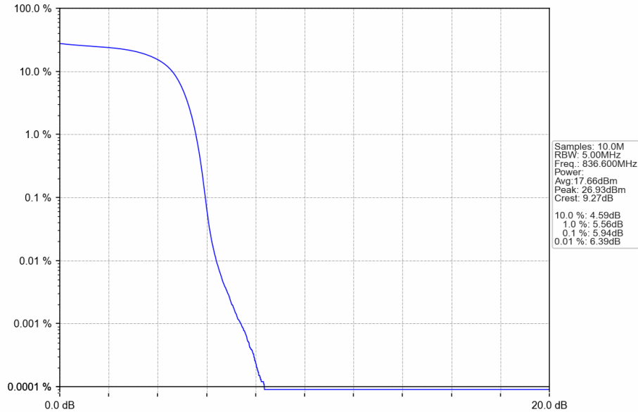
Band5_HSDPA_MCH_836.6MHz_Subtest 1_NTNV
