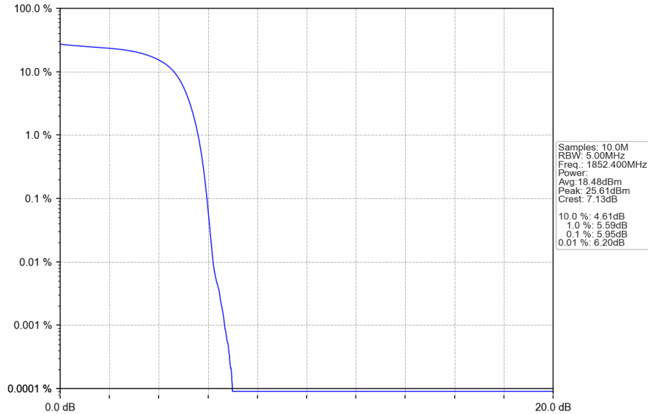
Band2_HSUPA_LCH_1852.4MHz_Subtest 1_NTNV
