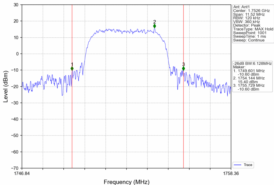
Band4_HSUPA_HCH_1752.6MHz_Subtest 1_NTNV
