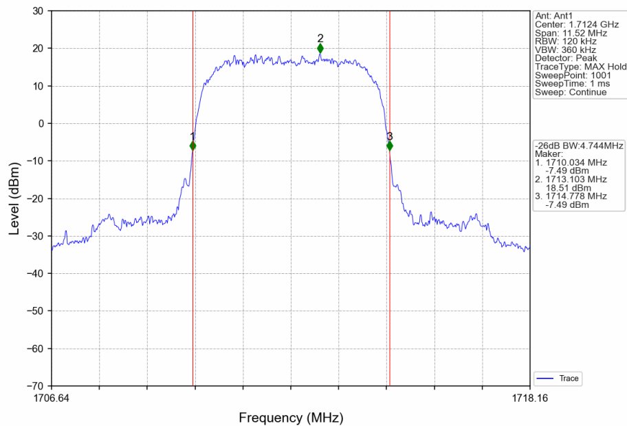
Band4_RMC_LCH_1712.4MHz_12.2kbps RMC_NTNV
