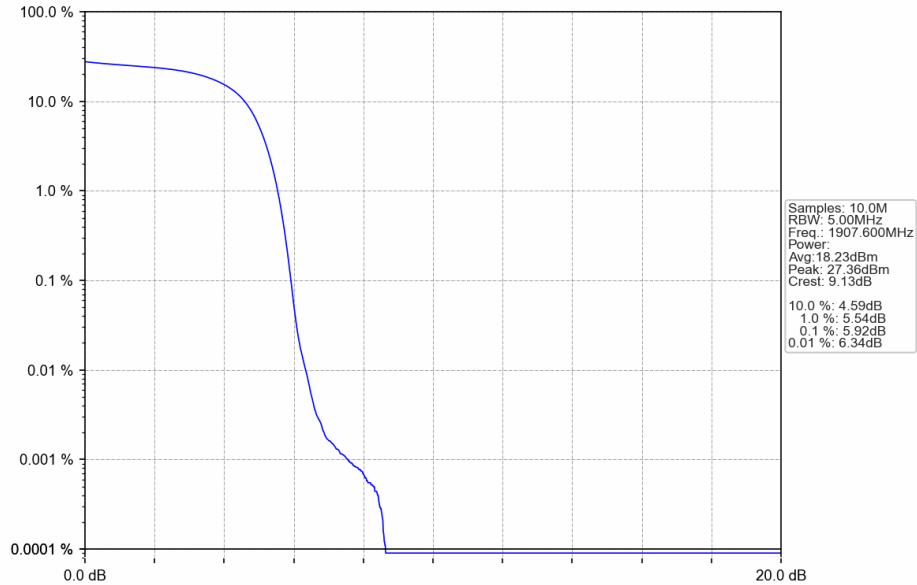
Band2_HSUPA_HCH_1907.6MHz_Subtest 1_NTNV
