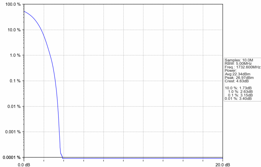
Band4_RMC_MCH_1732.6MHz_12.2kbps RMC_NTNV
