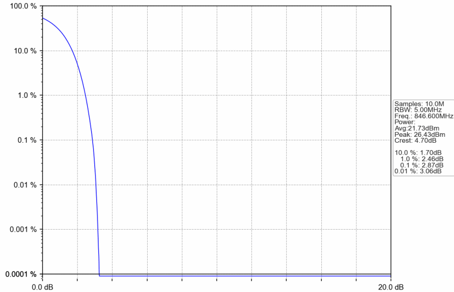
Band5_RMC_HCH_846.6MHz_12.2kbps RMC_NTNV
