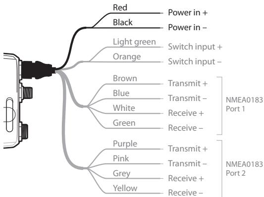
Figure 11 Connecting the power supply
