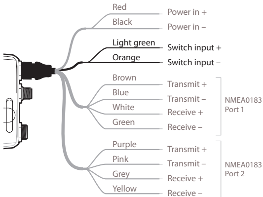
Figure 9 Connecting an external switch
