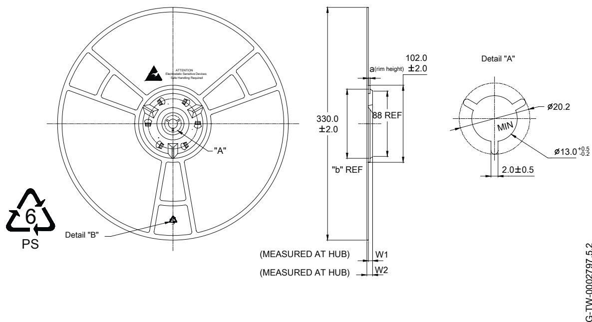
Figure 17.2: Reel Dimensions
