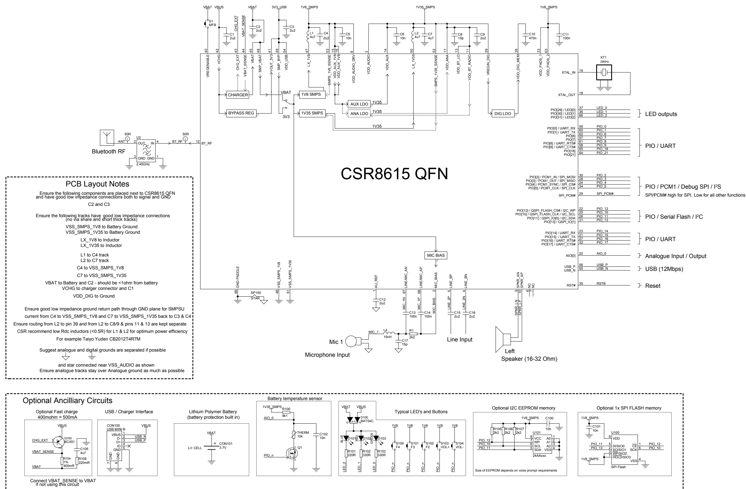
Figure 12.1: Single Microphone and Single Line Input
