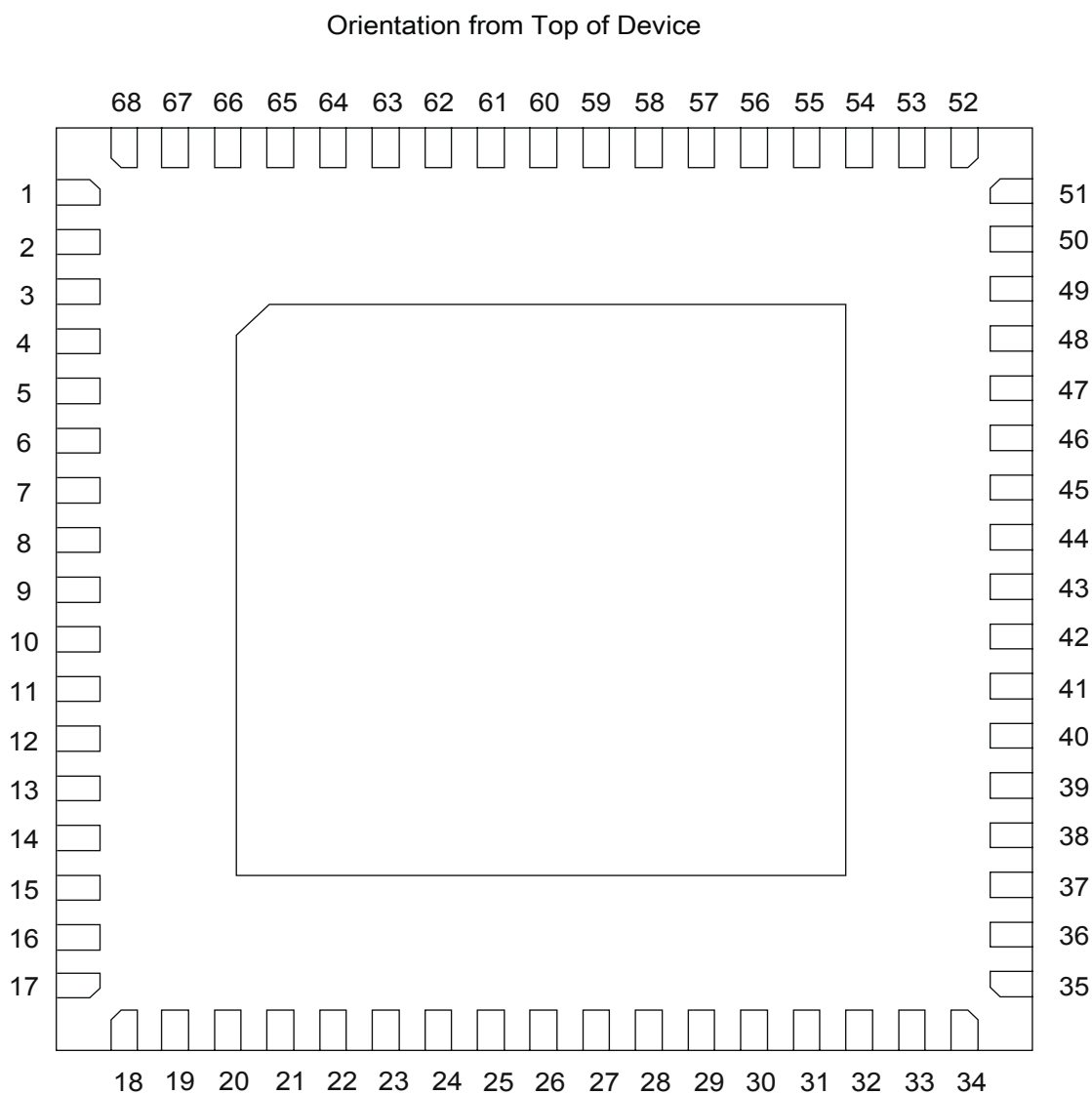
Figure 1.1: Device Pinout
