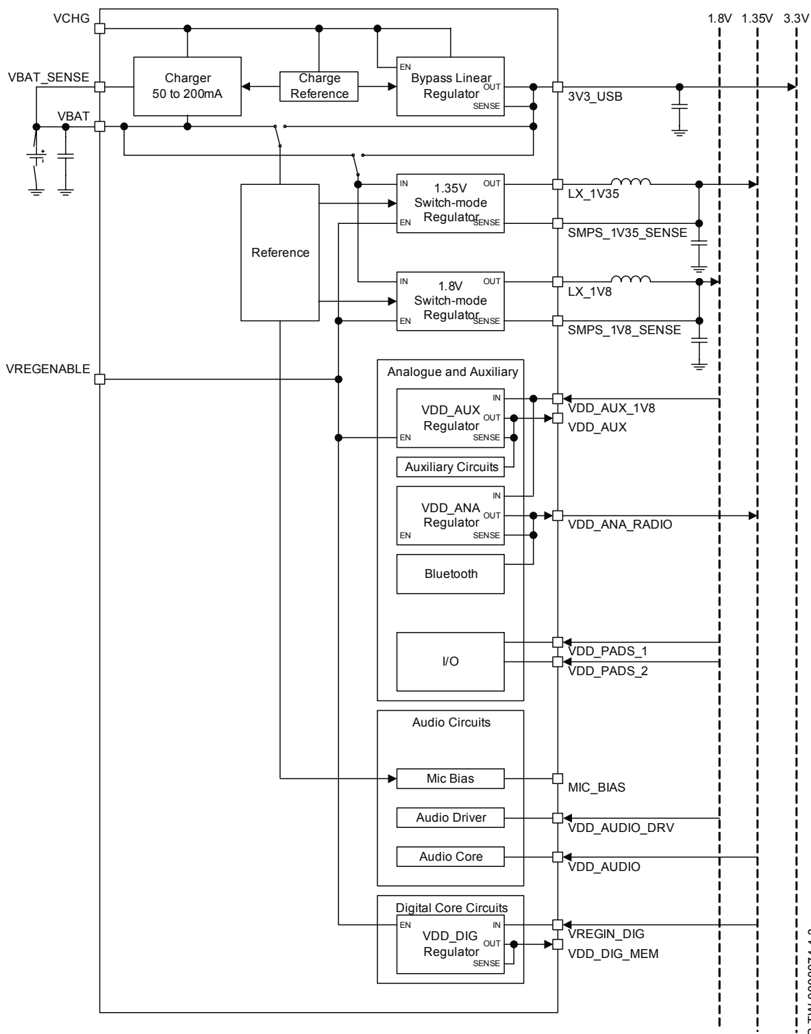
Figure 10.1: 1.80V and 1.35V Dual-supply Switch-mode System Configuration
