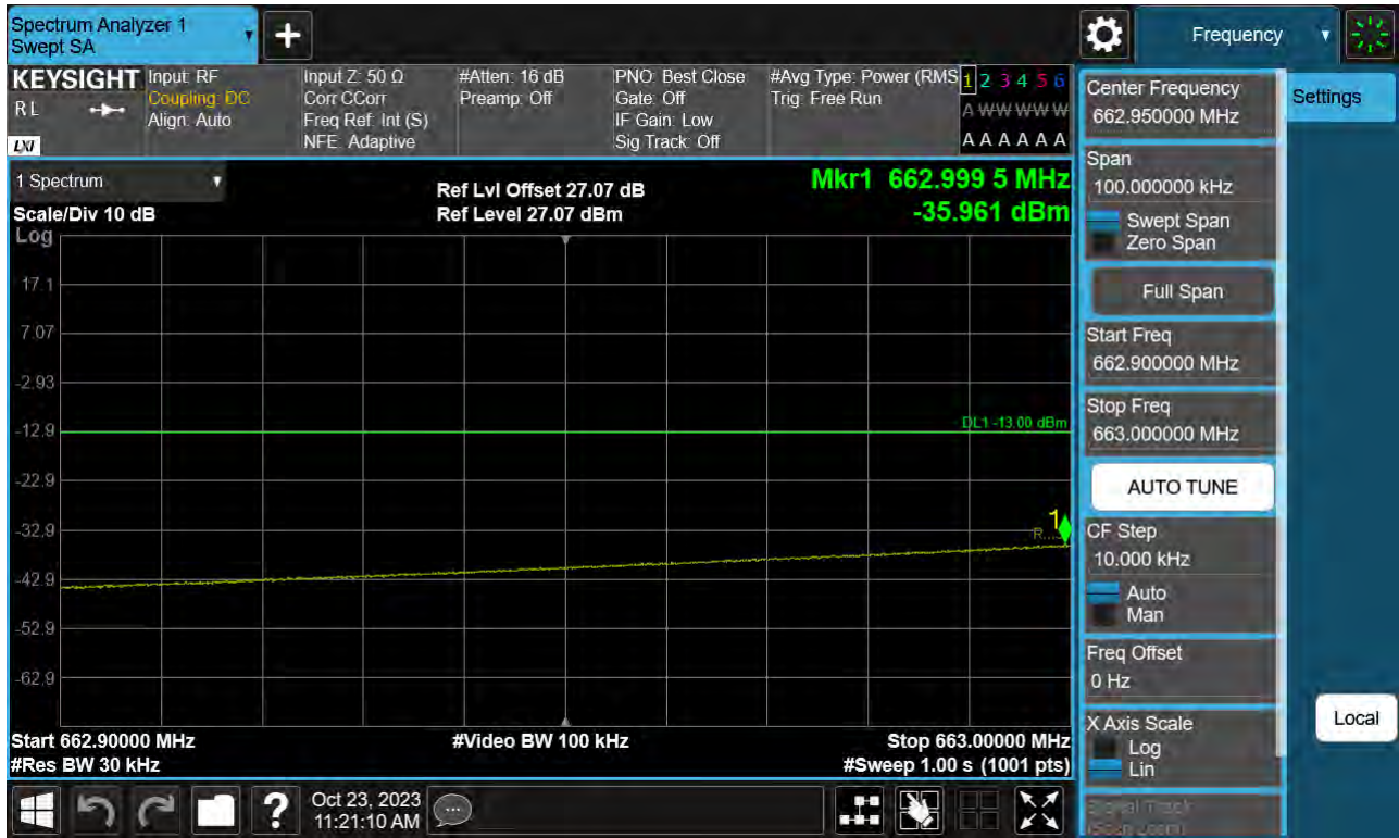
Sub6 n71. Lower Band Edge Plot (20 M BW Ch.134600 BPSK_RB1_Offset 0)_1
