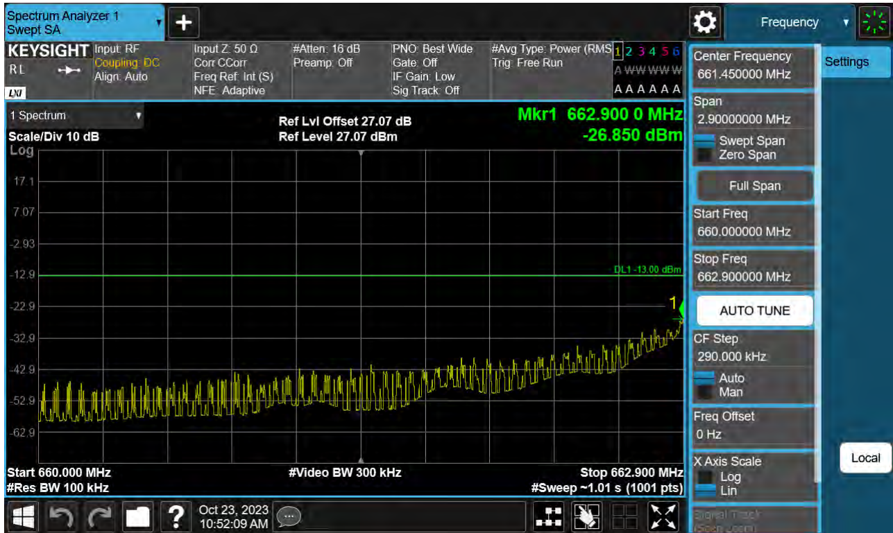
Sub6 n71. Lower Band Edge Plot (5 M BW Ch.133100 BPSK_RB1_Offset 0)_2
