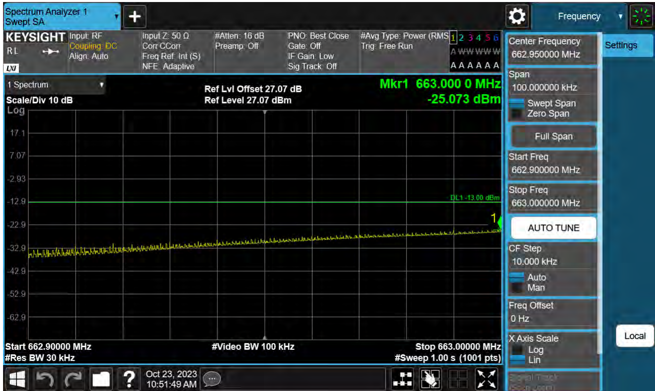
Sub6 n71. Lower Band Edge Plot (5 M BW Ch.133100 BPSK_RB1_Offset 0)_1
