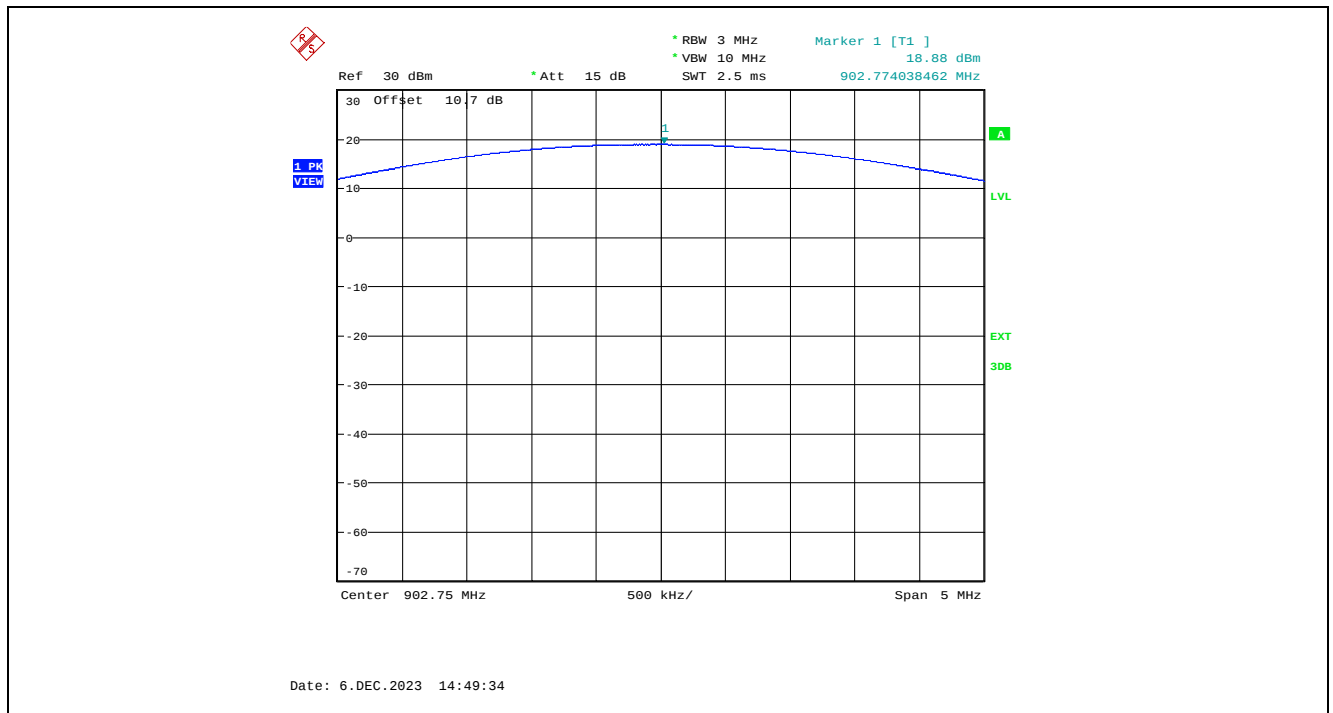
Plot 5.4.4.1.7. XB-9XR-DMUM-001 Maximum Peak Conducted Output Power, High Power Setting, 250 kbps, 902.75 MHz
