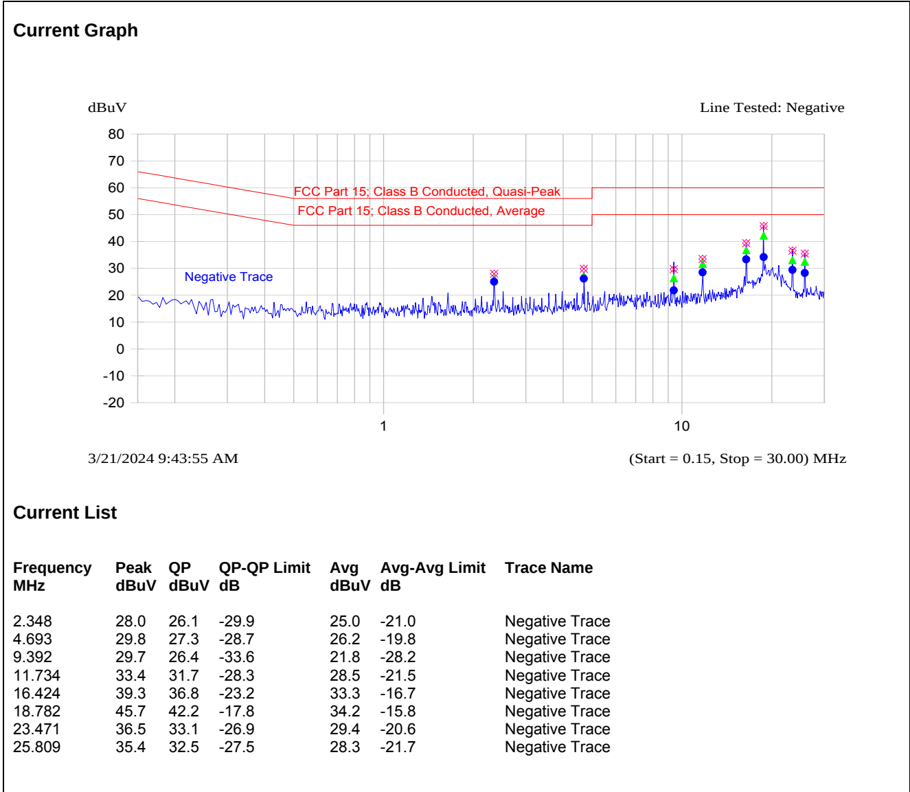
Plot 5.1.4.2. XB-9XR-DMUM-001 Power Line Conducted Emissions (Tx Mode) Line Voltage: 3.6 VDC; Line Tested: Negative
