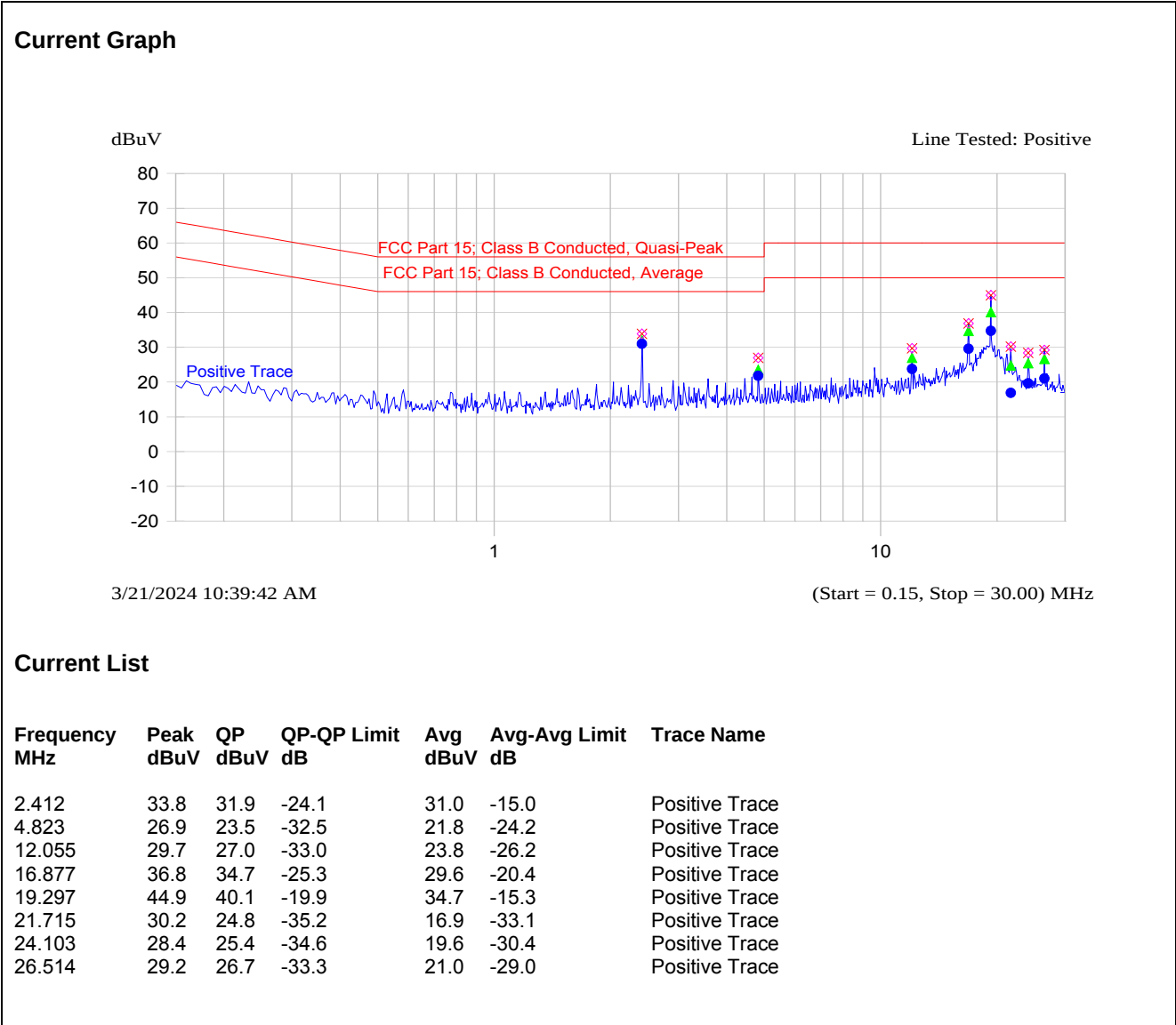
Plot 5.1.4.13. XB-9XR-DMST-001 Power Line Conducted Emissions (Tx Mode) Line Voltage: 3.6 VDC; Line Tested: Positive
