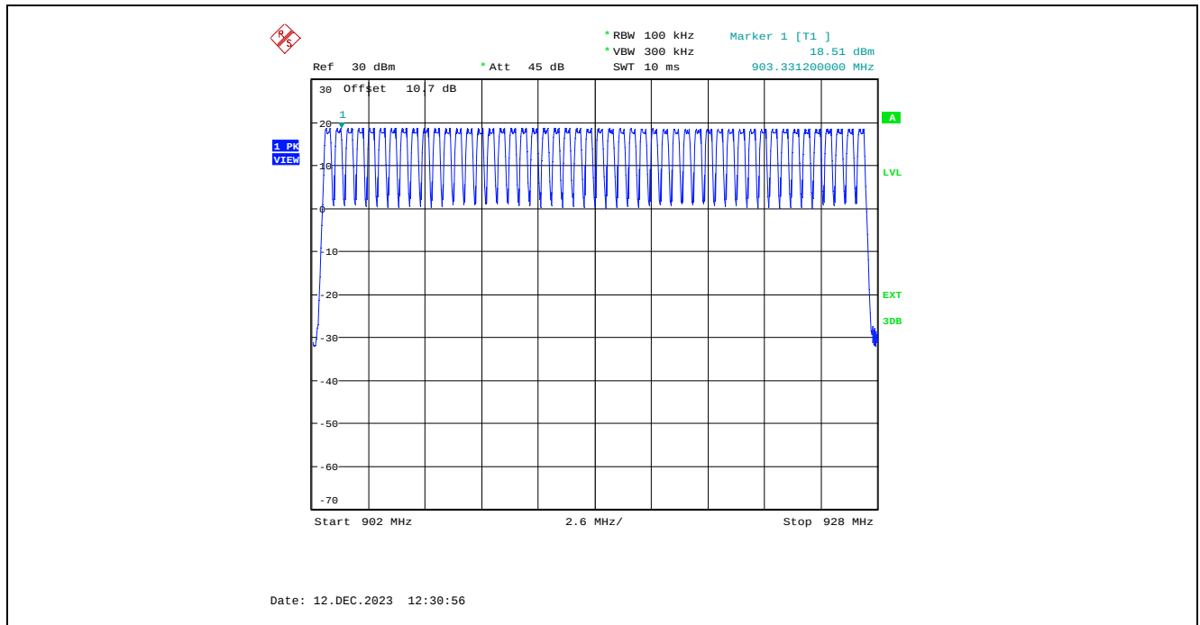
Plot 5.3.4.15. Number of Hopping Frequencies, 250 kbps 50 Hopping Channels
