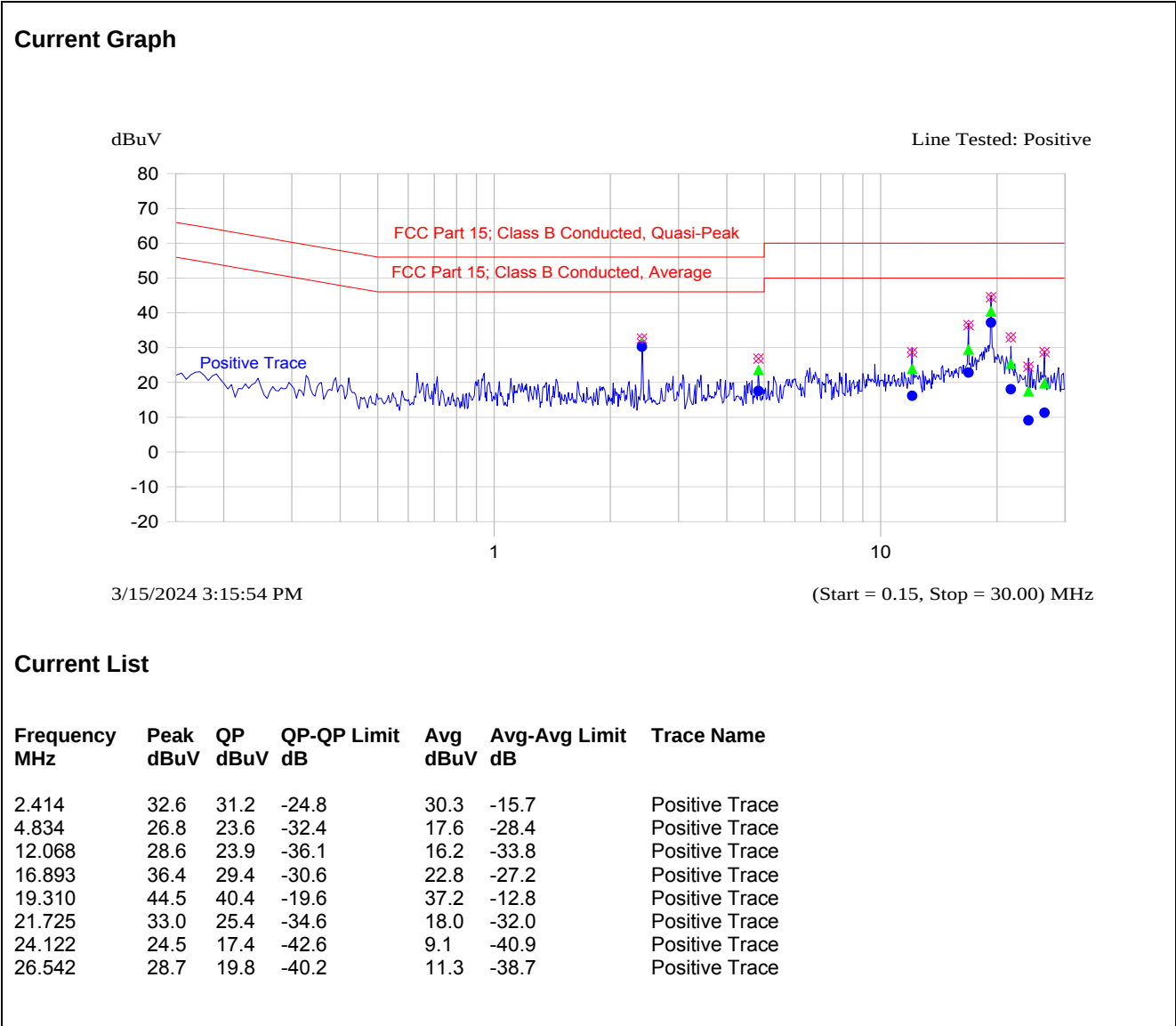
Plot 5.1.4.11. XB-9XR-DMUT-001 Power Line Conducted Emissions (Rx Mode) Line Voltage: 3.6 VDC; Line Tested: Positive
