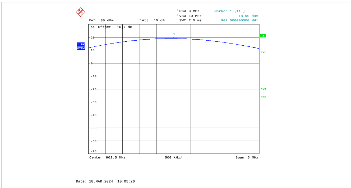
Plot 5.4.4.2.4. XB-9XR-DMUS-001 - Maximum Peak Conducted Output Power, High Power Setting, 110 kbps, 902.5 MHz
