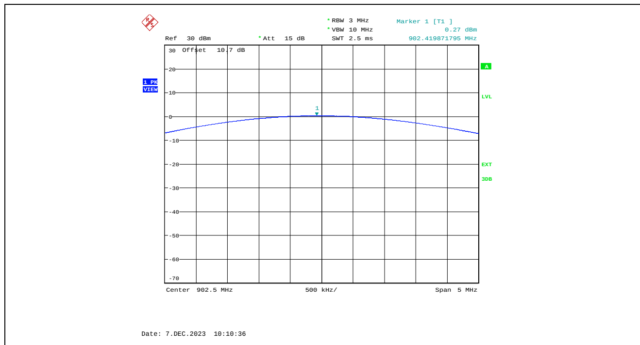
Plot 5.4.4.1.10. XB-9XR-DMUM-001 Maximum Peak Conducted Output Power, Low Power Setting, 10 kbps, 902.5 MHz
