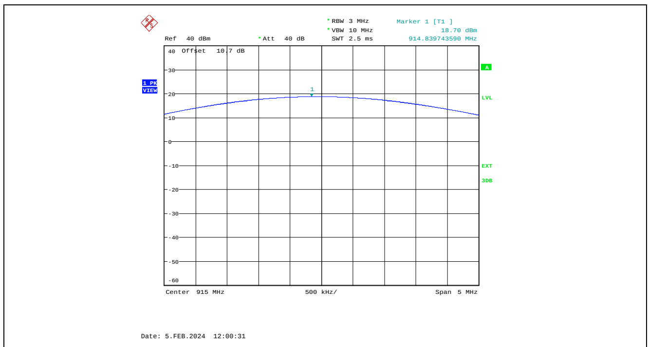
Plot 5.4.4.3.2. XB-9XR-DMUT-001 - Maximum Peak Conducted Output Power, High Power Setting, 10 kbps, 915 MHz
