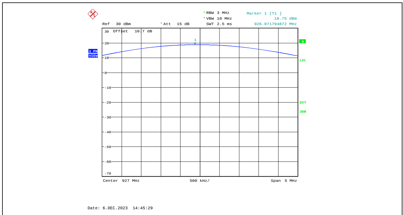
Plot 5.4.4.1.6. XB-9XR-DMUM-001 Maximum Peak Conducted Output Power, High Power Setting, 110 kbps, 927 MHz
