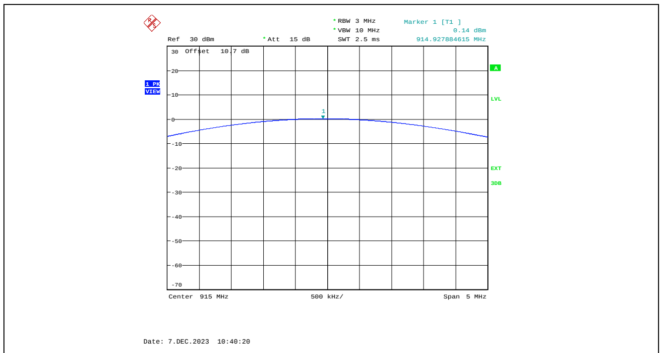
Plot 5.4.4.1.14. XB-9XR-DMUM-001 Maximum Peak Conducted Output Power, Low Power Setting, 110 kbps, 915 MHz
