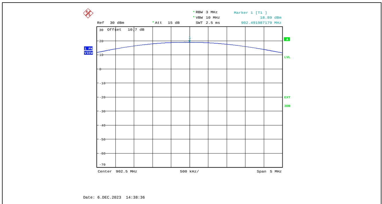
Plot 5.4.4.1.4. XB-9XR-DMUM-001 Maximum Peak Conducted Output Power, High Power Setting, 110 kbps, 902.5 MHz
