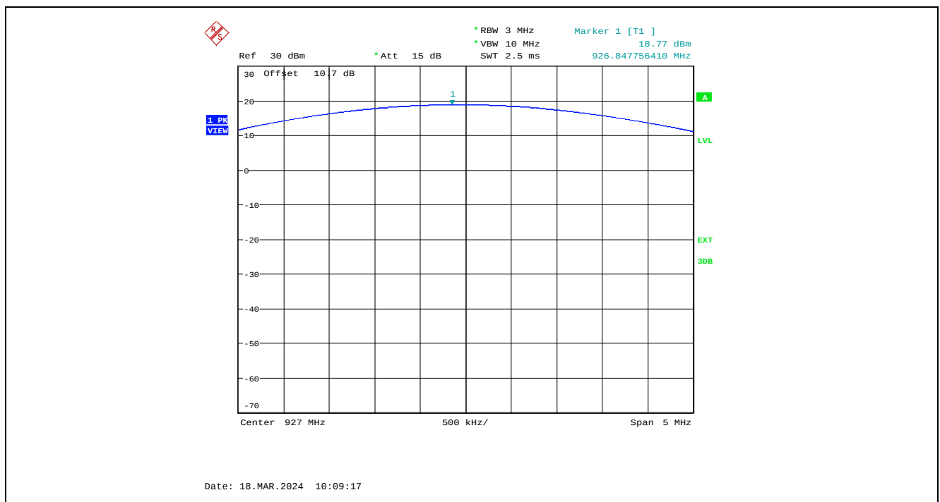
Plot 5.4.4.2.6. XB-9XR-DMUS-001 - Maximum Peak Conducted Output Power, High Power Setting, 110 kbps, 927 MHz
