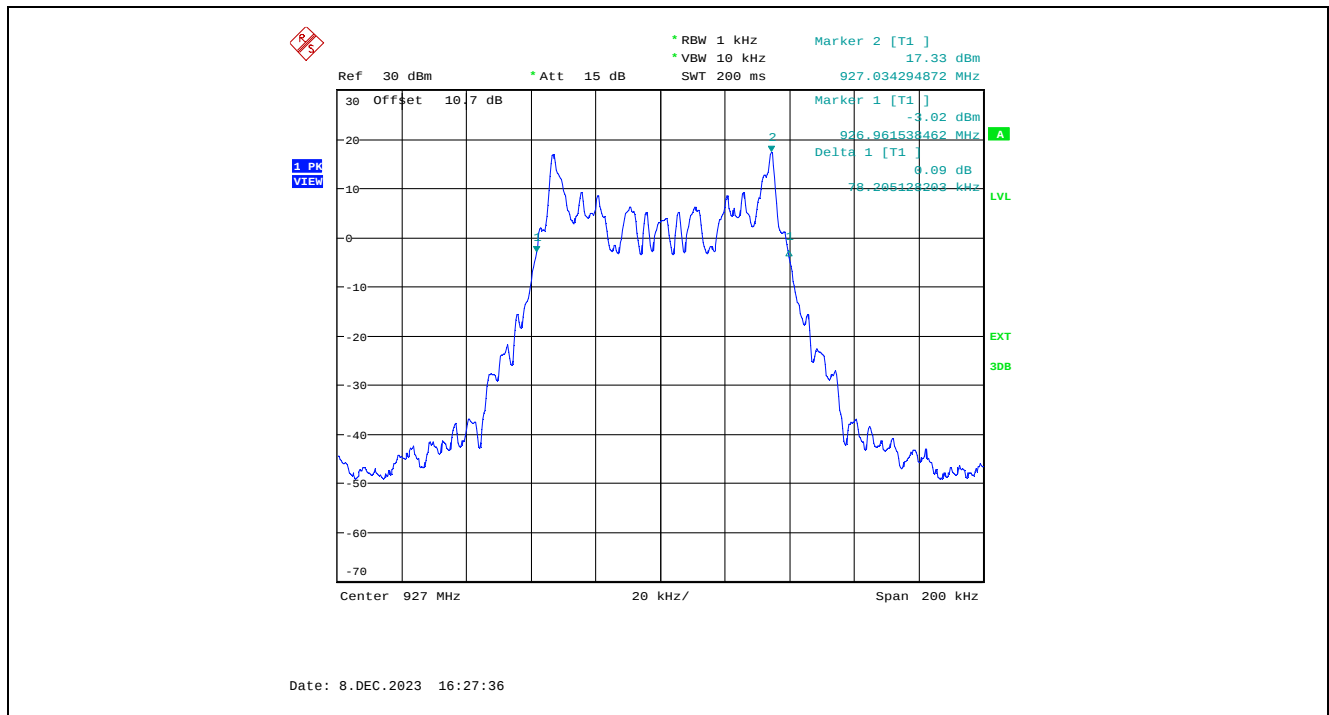
Plot 5.3.4.3. 20 dB Bandwidth, 927 MHz, MHz, 10 kbps
