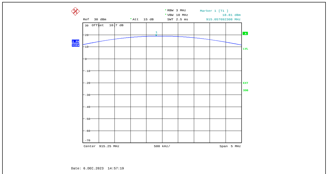
Plot 5.4.4.1.8. XB-9XR-DMUM-001 Maximum Peak Conducted Output Power, High Power Setting, 250 kbps, 915.25 MHz
