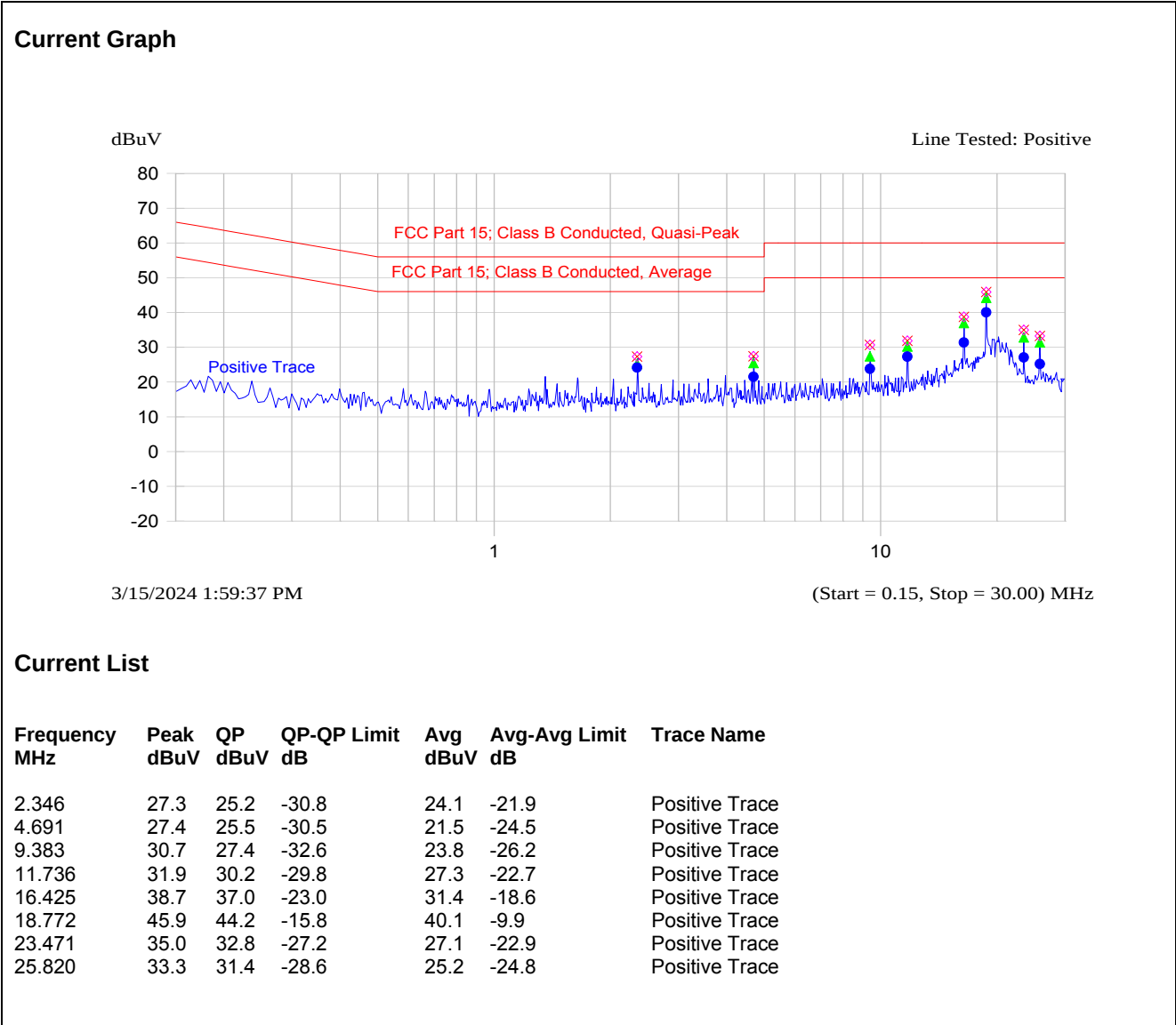
Plot 5.1.4.3. XB-9XR-DMUM-001 Power Line Conducted Emissions (Rx Mode) Line Voltage: 3.6 VDC; Line Tested: Positive
