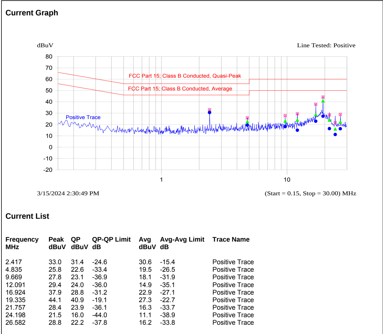
Plot 5.1.4.15. XB-9XR-DMST-001 Power Line Conducted Emissions (Rx Mode) Line Voltage: 3.6 VDC; Line Tested: Positive
