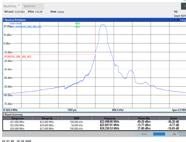
Band26-1.4MHz-QPSK-26797-6RB#0
