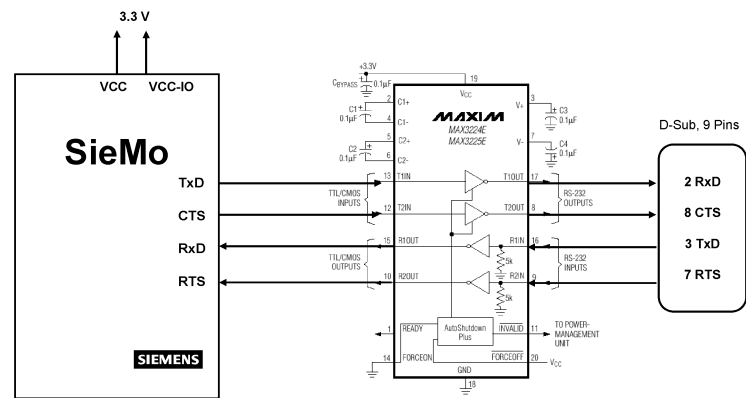
figure 16 Connection to PC via level converter
