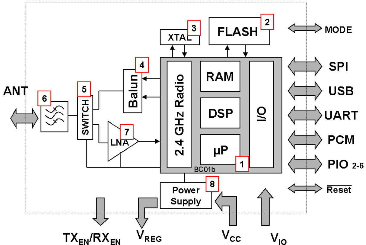
figure 25 block diagram
