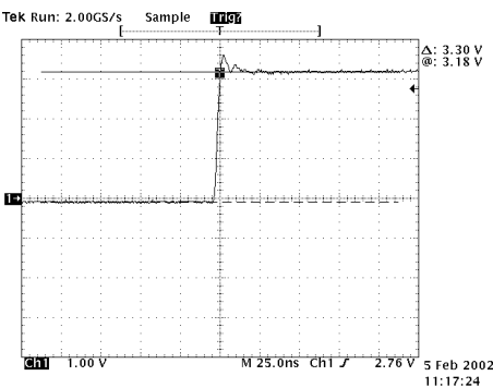
figure 17 UART TxD signal
