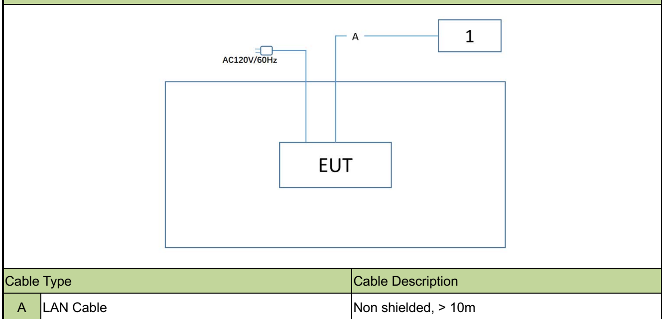
Connection Diagram – Radiated Emission & AC Conducted Emissions
