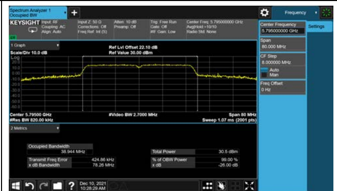
802.11ac-VHT80 26dB &amp; 99% Bandwidth
