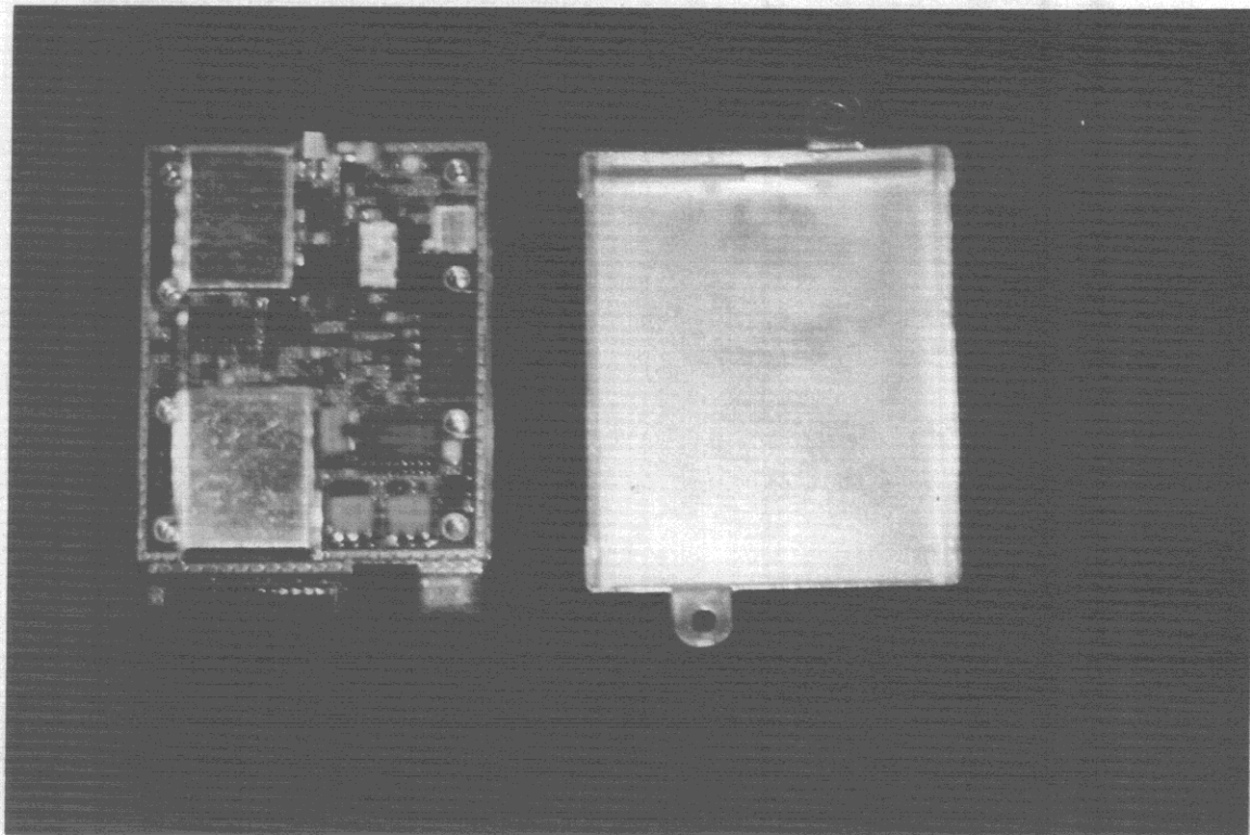
RF board with top shield cover:
