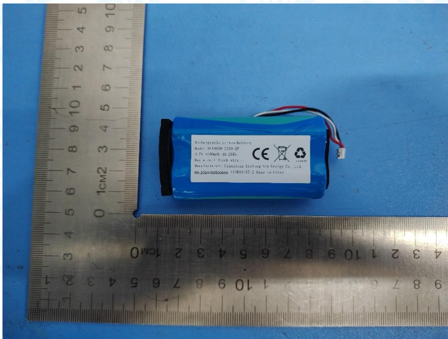
Photo 10 Battery appearance (INR18650)
