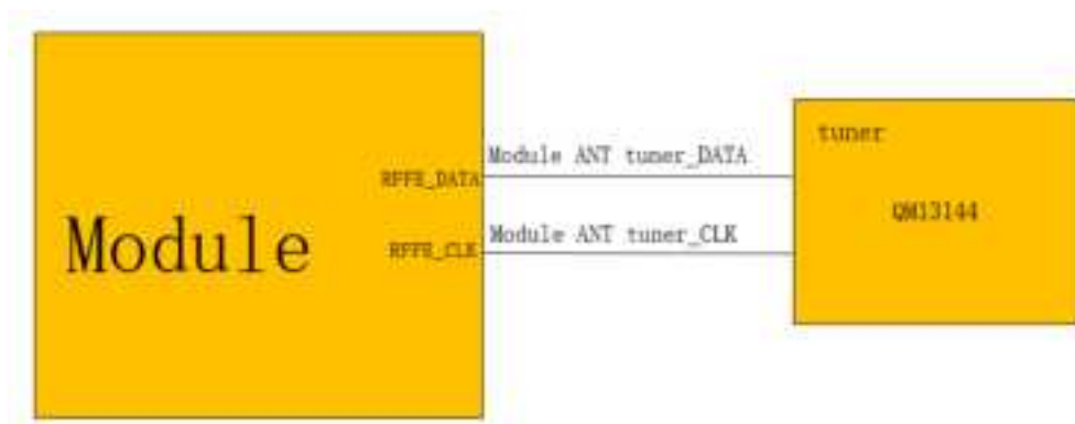
Figure 35: LGA package Tuner mipi interface
