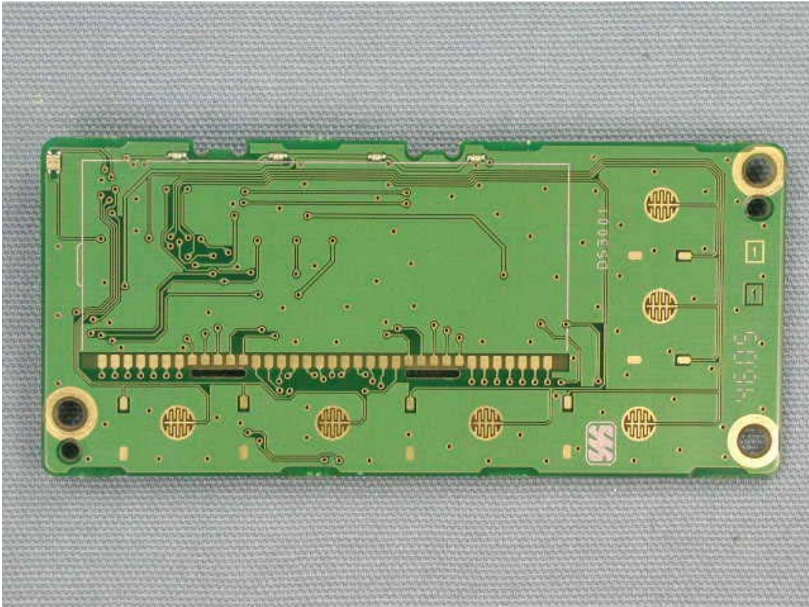
Side-A of FRONT-B-UNIT (for VX-2200) without LCD
