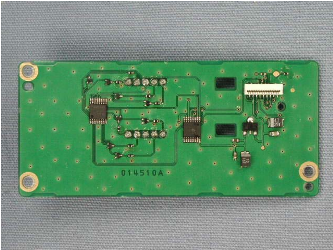
Side-B of FRONT-A-UNIT (for VX-2100)
