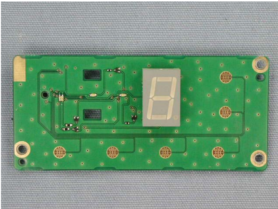
Side-A of FRONT-A-UNIT (for VX-2100)
