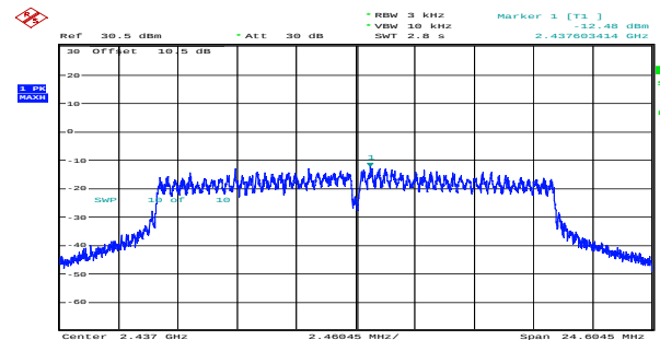
g_2437MHz_Chain 1 -12.48dBm/3kHz
