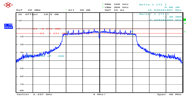
n20_2437MHz_Chain 1 15.635MHz
