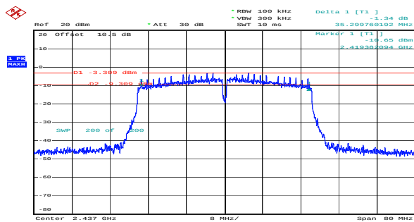
n40_2437MHz_Chain 0 35.300MHz
