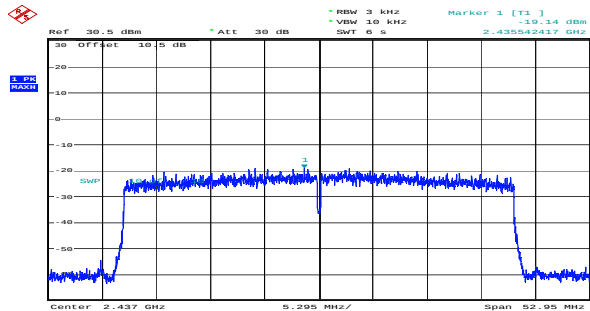
ax40_2437MHz_RU_Full_Chain 0 -19.14dBm/3kHz
