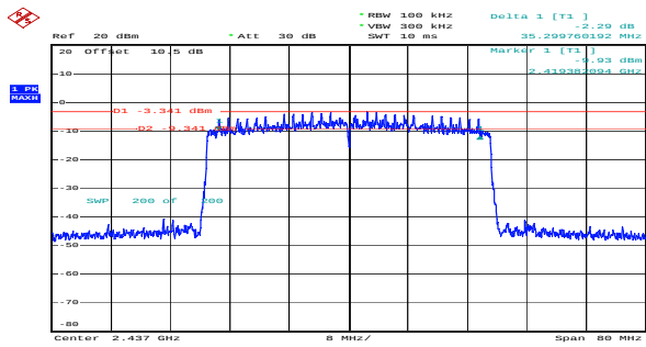
ax40_2437MHz_RU_Full_Chain 0 35.300MHz
