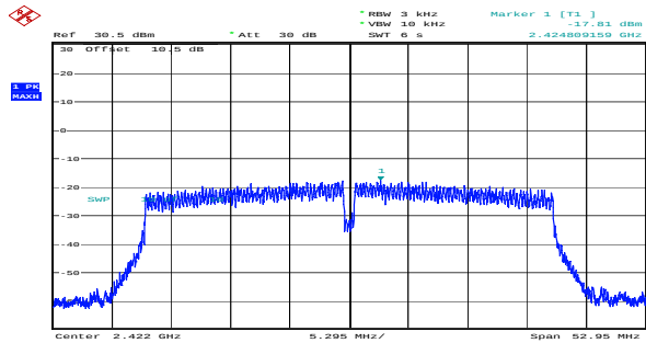
n40_2422MHz_Chain 0 -17.81dBm/3kHz
