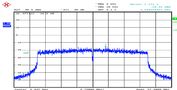
ax20_2437MHz_RU_Full_Chain 0 -16.31dBm/3kHz
