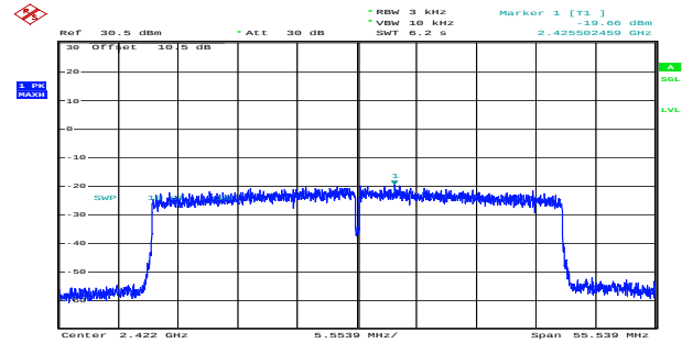
ax40_2422MHz_RU_Full_Chain 1 -19.66dBm/3kHz
