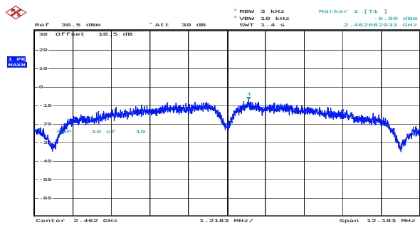
b_2462MHz_Chain 0 -6.90dBm/3kHz
