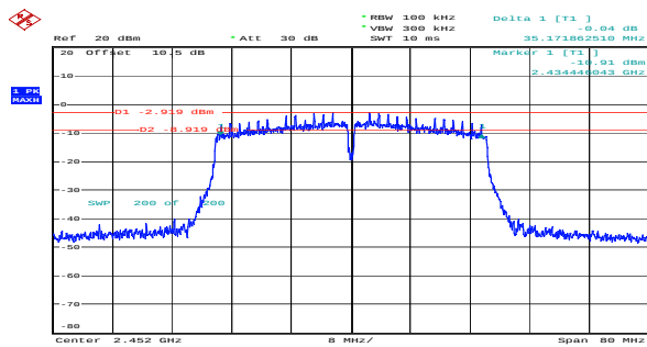
n40_2452MHz_Chain 0 35.172MHz
