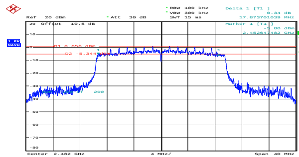
ax20_2462MHz_RU_Full_Chain 1 17.874MHz
