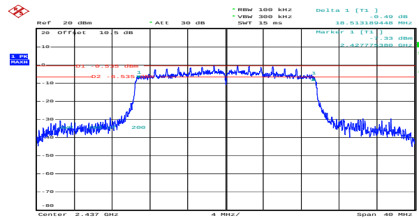
ax20_2437MHz_RU_Full_Chain 1 18.513MHz
