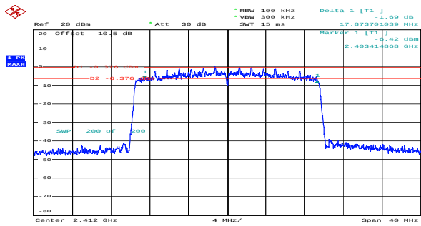
ax20_2412MHz_RU_Full_Chain 0 17.874MHz
