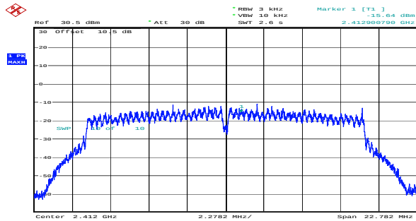
g_2412MHz_Chain 0 -15.64dBm/3kHz
