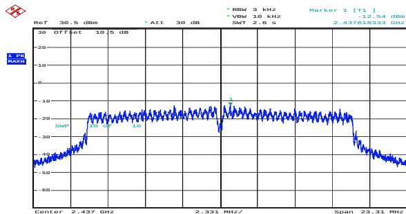
g_2437MHz_Chain 0 -12.54dBm/3kHz
