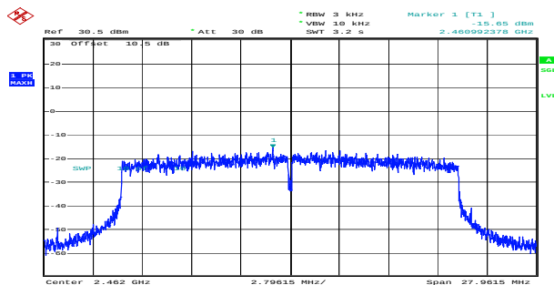
ax20_2462MHz_RU_Full_Chain 0 -15.65dBm/3kHz
