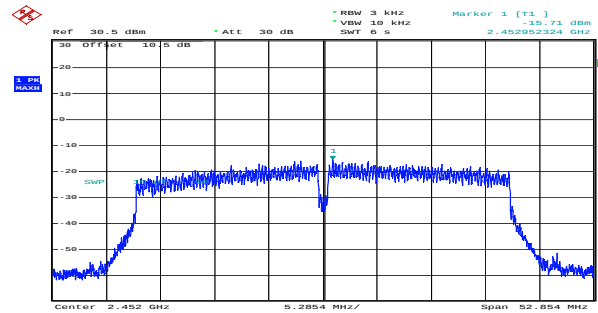
n40_2452MHz_Chain 1 -15.71dBm/3kHz
