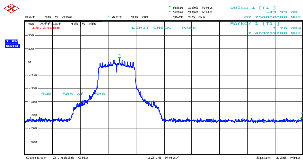
g_2462MHz_Chain 0 43.33dB
