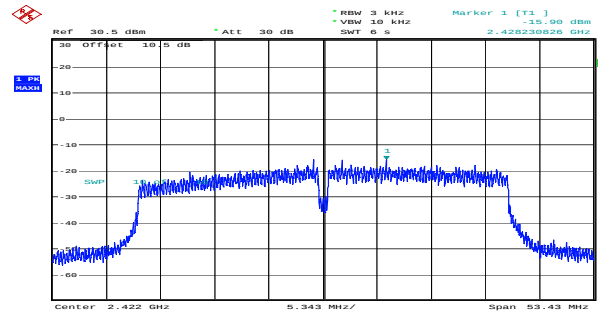
n40_2422MHz_Chain 1 -15.90dBm/3kHz
