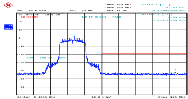
ax20_2462MHz_RU_Full_Chain 1 42.83dB
