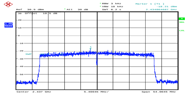
ax40_2437MHz_RU_Full_Chain 1 -18.21dBm/3kHz
