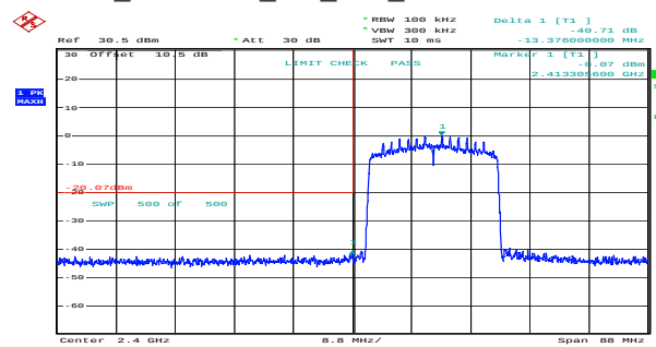
ax20_2412MHz_RU_Full_Chain 1 40.71dB
