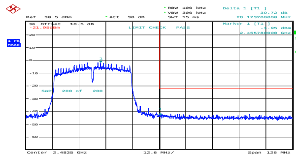
n40_2452MHz_Chain 1 39.72dB
