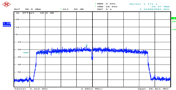
ax20_2412MHz_RU_Full_Chain 0 -16.37dBm/3kHz
