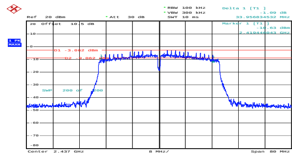
n40_2437MHz_Chain 1 33.957MHz
