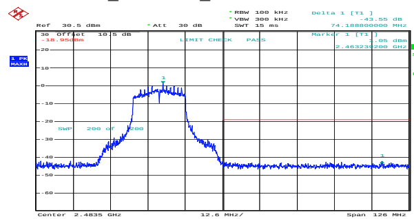
n20_2462MHz_Chain 1 43.55dB
