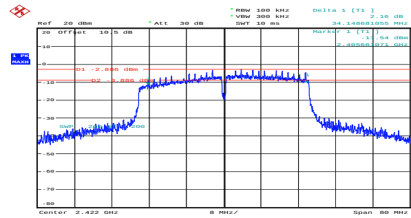
n40_2422MHz_Chain 1 34.149MHz
