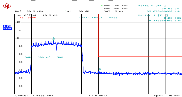
ax40_2452MHz_RU_Full_Chain 0 38.63dB
