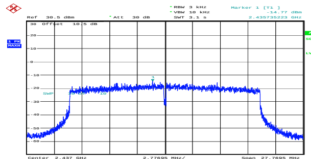
ax20_2437MHz_RU_Full_Chain 1 -14.77dBm/3kHz
