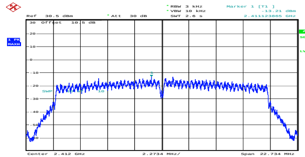
n20_2412MHz_Chain 1 -13.21dBm/3kHz
