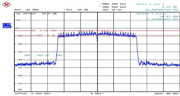
ax40_2452MHz_RU_Full_Chain 0 36.898MHz
