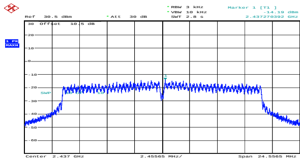
n20_2437MHz_Chain 0 -14.19dBm/3kHz
