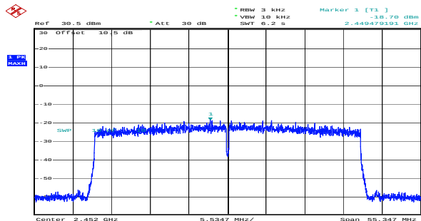
ax40_2452MHz_RU_Full_Chain 0 -18.70dBm/3kHz
