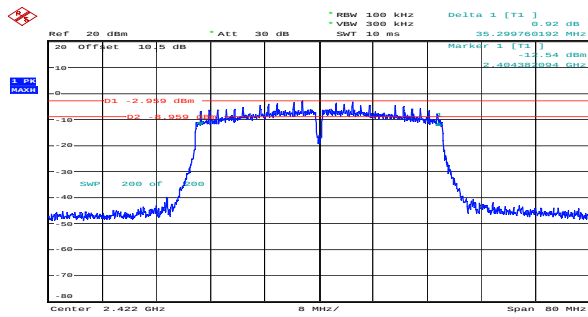
n40_2422MHz_Chain 0 35.300MHz
