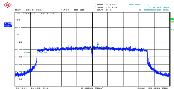
ax20_2462MHz_RU_Full_Chain 1 -14.45dBm/3kHz
