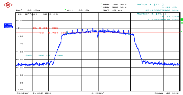
n20_2412MHz_Chain 1 15.156MHz
