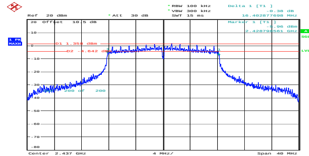
g_2437MHz_Chain 1 16.403MHz
