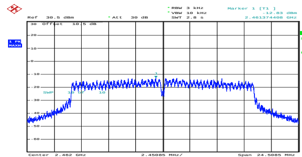
g_2462MHz_Chain 1 -12.83dBm/3kHz
