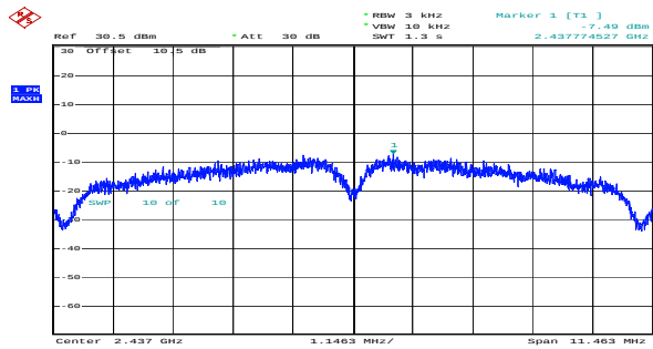
b_2437MHz_Chain 0 -7.49dBm/3kHz
