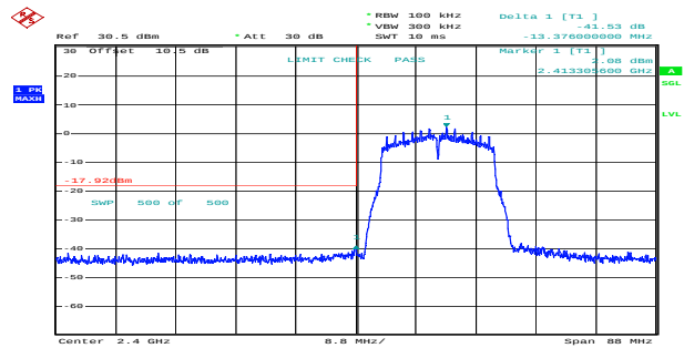
g_2412MHz_Chain 1 41.53dB
