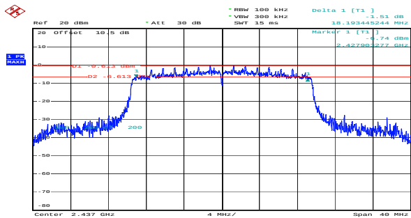
ax20_2437MHz_RU_Full_Chain 0 18.193MHz
