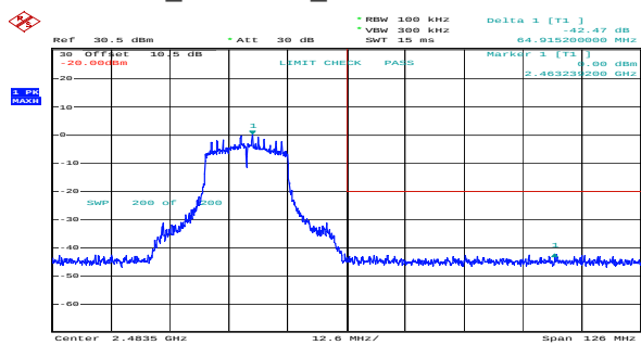
n20_2462MHz_Chain 0 42.47dB
