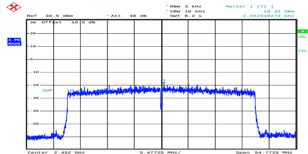
ax40_2452MHz_RU_Full_Chain 1 -19.33dBm/3kHz
