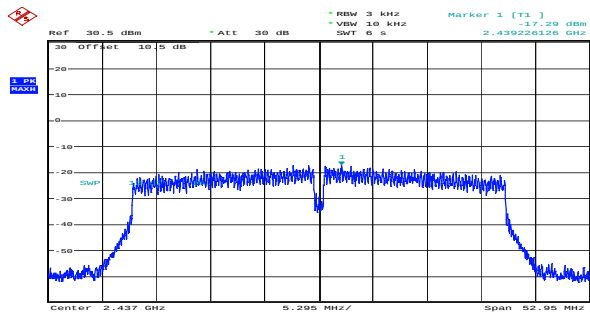
n40_2437MHz_Chain 0 -17.29dBm/3kHz
