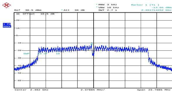
g_2462MHz_Chain 0 -13.05dBm/3kHz
