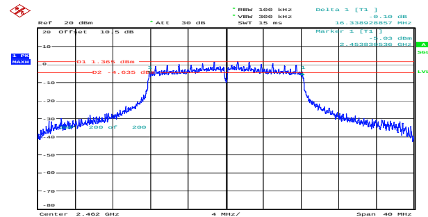
g_2462MHz_Chain 1 16.339MHz
