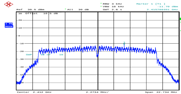
g_2412MHz_Chain 1 -11.70dBm/3kHz
