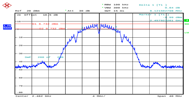
b_2462MHz_Chain 0 8.122MHz
