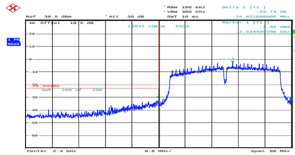
n40_2422MHz_Chain 1 29.73dB
