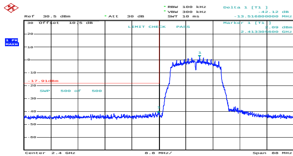
g_2412MHz_Chain 0 42.12dB
