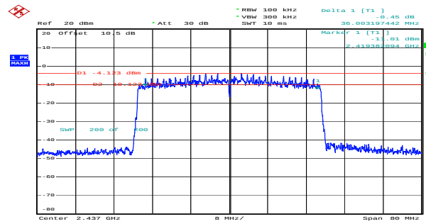
ax40_2437MHz_RU_Full_Chain 1 36.003MHz
