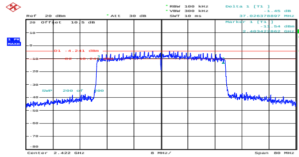
ax40_2422MHz_RU_Full_Chain 1 37.026MHz
