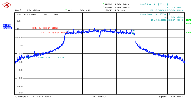
g_2462MHz_Chain 0 15.859MHz
