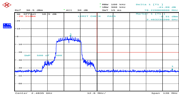
ax20_2462MHz_RU_Full_Chain 0 41.09dB
