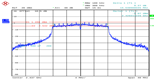
g_2437MHz_Chain 0 15.540MHz
