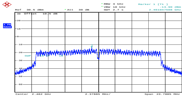
n20_2462MHz_Chain 0 -13.90dBm/3kHz
