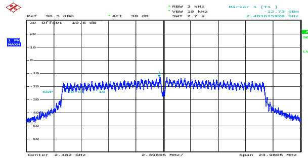
n20_2462MHz_Chain 1 -12.73dBm/3kHz
