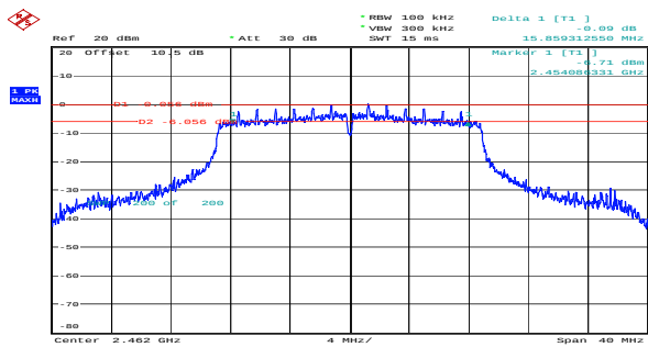
n20_2462MHz_Chain 0 15.859MHz
