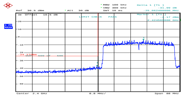
ax40_2422MHz_RU_Full_Chain 1 31.99dB
