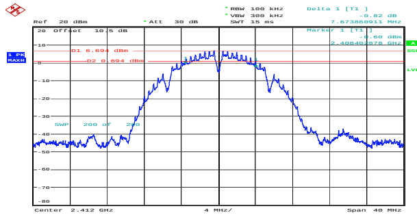
b_2412MHz_Chain 0 7.674MHz
