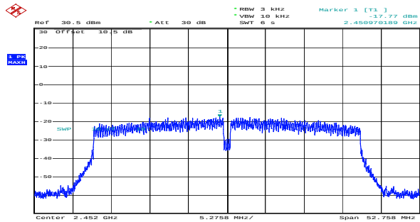
n40_2452MHz_Chain 0 -17.77dBm/3kHz
