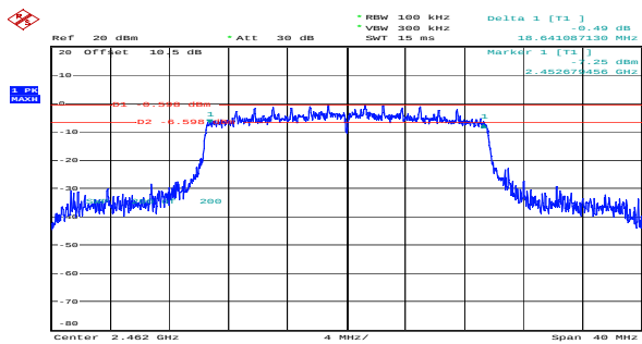
ax20_2462MHz_RU_Full_Chain 0 18.641MHz
