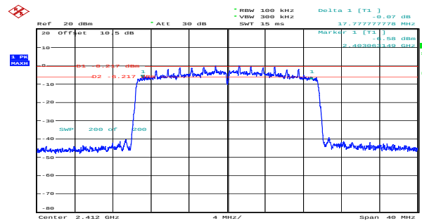
ax20_2412MHz_RU_Full_Chain 1 17.778MHz
