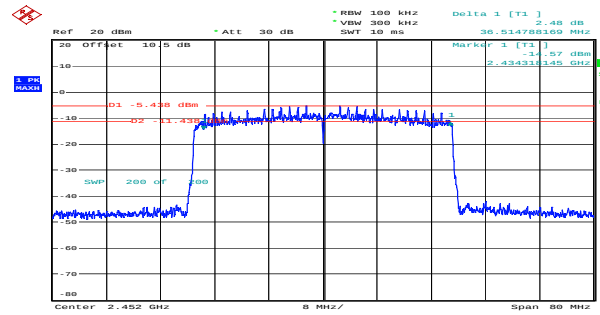
ax40_2452MHz_RU_Full_Chain 1 36.515MHz
