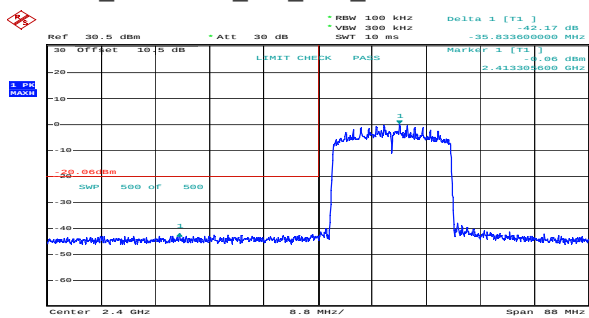
ax20_2412MHz_RU_Full_Chain 0 42.17dB
