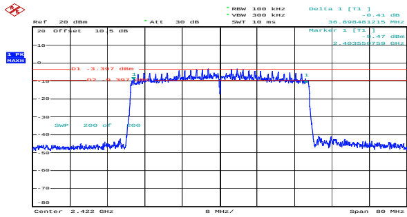
ax40_2422MHz_RU_Full_Chain 0 36.898MHz
