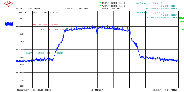
g_2412MHz_Chain 1 15.156MHz
