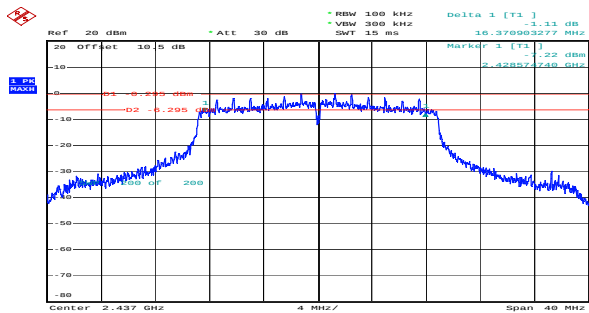
n20_2437MHz_Chain 0 16.371MHz
