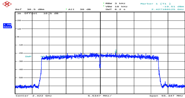
ax40_2422MHz_RU_Full_Chain 0 -19.51dBm/3kHz
