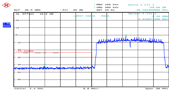
ax40_2422MHz_RU_Full_Chain 0 38.60dB
