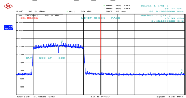
ax40_2452MHz_RU_Full_Chain 1 36.71dB
