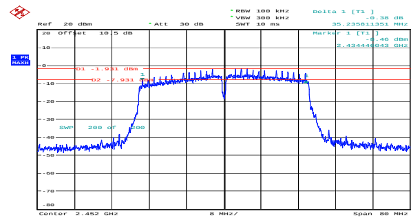
n40_2452MHz_Chain 1 35.236MHz
