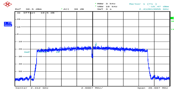
ax20_2412MHz_RU_Full_Chain 1 -15.47dBm/3kHz
