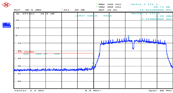
n40_2422MHz_Chain 0 36.71dB
