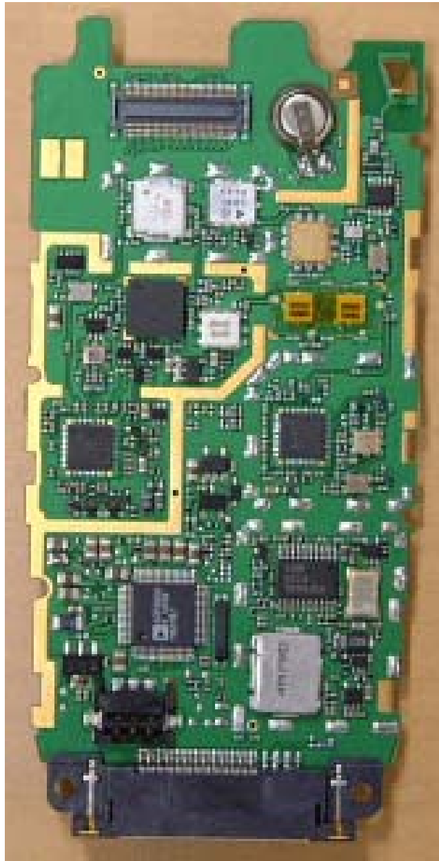
Handheld Portable MAIN Board (Back side , With shield cover removed) VCTCXO : VC-TCXO-208C3-19.2MHz
