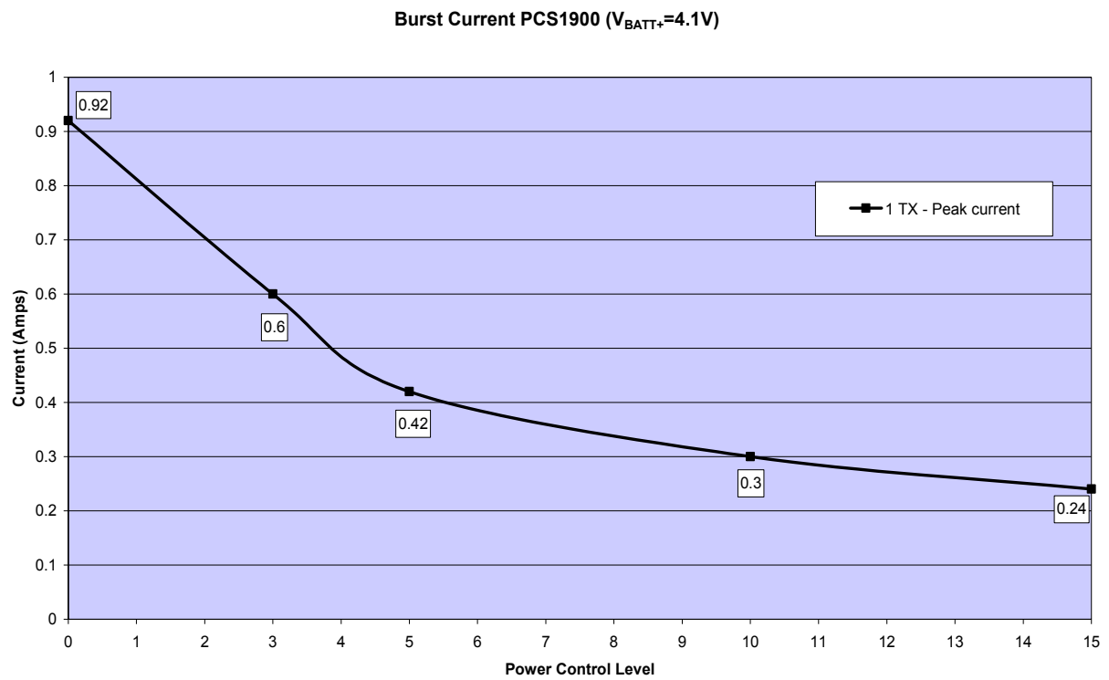
Figure 36: Typical current consumption vs. power control level
