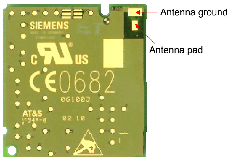
Figure 28: Antenna pad and GND plane
