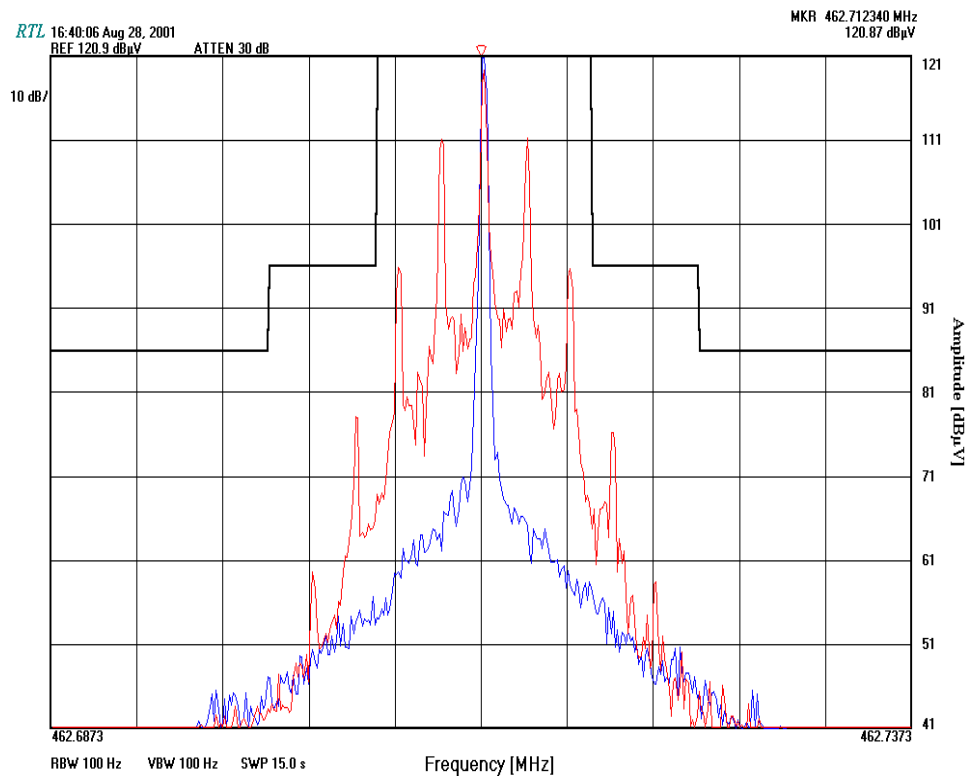
PLOT 8-1: EMISSION BANDWIDTH {FCC PART 95 §95.633}
