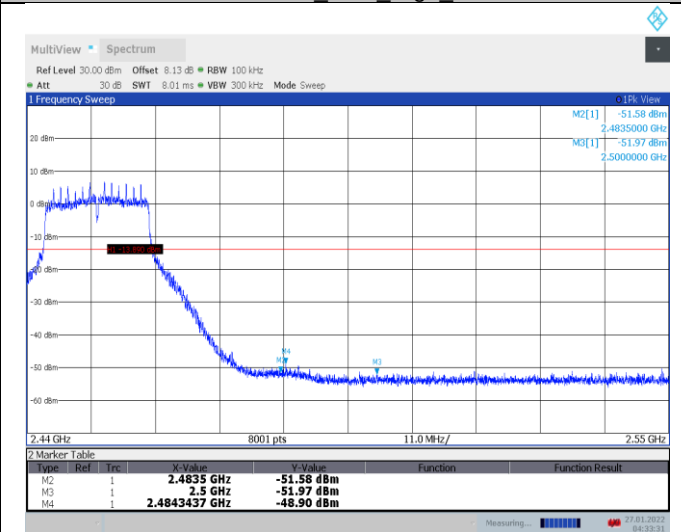
11N20SISO_Ant1_High_2457
