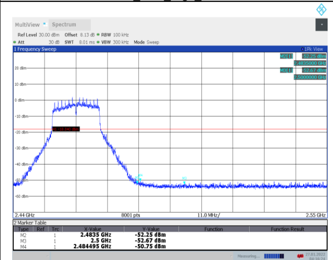
11G_Ant1_High_2462
