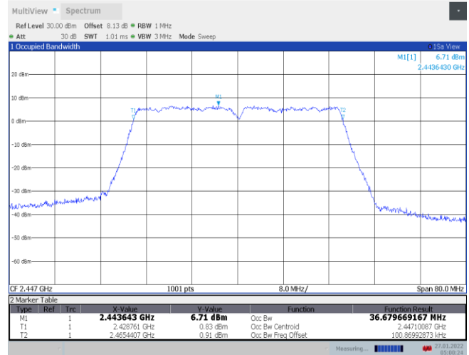
11N40SISO_Ant1_2447
