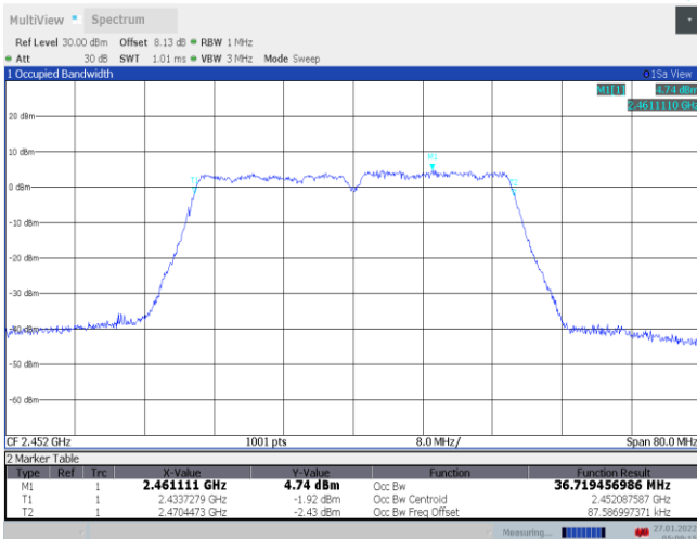
11N40SISO_Ant1_2452
