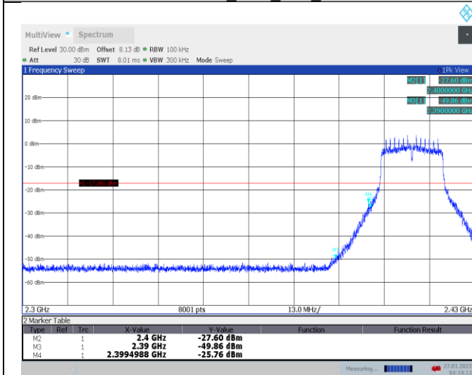
11N20SISO_Ant1_Low_2417
