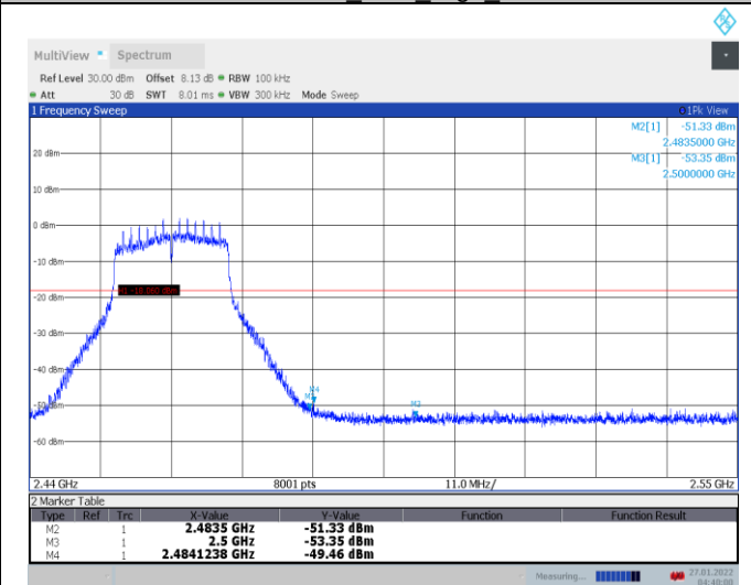
11N20SISO_Ant1_High_2462
