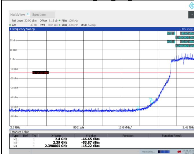
11N20SISO_Ant1_Low_2422
