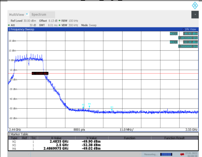
11G_Ant1_High_2457
