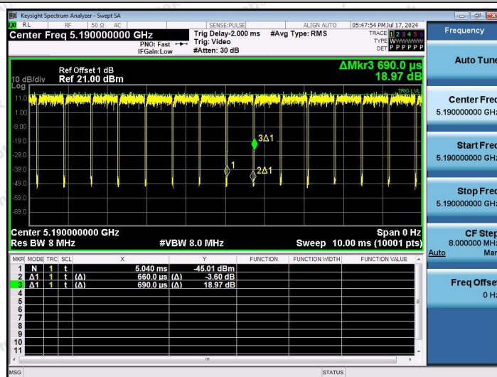
NTNV-11AC40SISO-Ant1-5190
