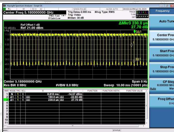
NTNV-11AX20SISO-Ant1-5180
