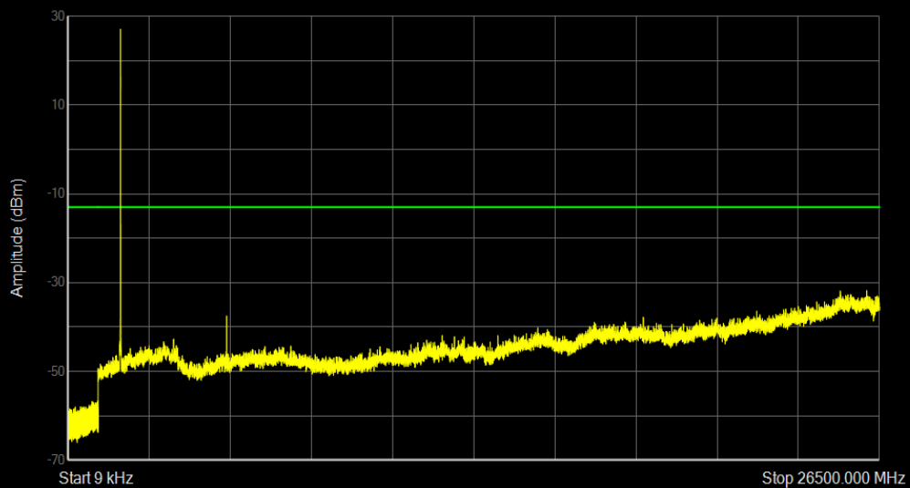
Band4 QAM16 BW=3MHz Channel=20175 RB Size=1 Position=#0
