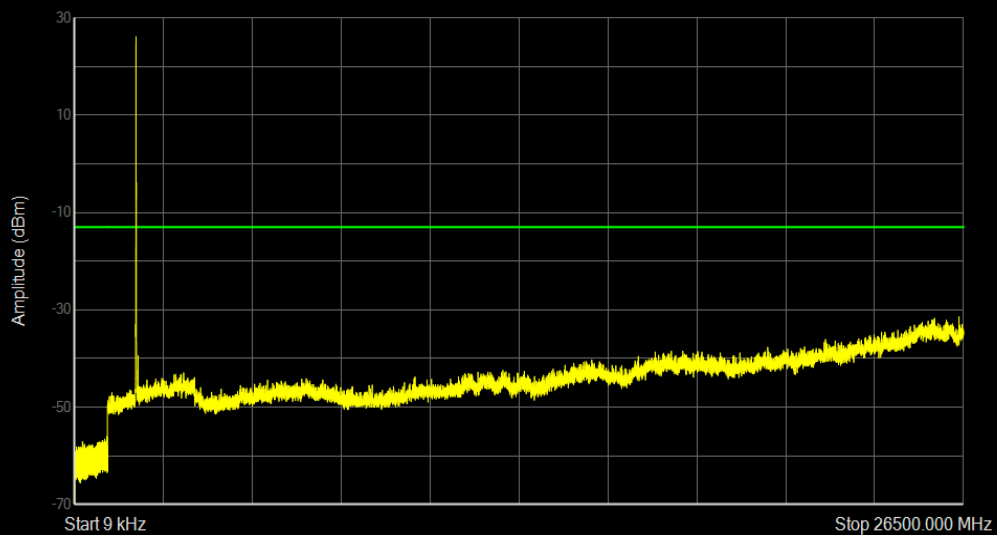
Band2 QAM16 BW=5MHz Channel=18625 RB Size=1 Position=#0
