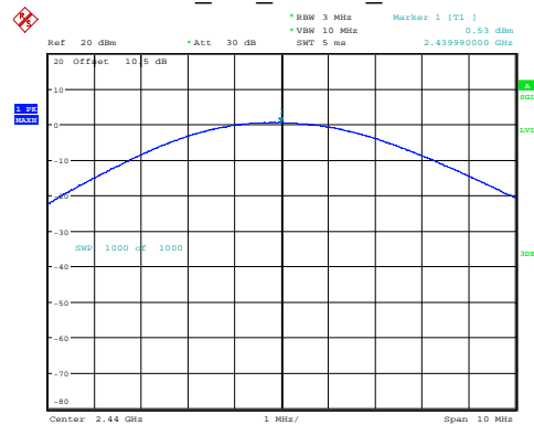
BLE_1M_Middle_Channel
