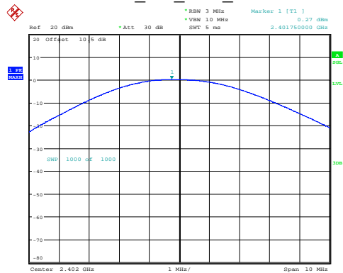
BLE_1M_Low_Channel
