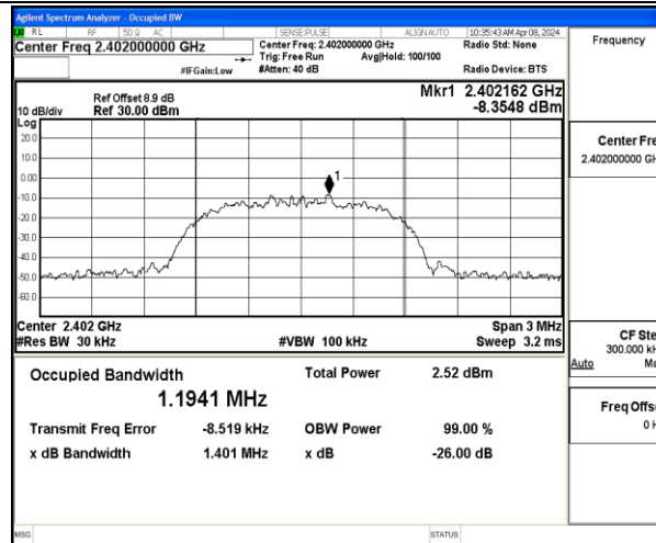
3DH5-Ant1-2402
