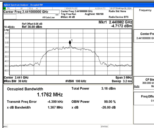
3DH5-Ant1-2441
