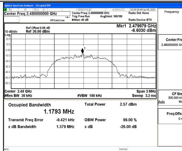
3DH5-Ant1-2480
