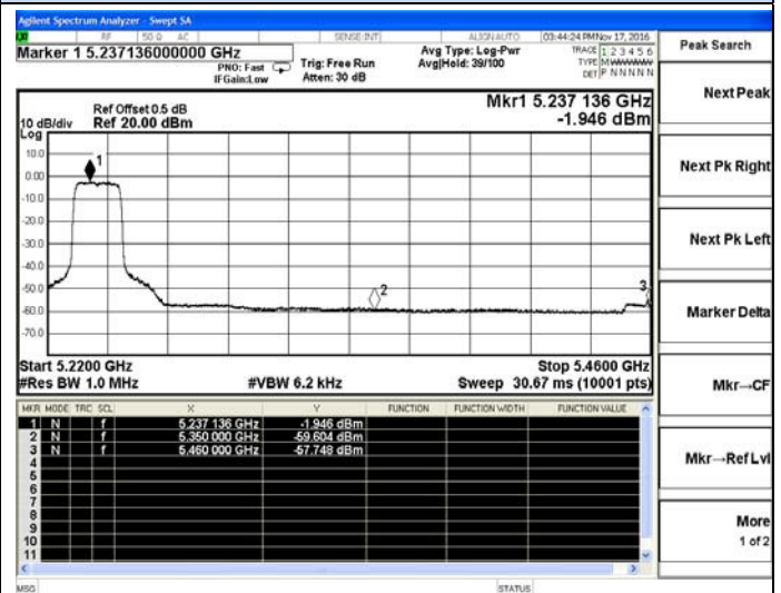
802.11ac20-High channel(Average)
