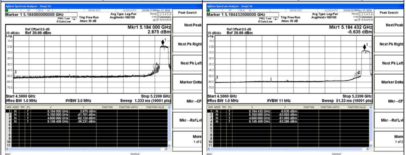
802.11n-HT40-Low channel(Peak)
