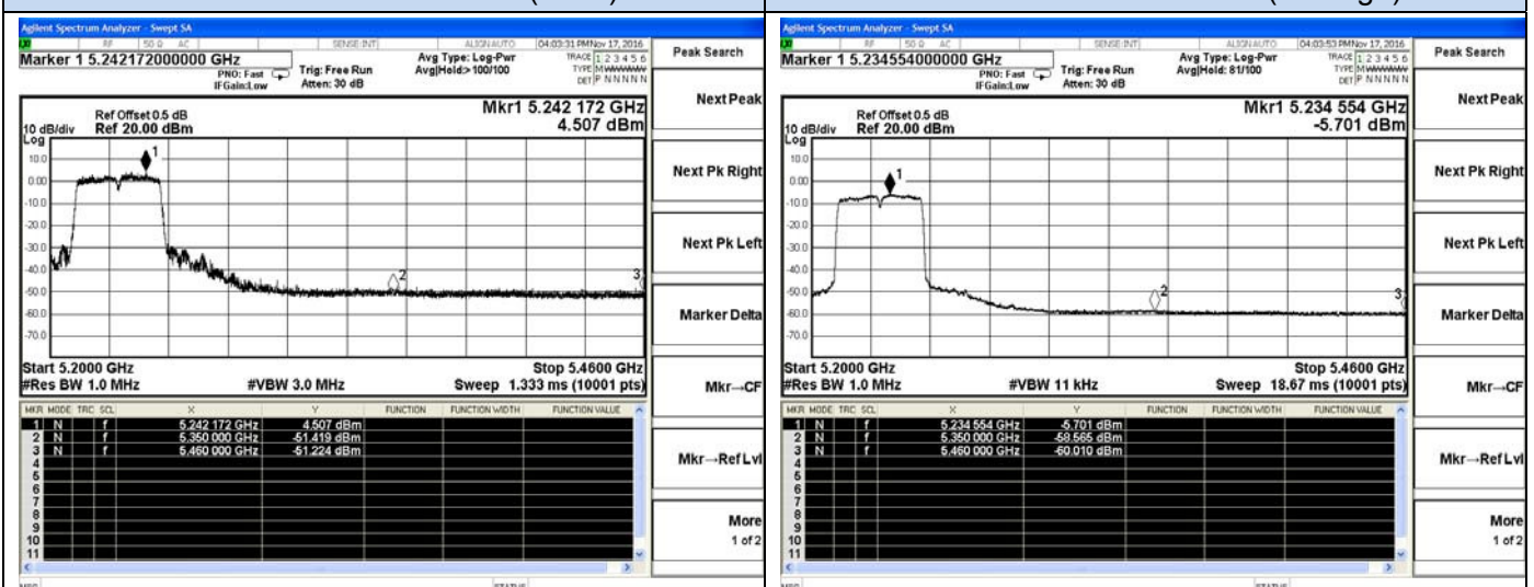
802.11n-HT40-High channel(Peak)
