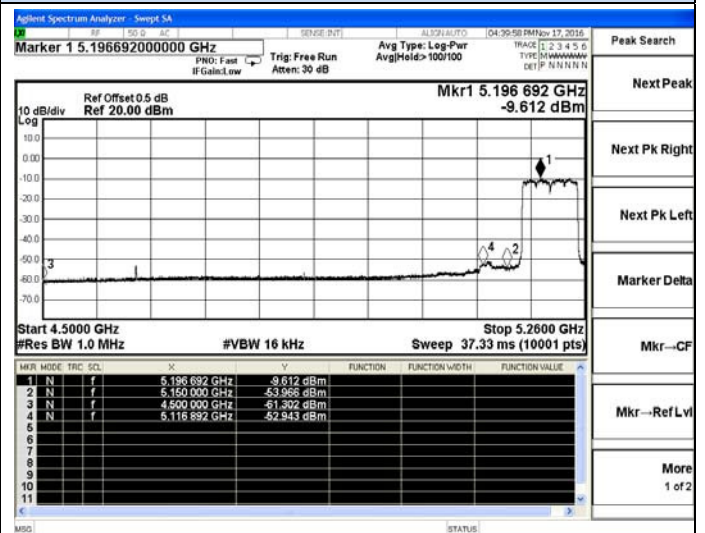
802.11ac80-Low channel(Average)
