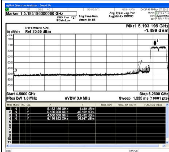
802.11ac80-Low channel(Peak)
