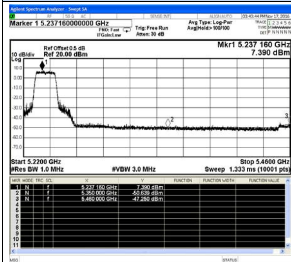
802.11ac20-High channel(Peak)
