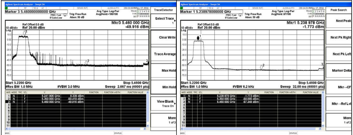
802.11a-High channel(Peak)
