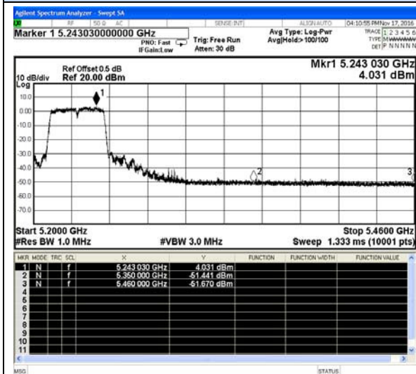
802.11ac40-High channel(Peak)
