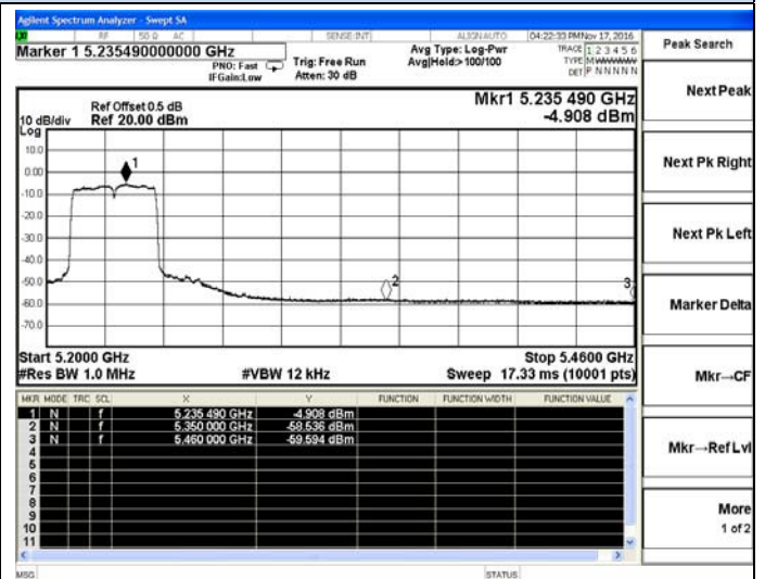
802.11ac40-High channel(Average)
