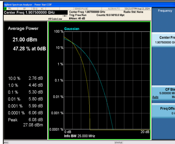
Band2-5MHz-16QAM-19175-25RB#0-PASS
