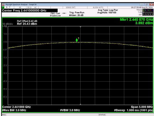
Peak Output Power n/4QPSK_Channel 39
