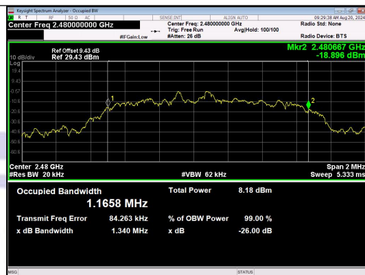
n/4QPSK_2-DH1_Channel 78
