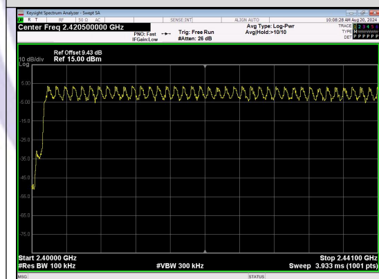
Low End Spectrum Channel Hopping Plot n/4DQPSK
