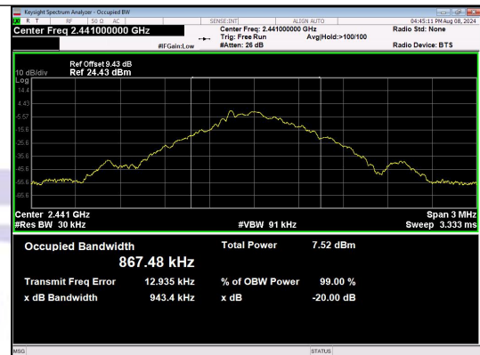
GFSK_DH1_Channel 39
