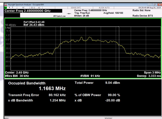
n/4DQPSK_2-DH1_Channel 78
