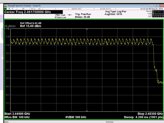
High End Spectrum Channel Hopping Plot n/4DQPSK
