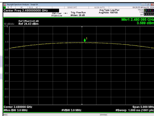
Peak Output Power n/4QPSK_Channel 78
