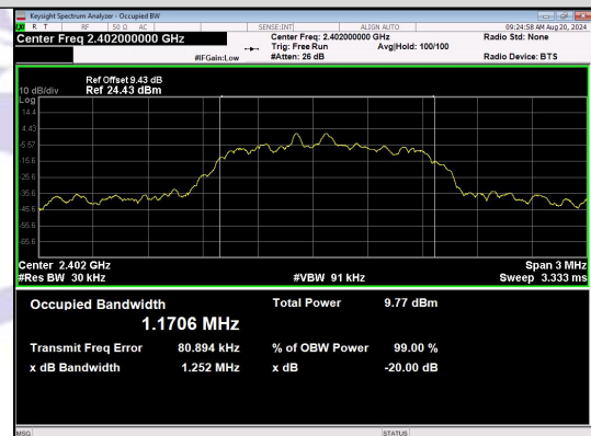
n/4DQPSK_2-DH1_Channel 0
