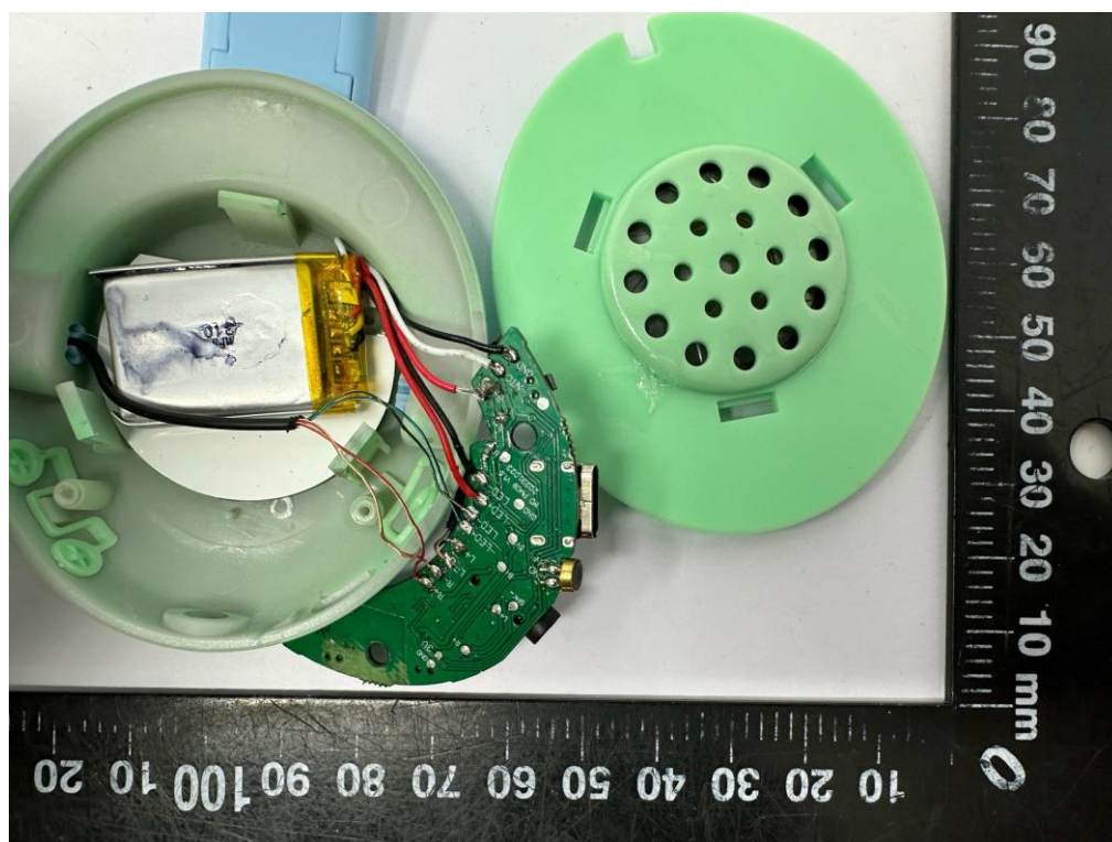
Fig.5. Internal view-02
