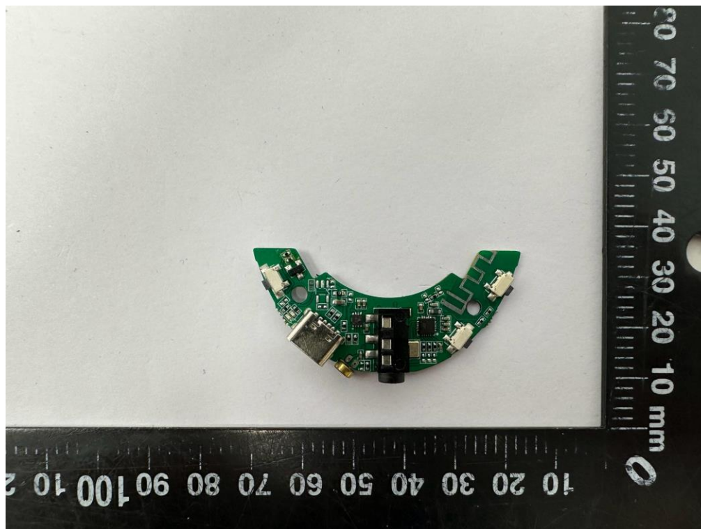
Fig.6. PCB view-01
